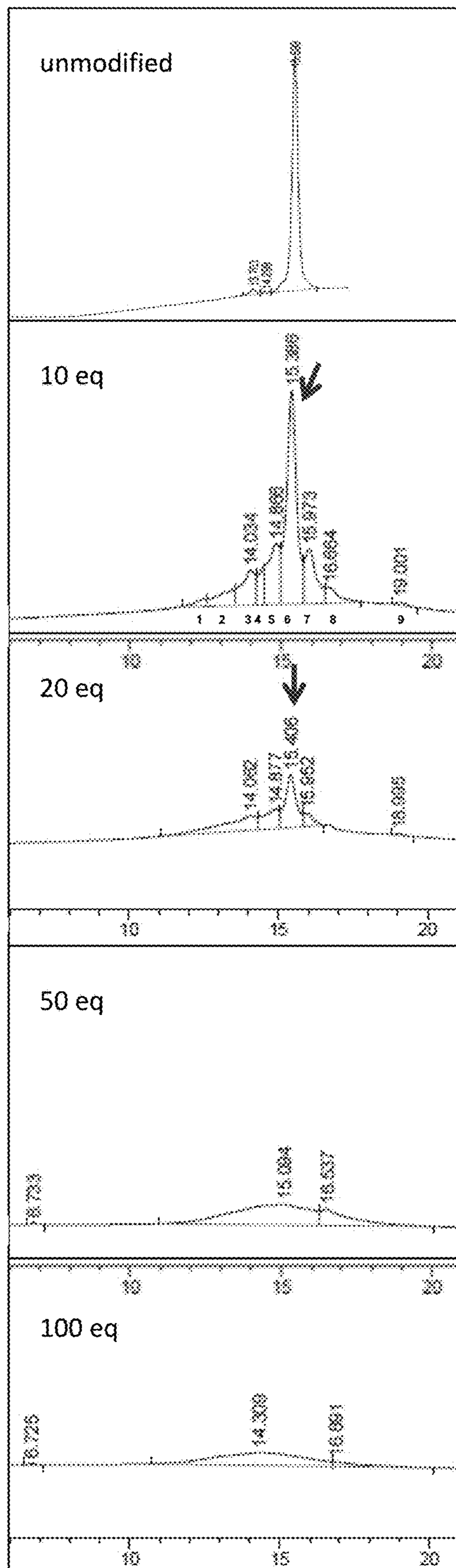
Figure 17: HPLC analysis of peroxynitrite oxidation products
