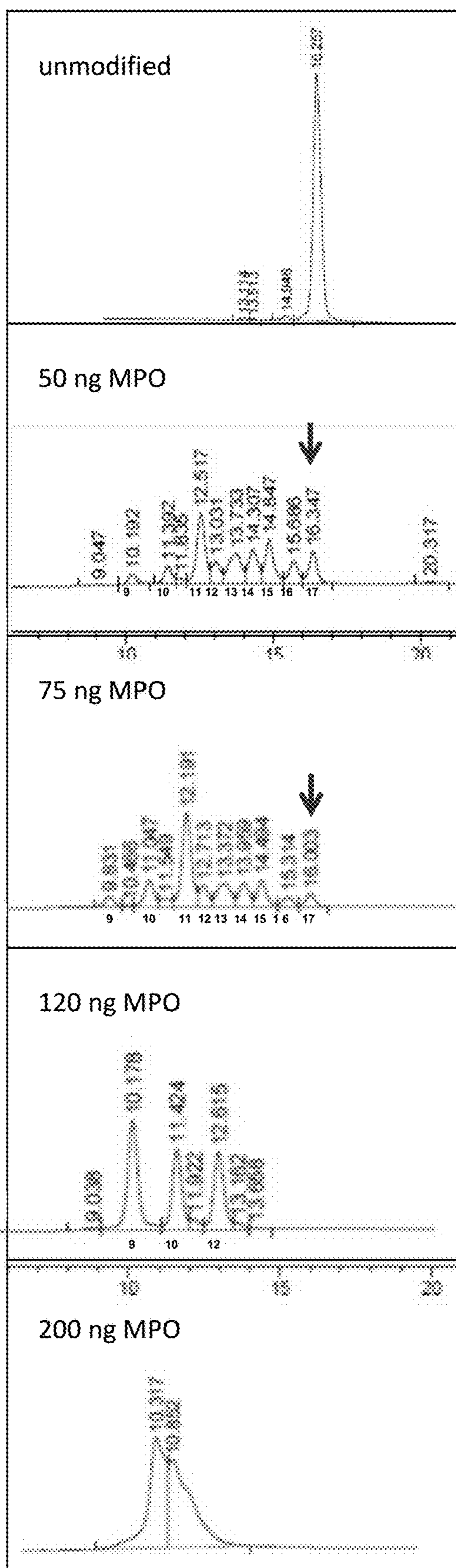
Figure 13: HPLC analysis of MPO-H 2 O 2 oxidation products
