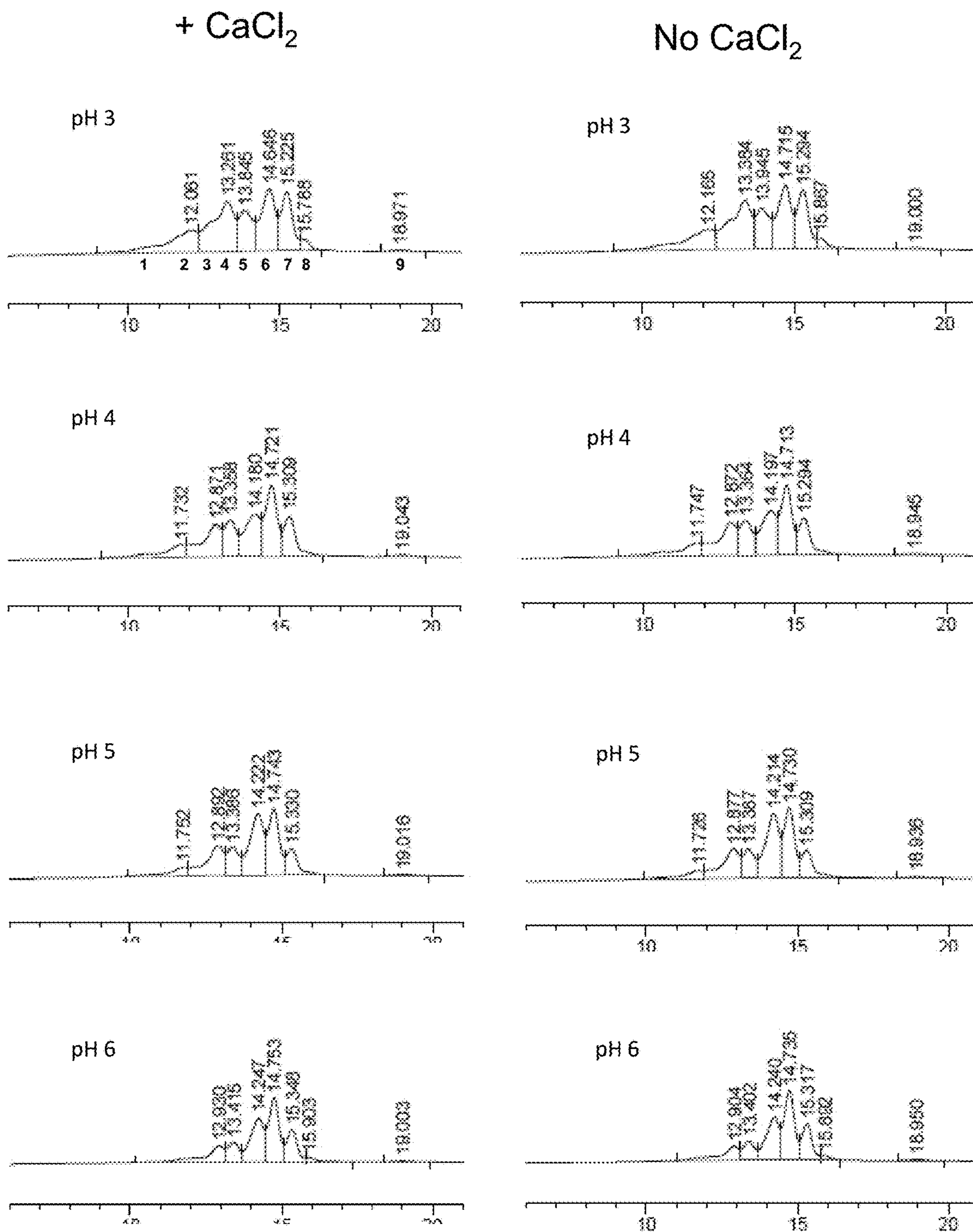
Figure 18: Effects of pH and CaCl 2 on peroxynitrite-mediated oxidation of rhCC10
