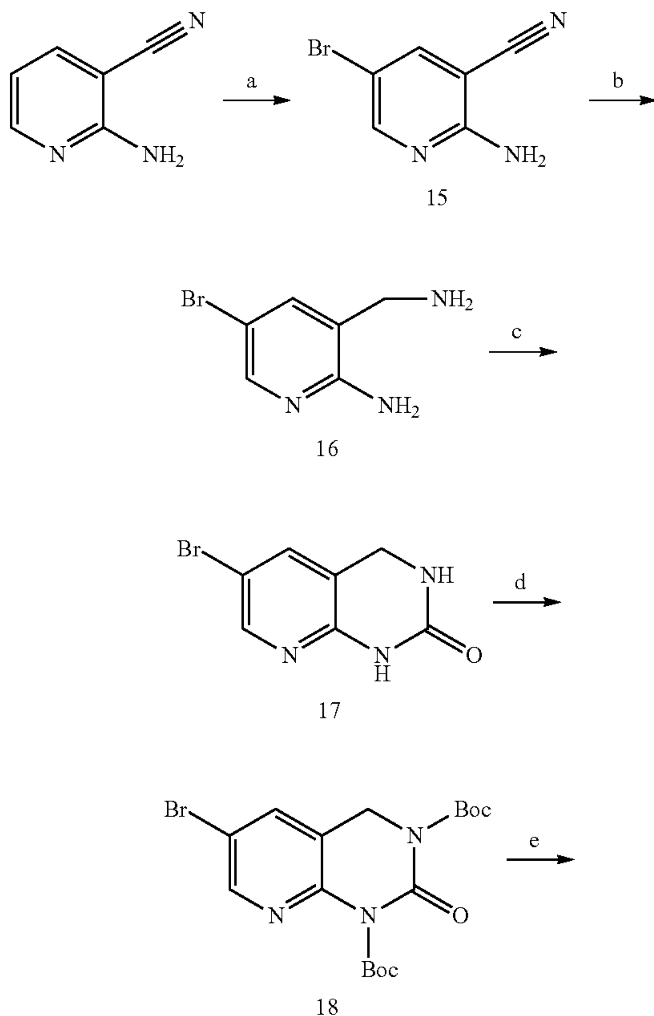
Scheme 1. Synthesis of pyridinol-fused ring analog 12.
