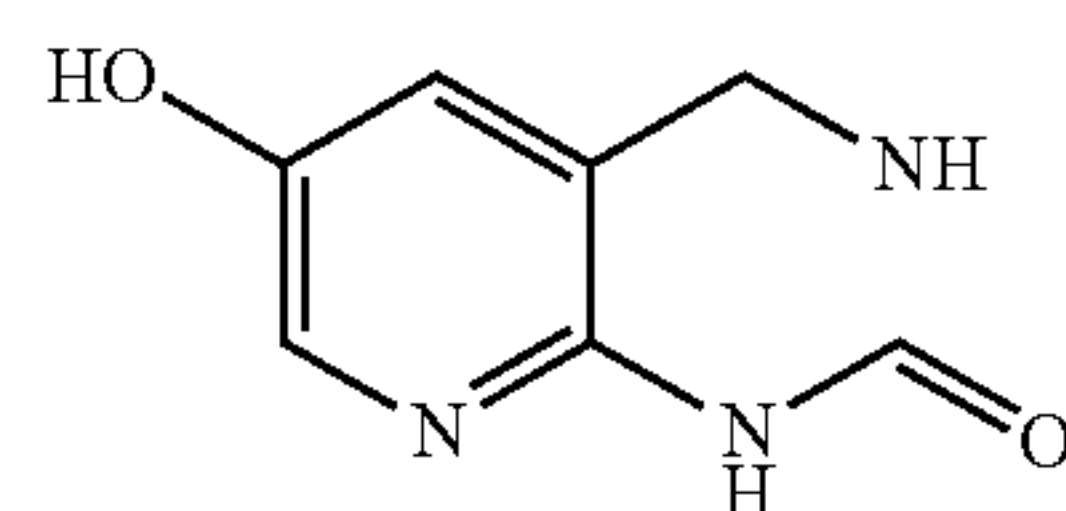
Uric Acid
