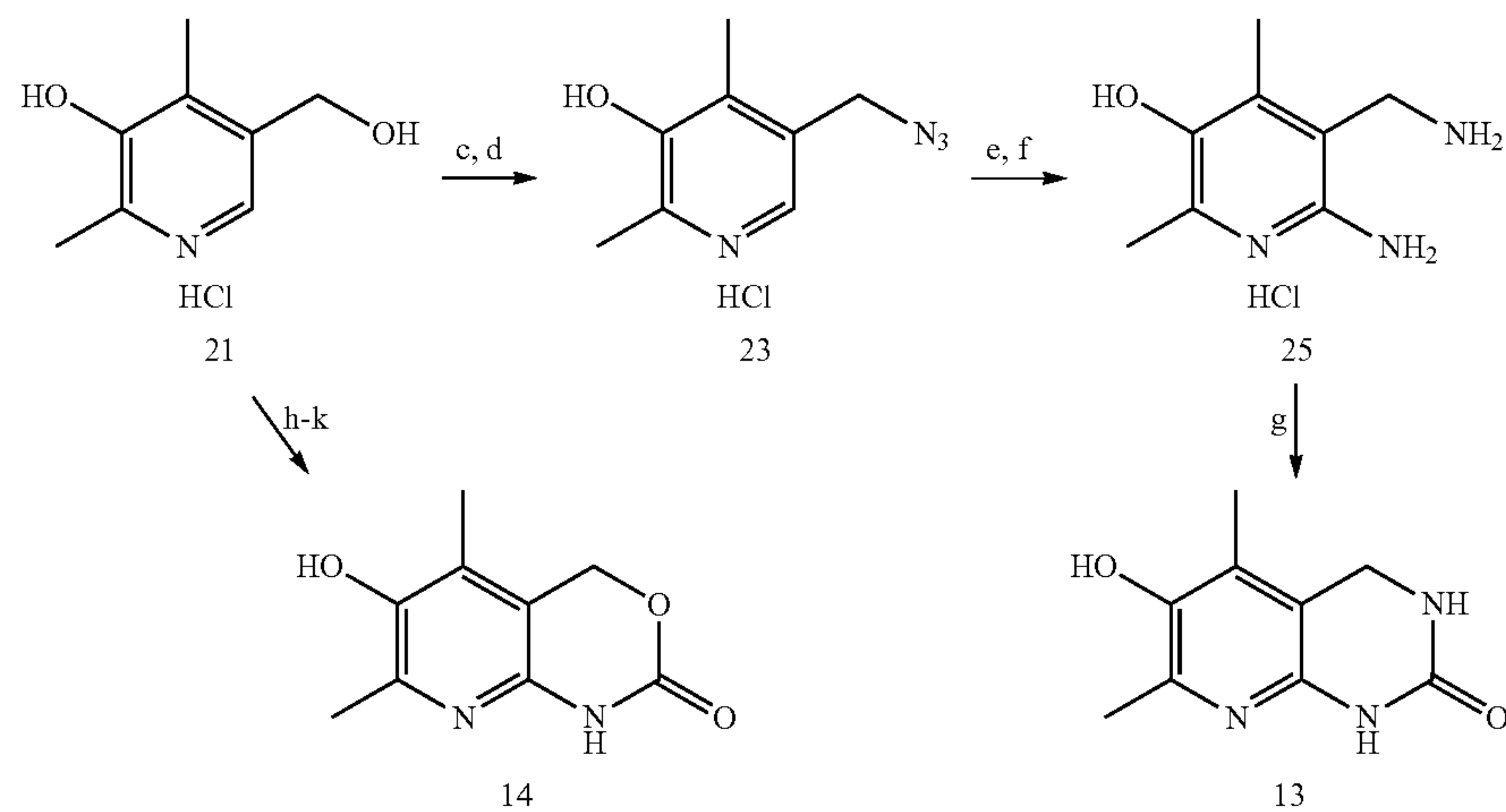
Scheme 2. Synthesis of pyridinol-fused ring analog 13.
