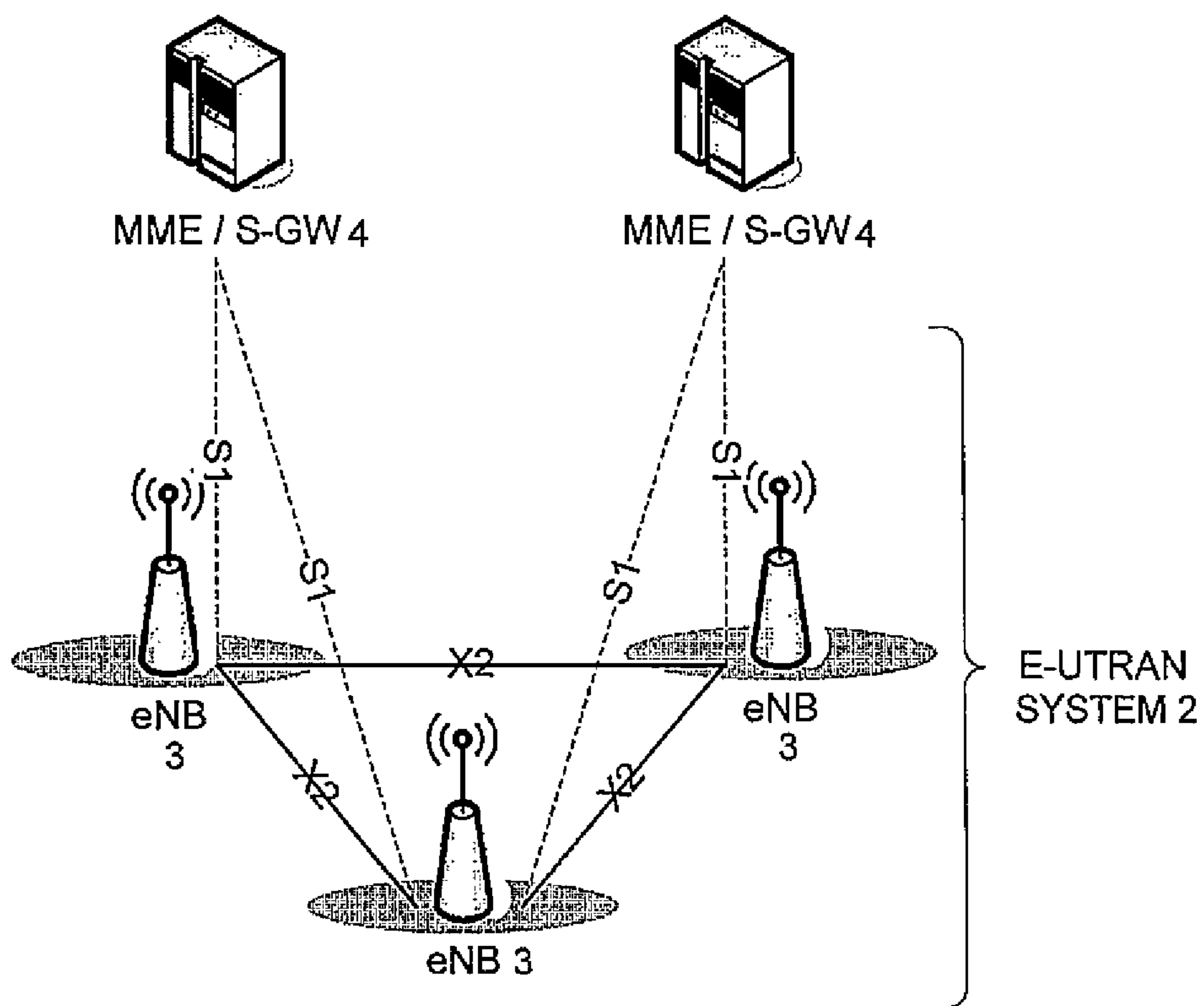
FIG. 1: PRIOR ART
