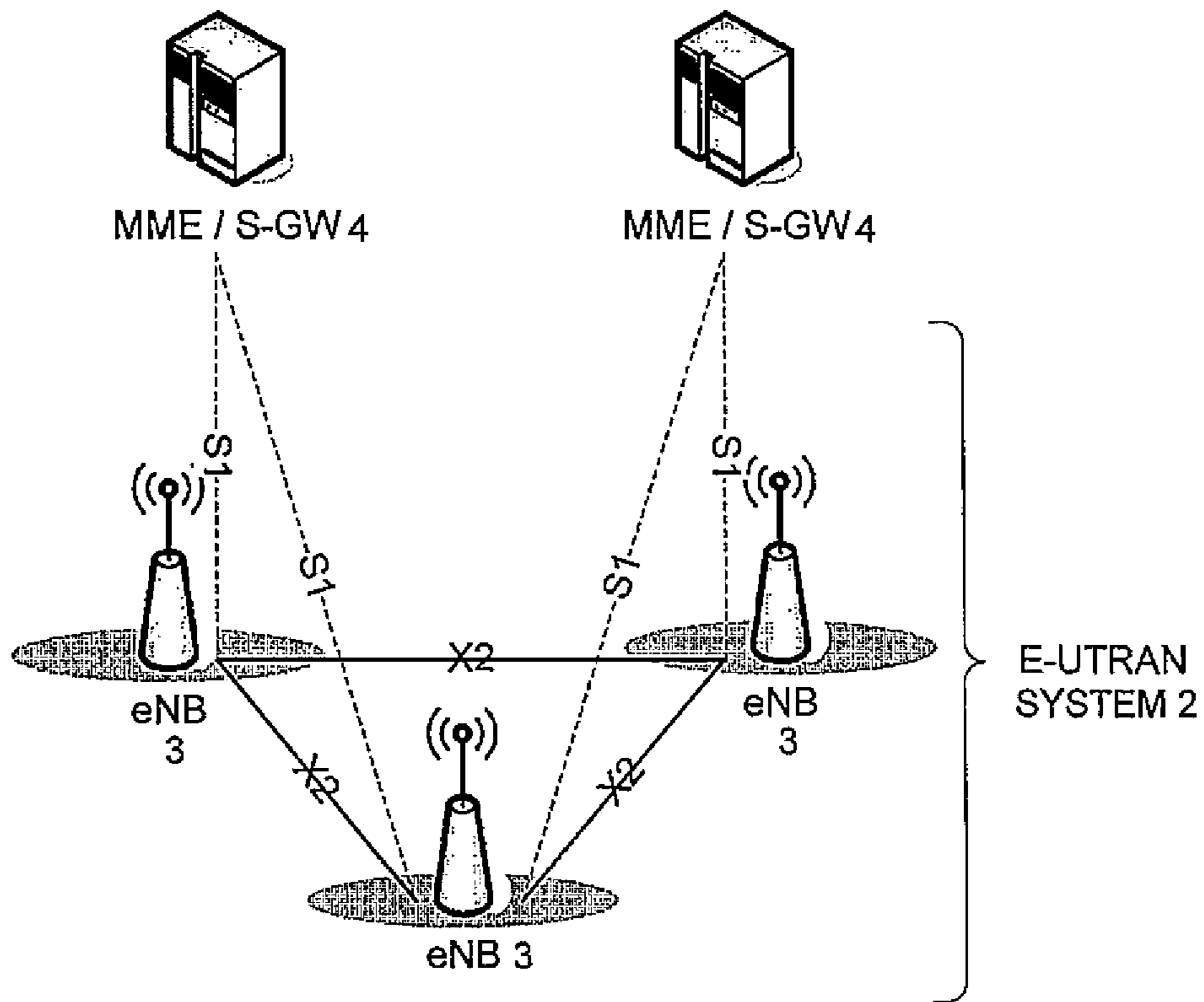
FIG. 1: PRIOR ART
