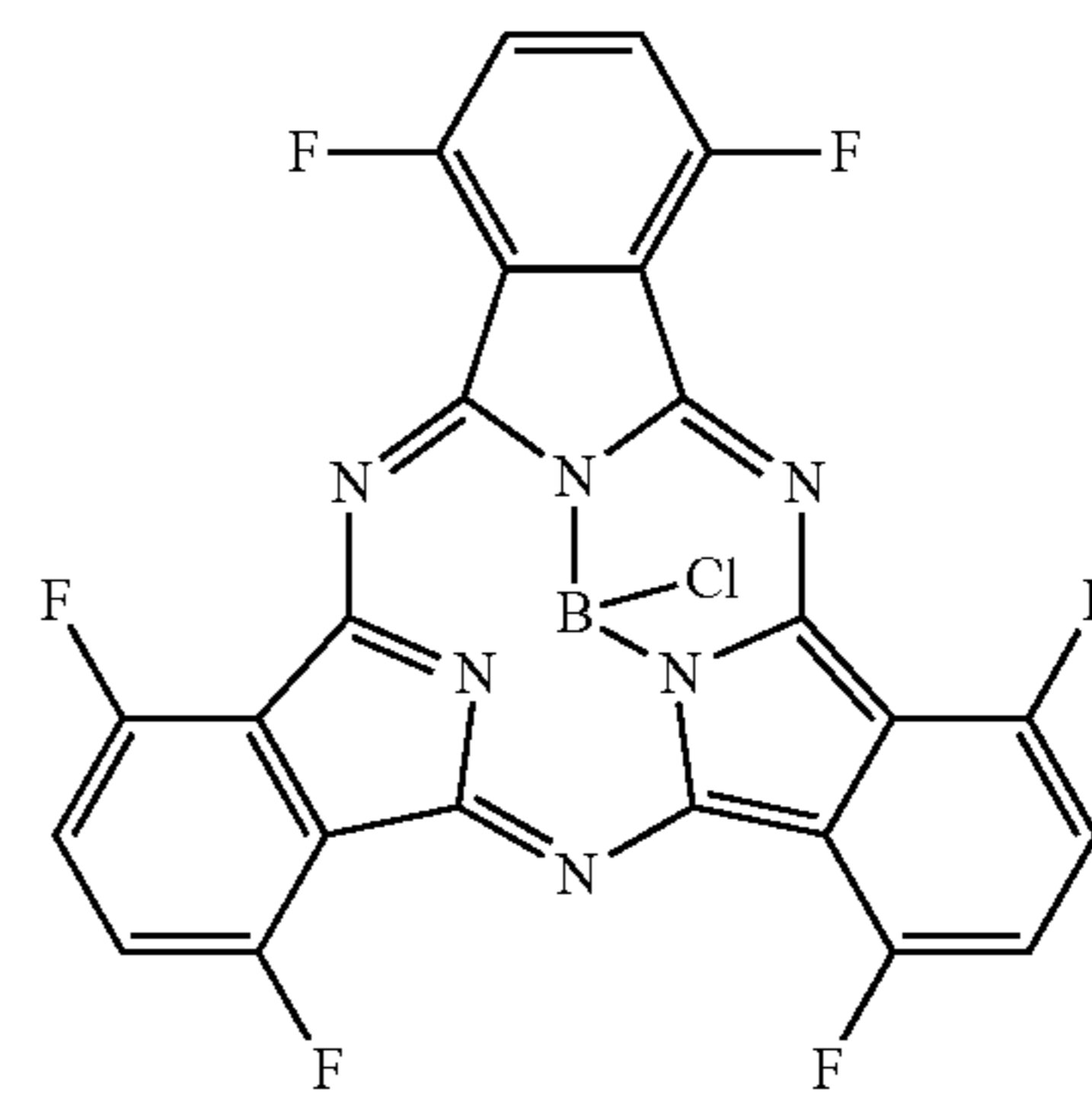
Bay-F6-SubPc-Cl
