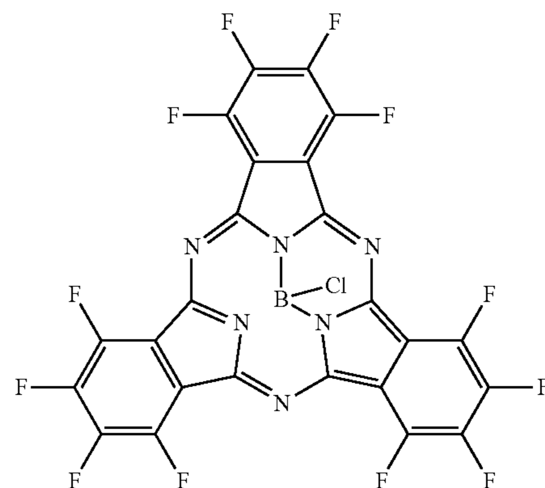
F12-SubPc-Cl
