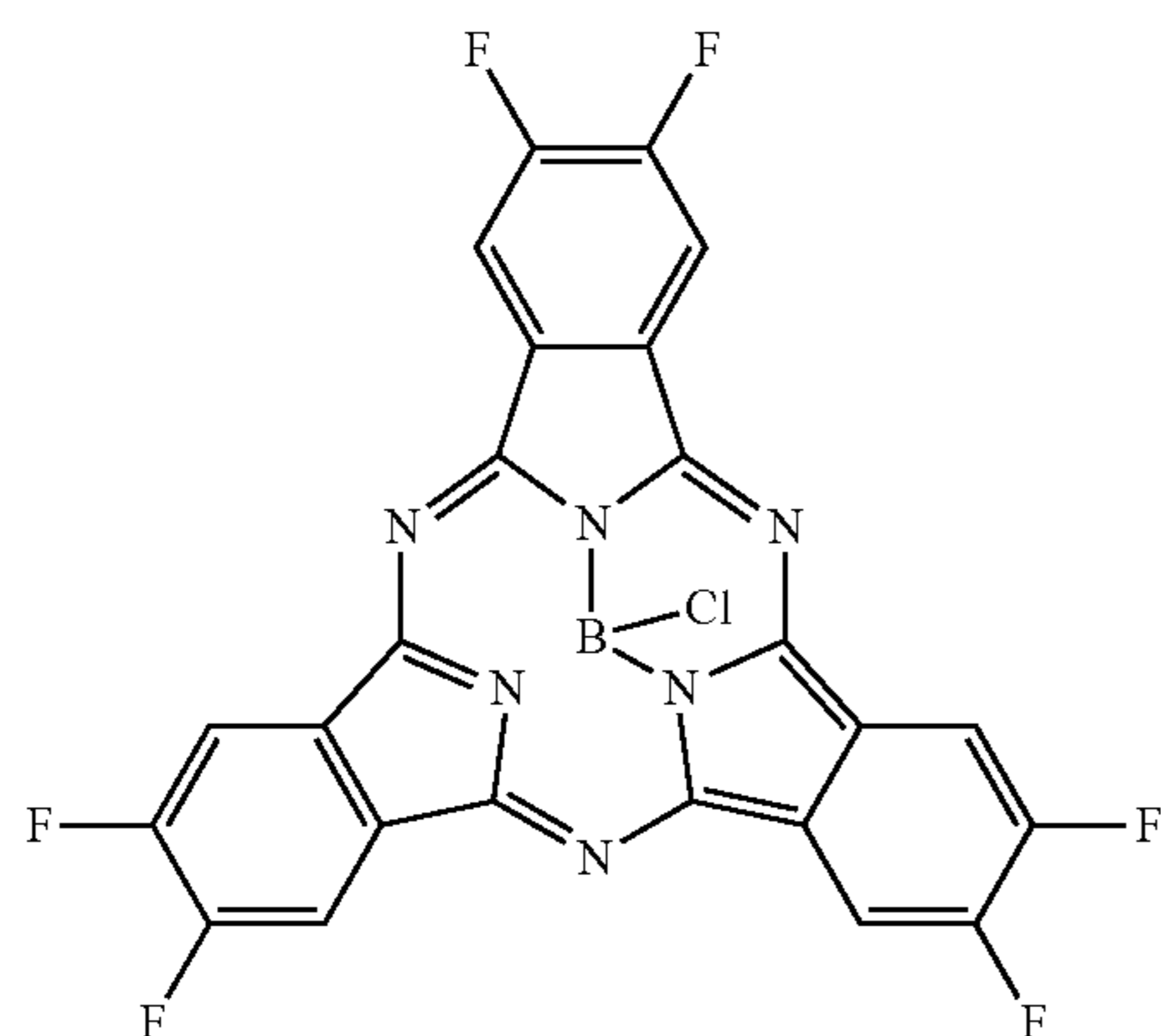
F6-SubPc-Cl
