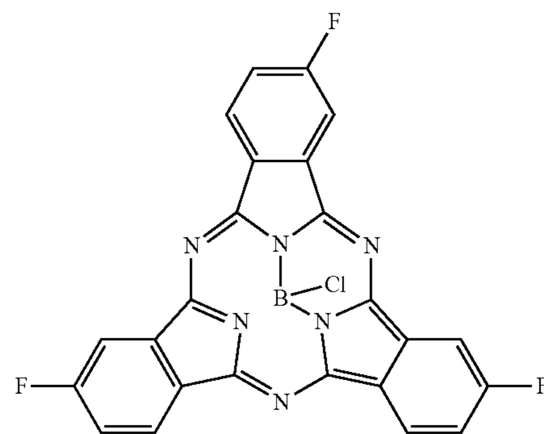
F3(C1)-SubPc-Cl
