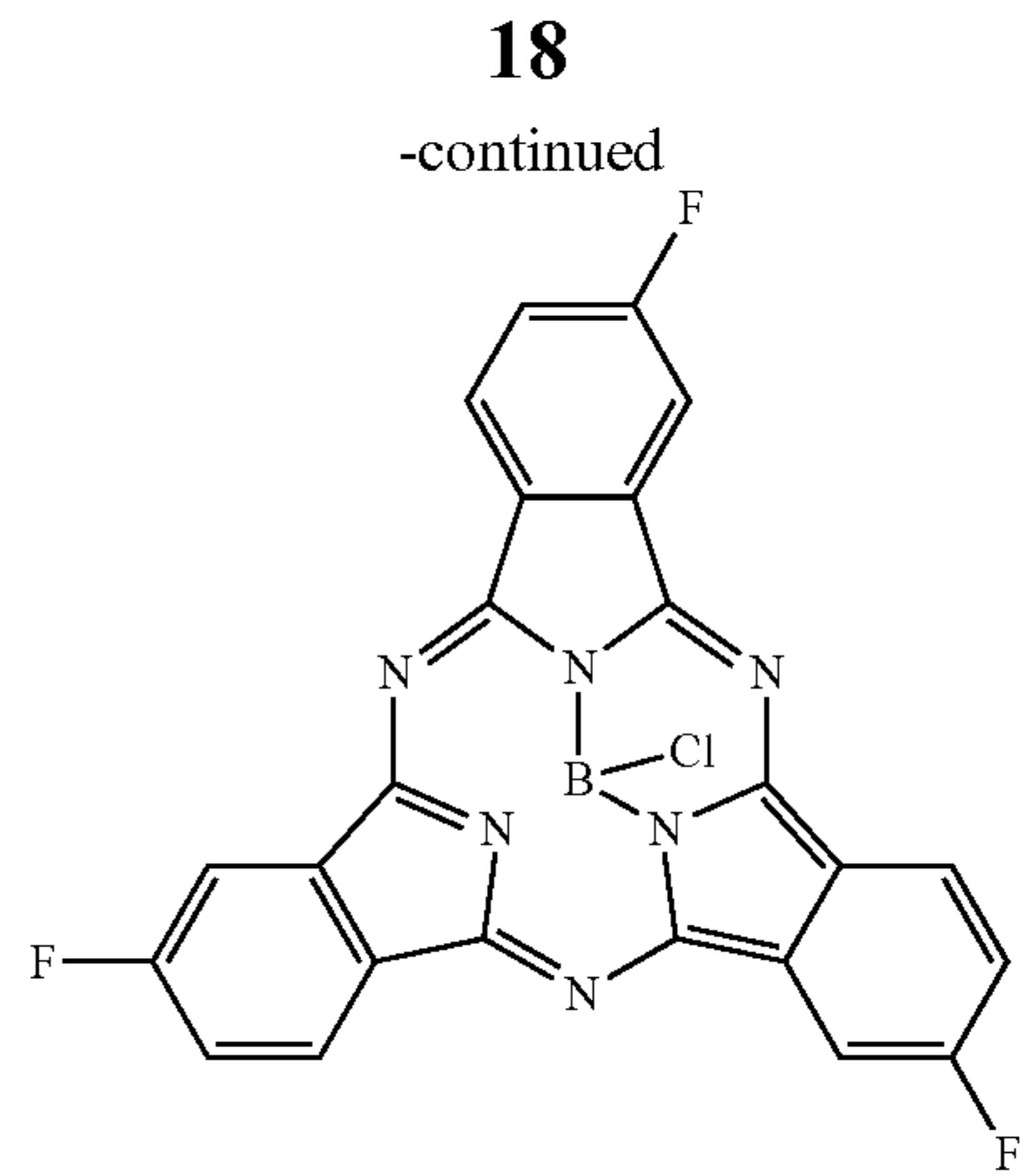
F3(C3)-SubPc-Cl
