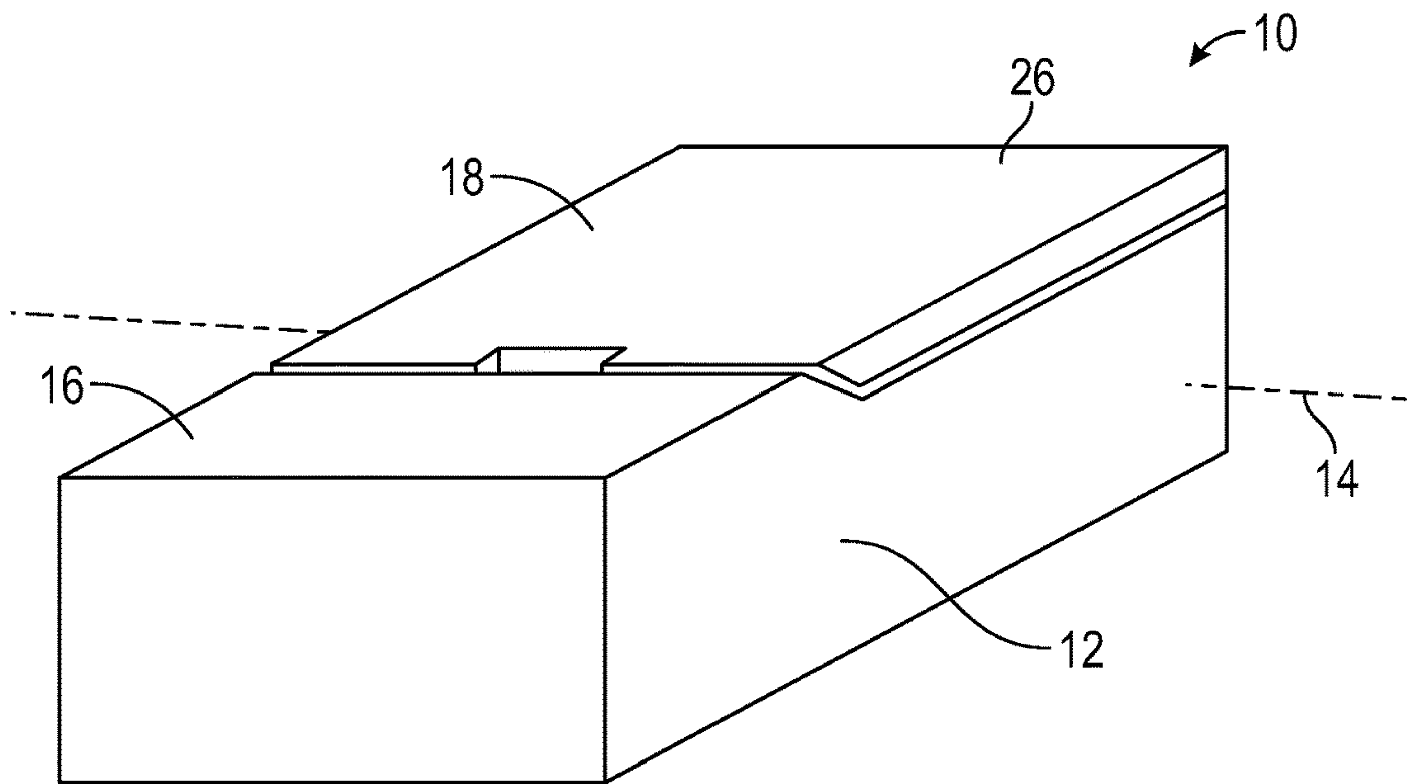
FIG. 1 (Prior Art)
