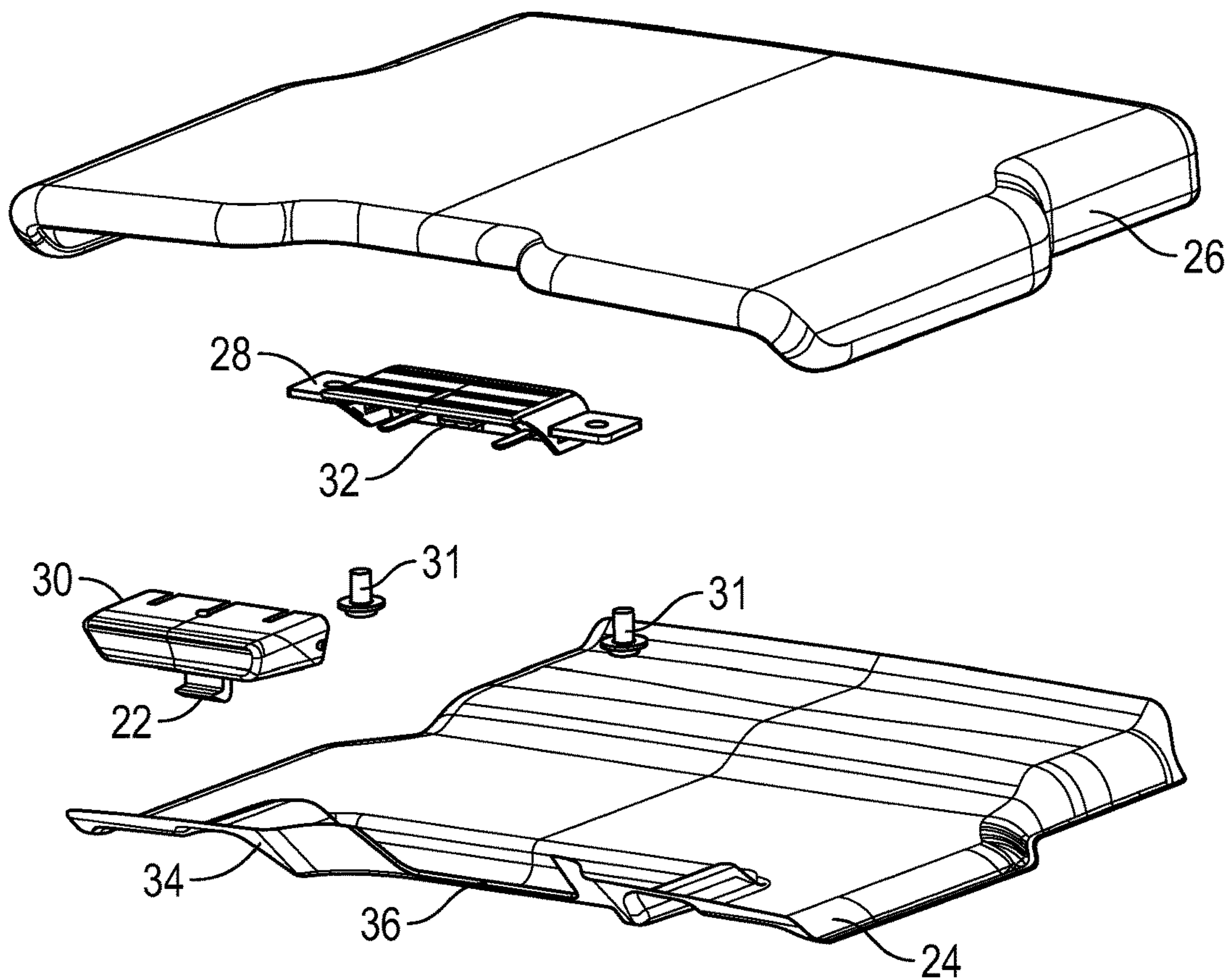
FIG. 3 (Prior Art)
