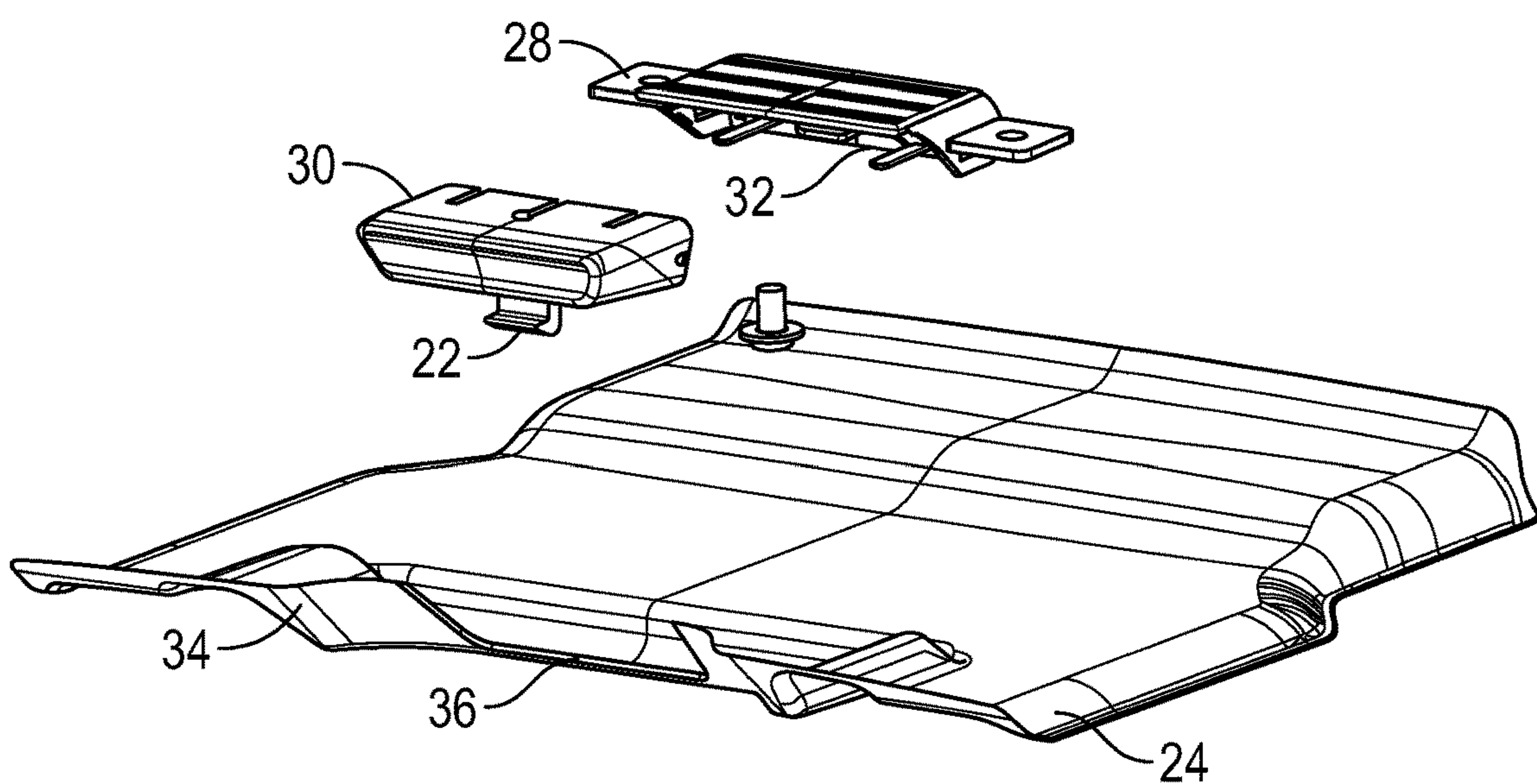
FIG. 4 (Prior Art)
