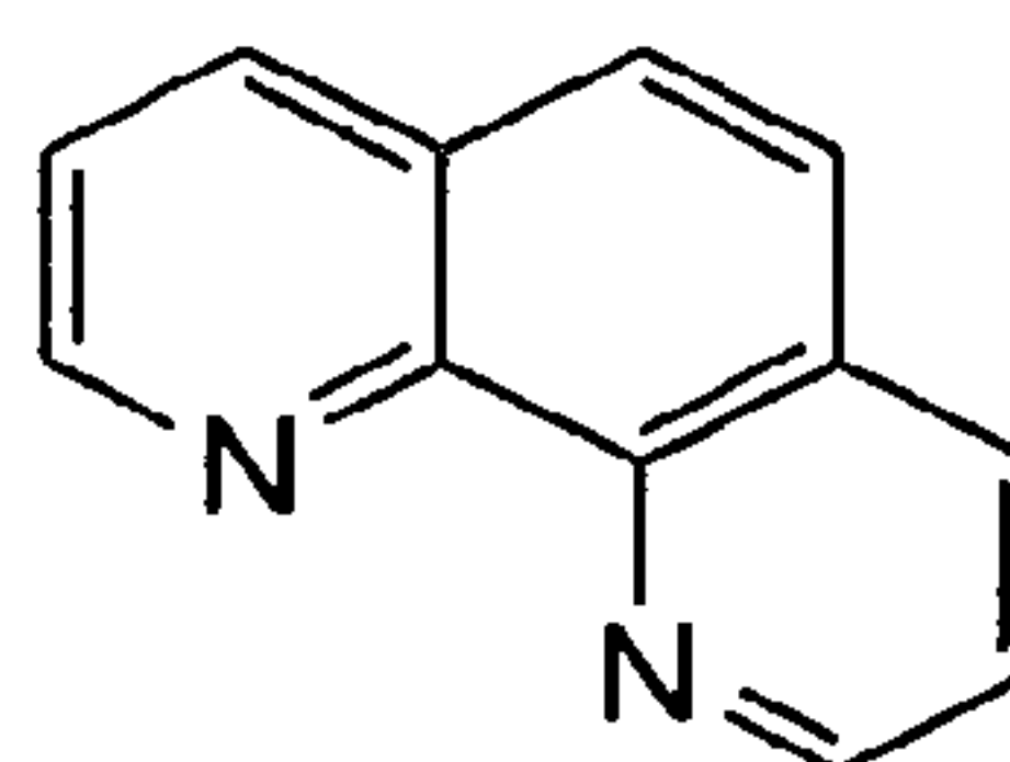
1,10-o-phenanthroline (4,5-diazaphenanthrene)
