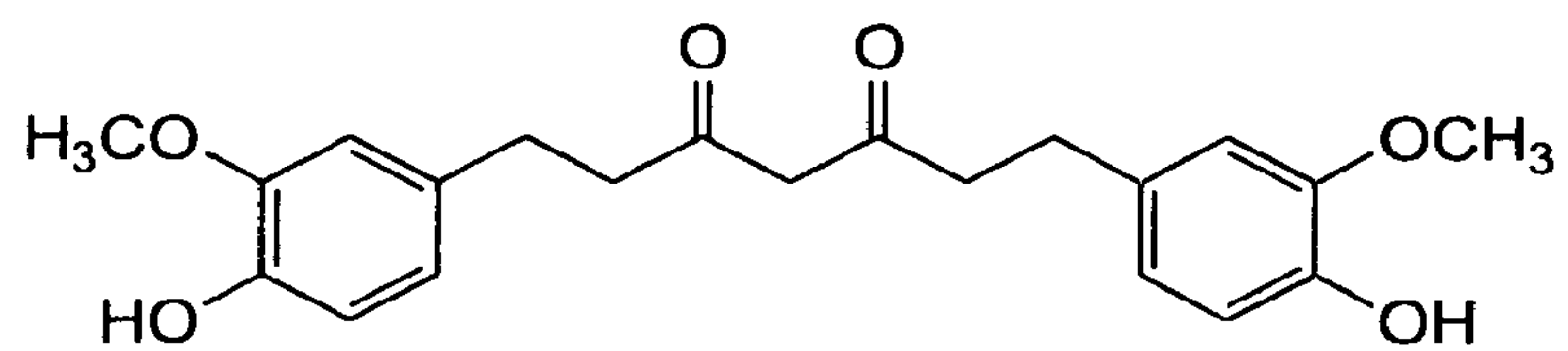
Tetrahydrocurcumin
