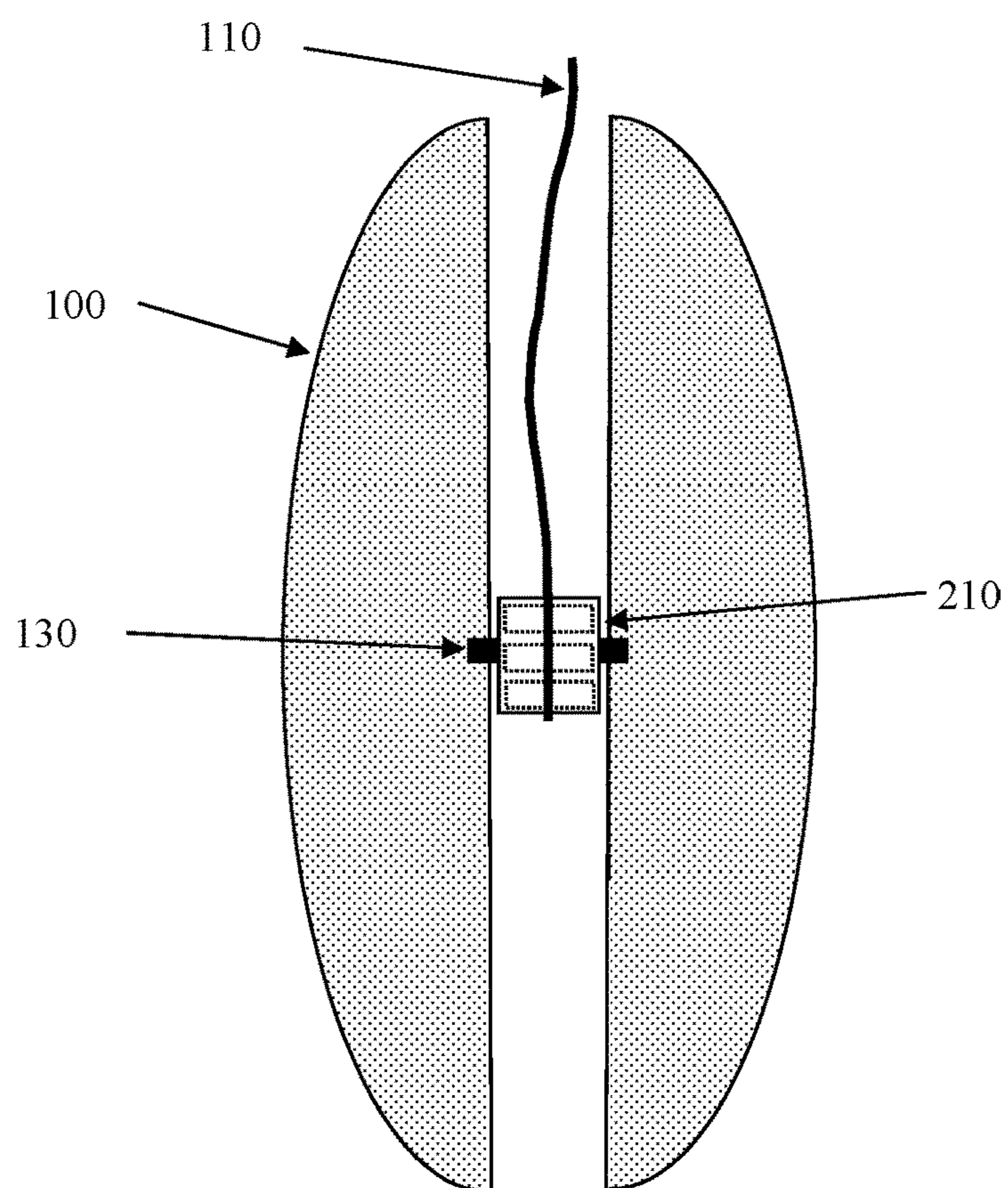
Figure 2 – A Schematic Side-View Diagram of a Ball Bearing Yo-Yo
