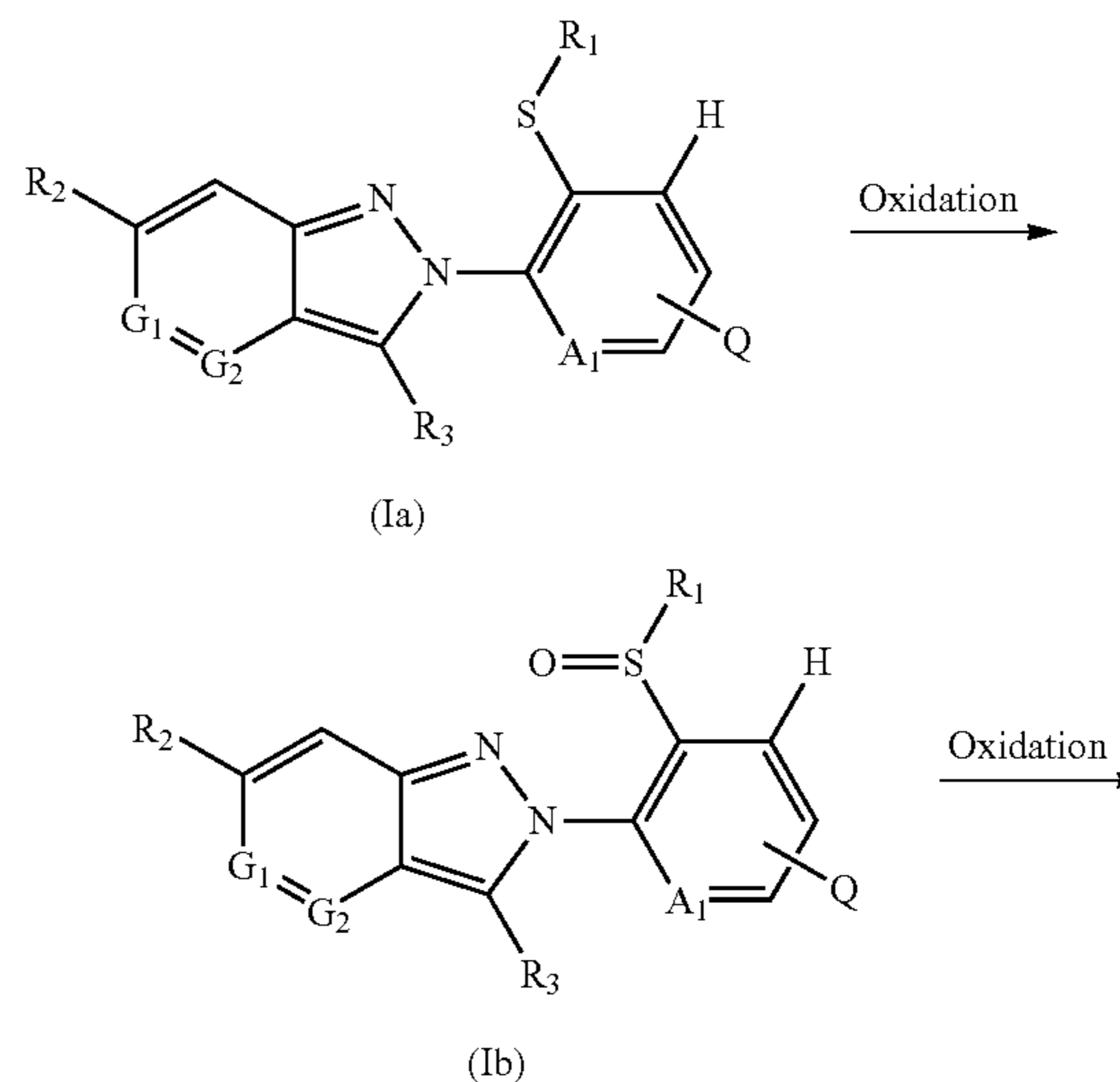
Scheme 7
