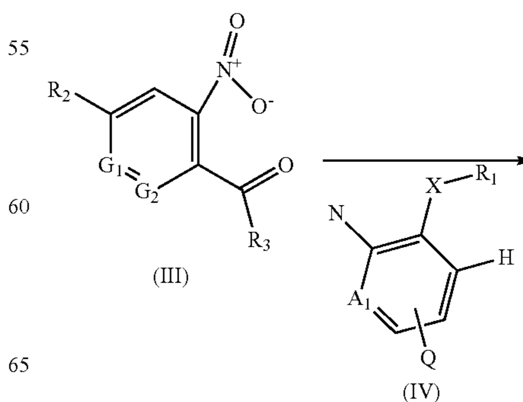
Scheme 2
