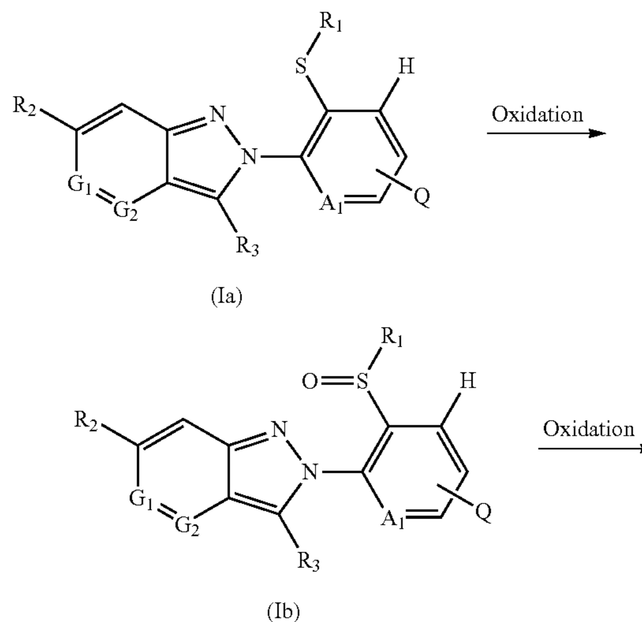
Scheme 7
