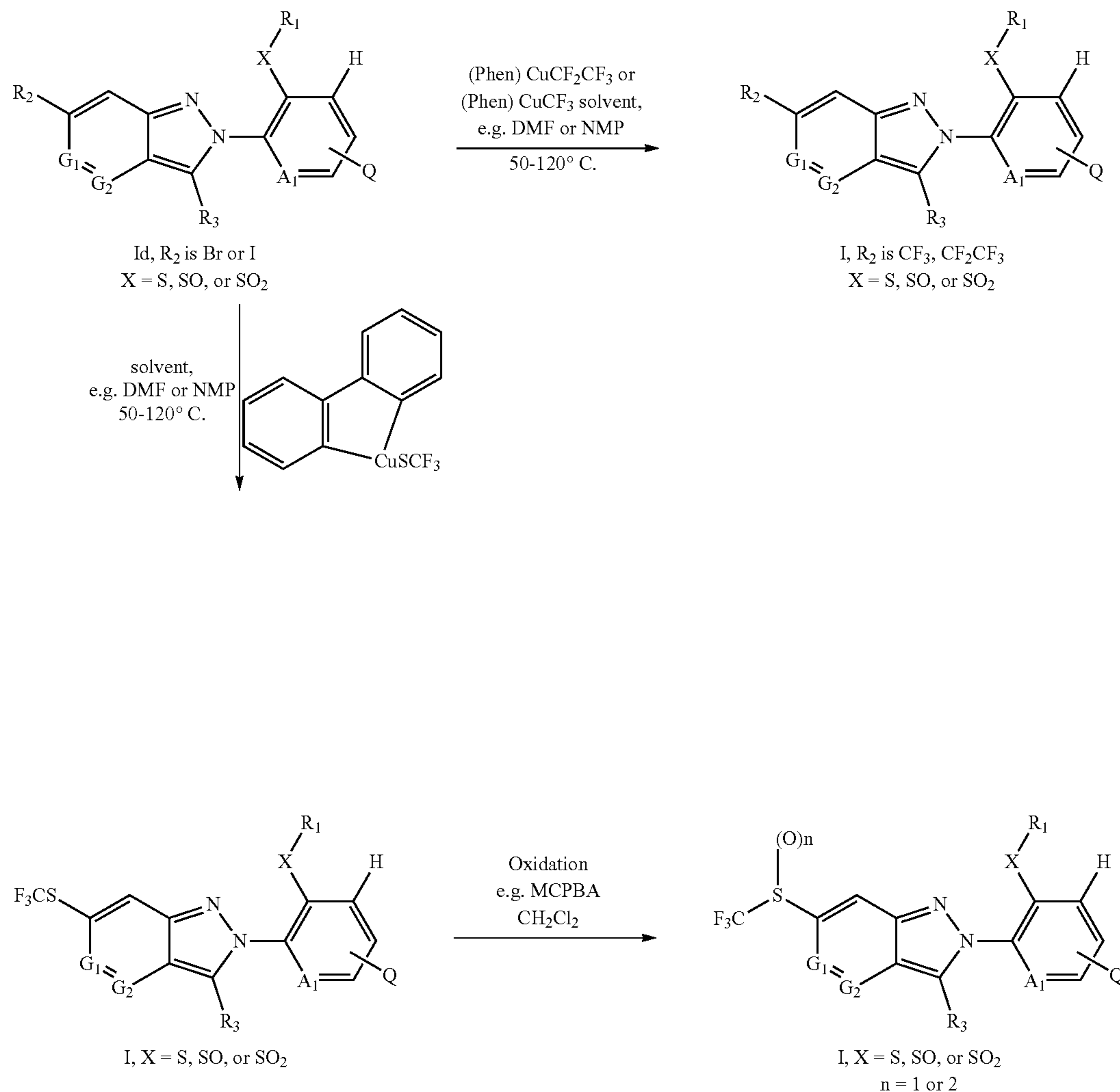
Scheme 6
