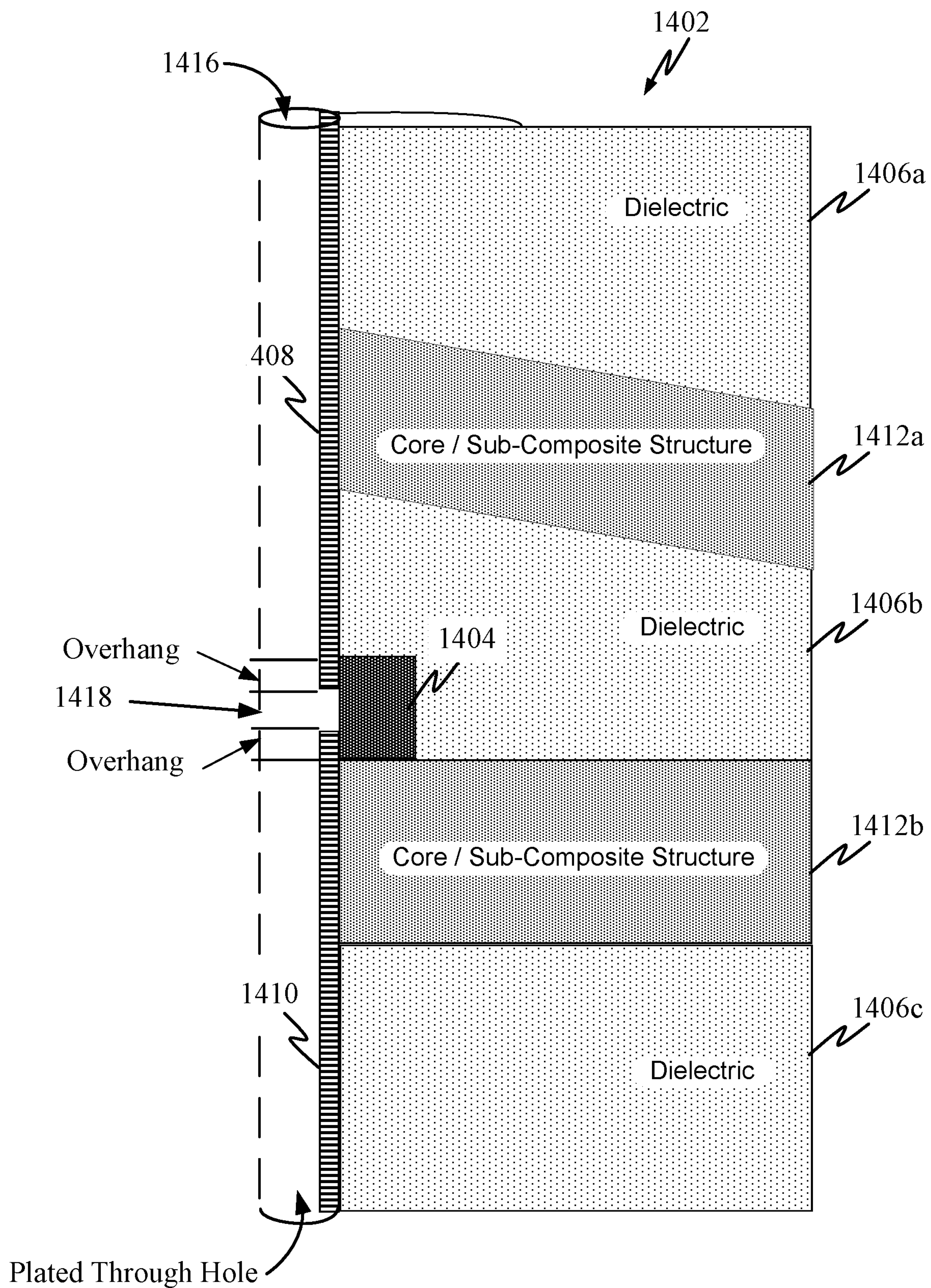
FIG. 14 (Practical Structure)
