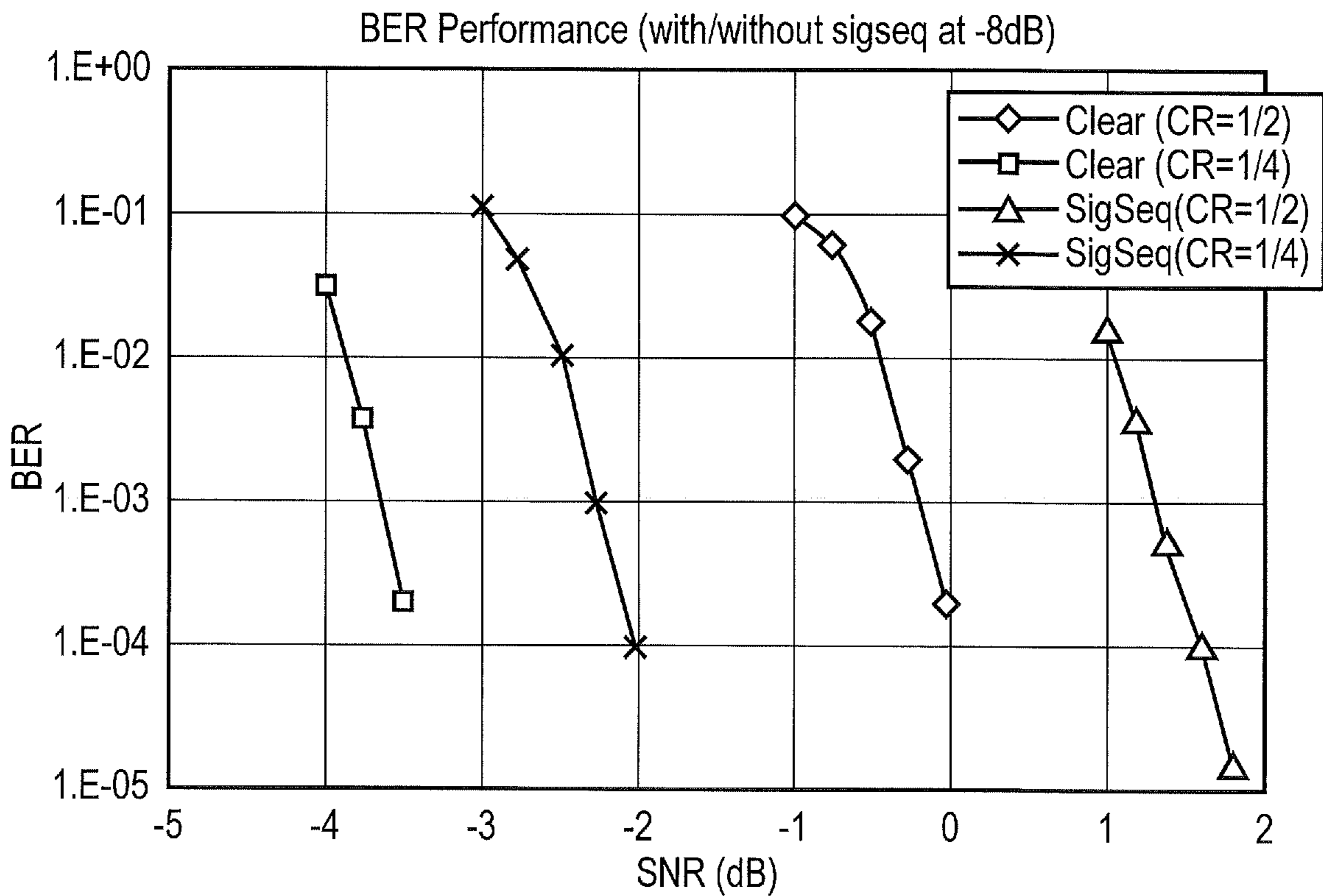
AWGN performance of composite preamble symbol
