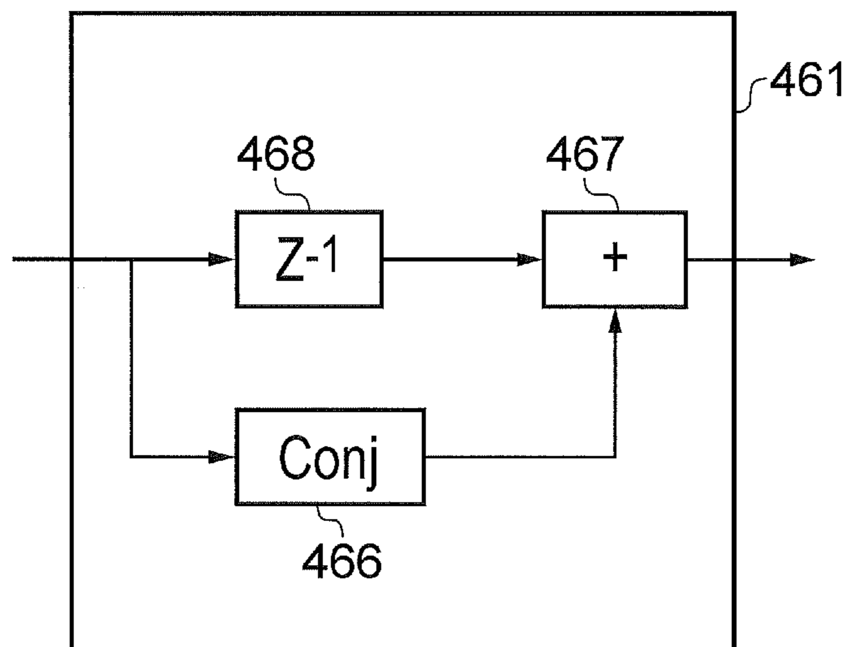
Differential Encoder
