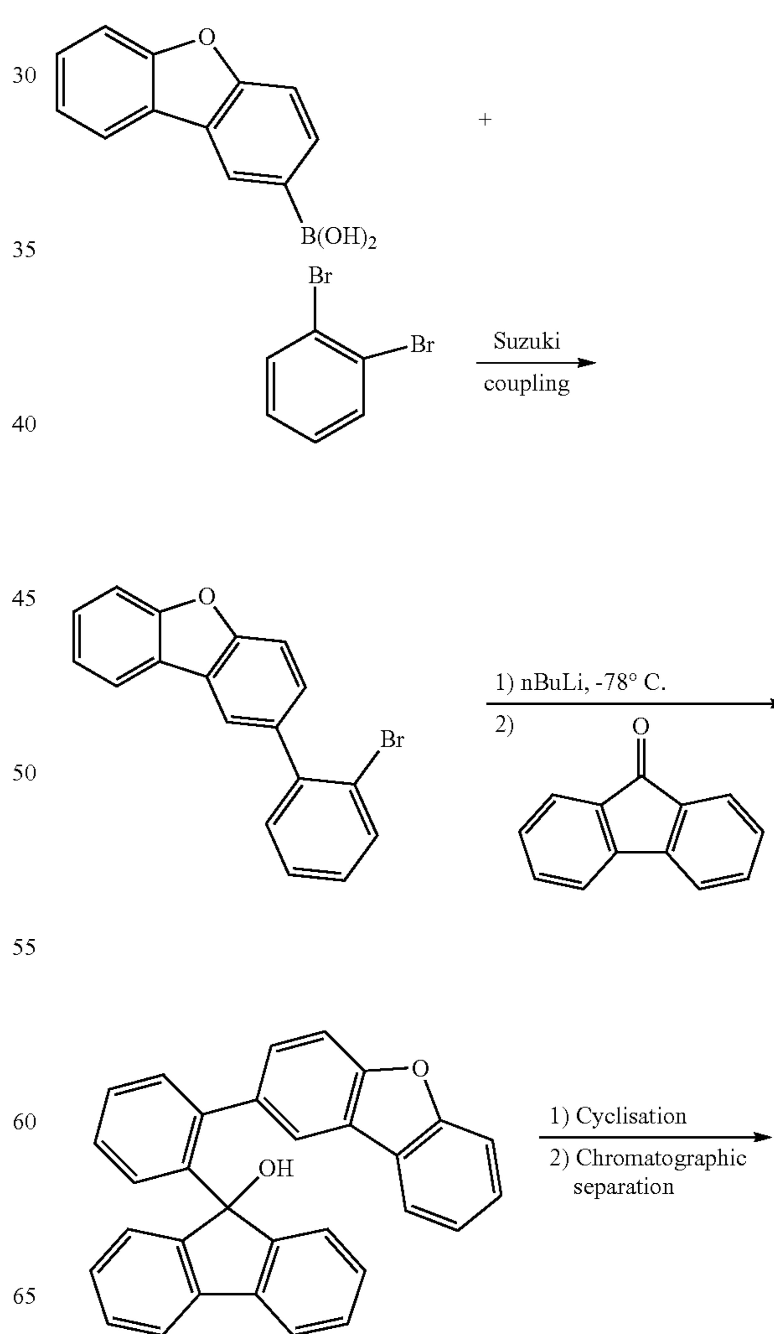
Scheme 8
