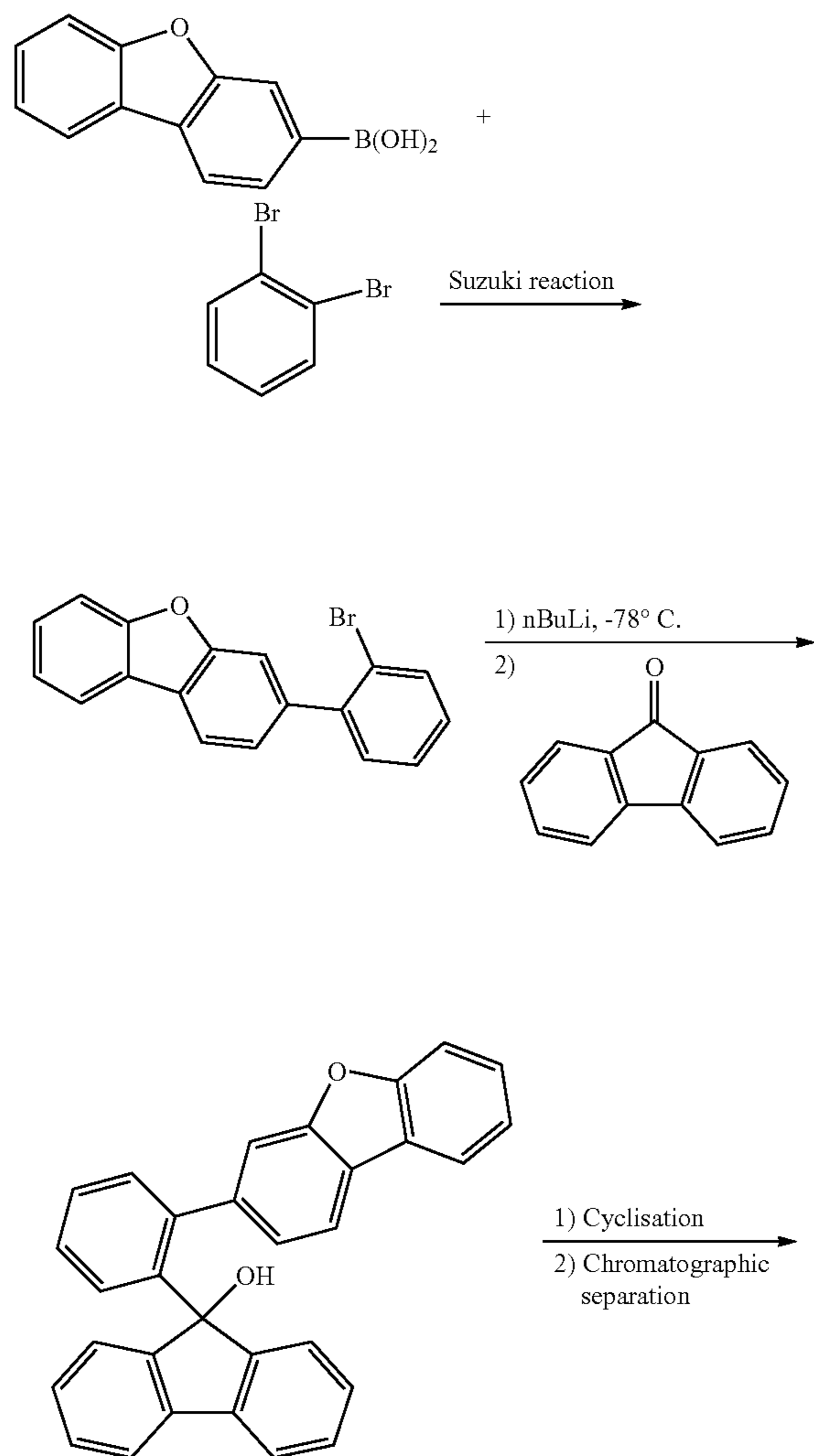
Scheme 7
