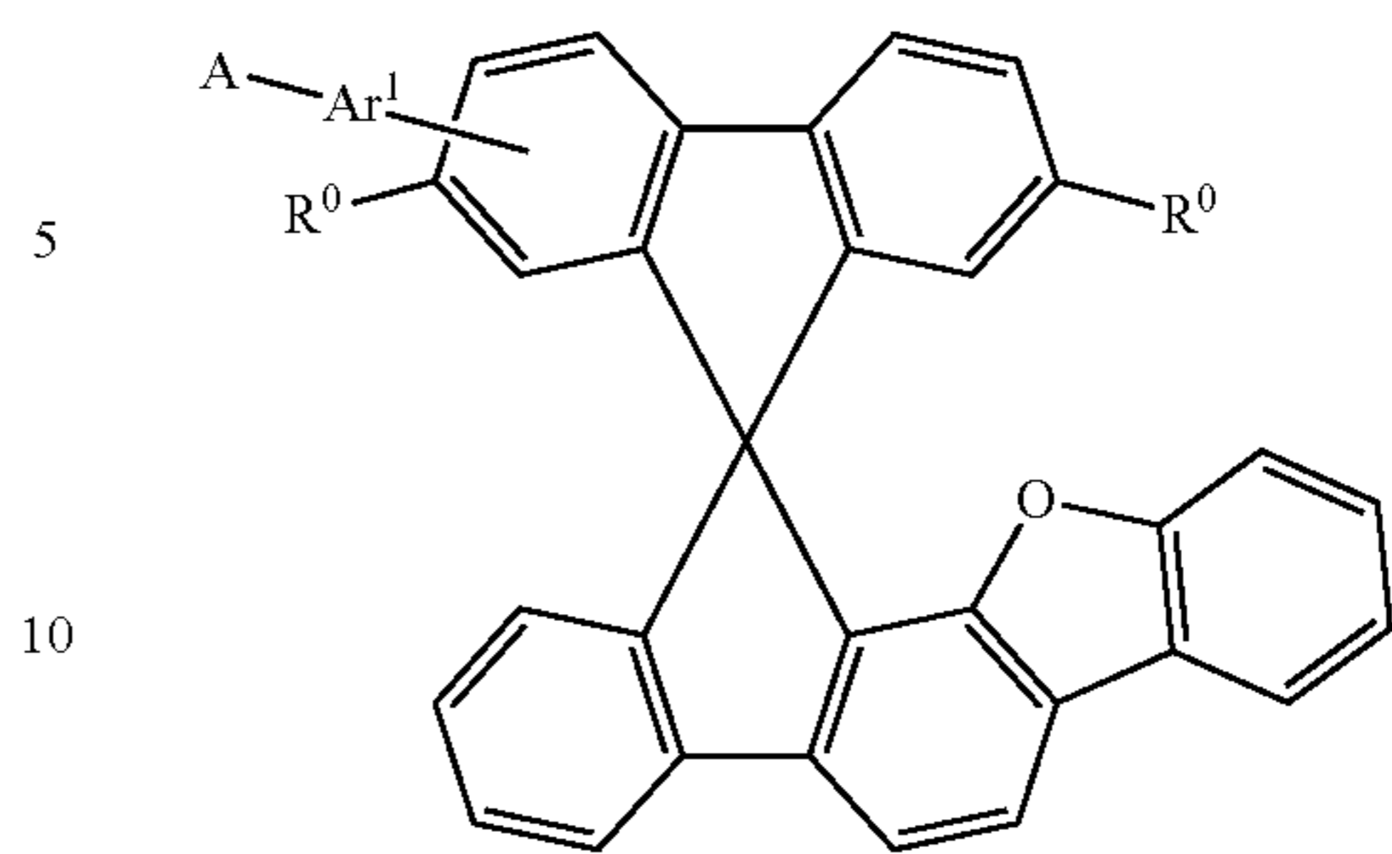
formula (I-1'')
