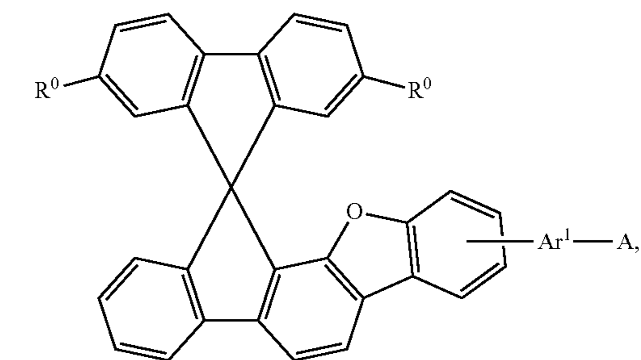
formula (I-18)
