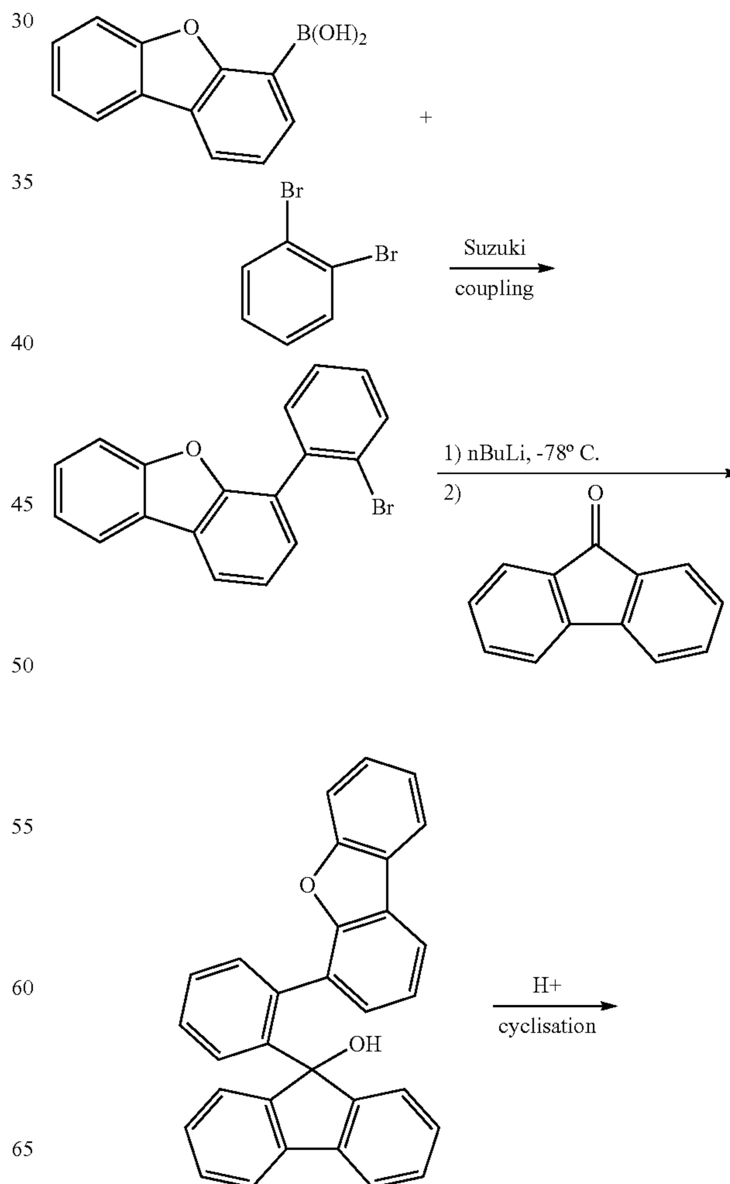
Scheme 1
