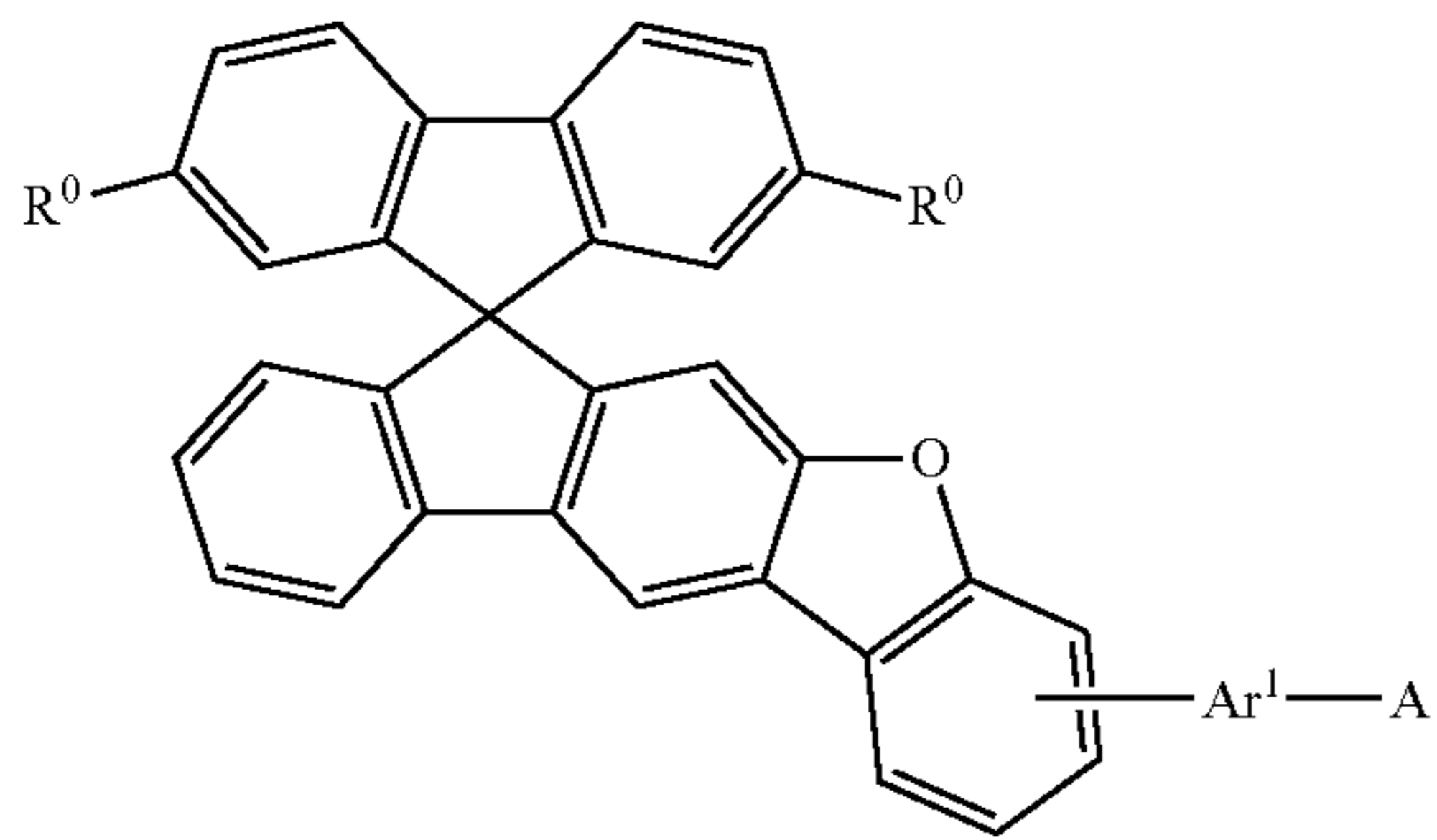
formula (I-13)
