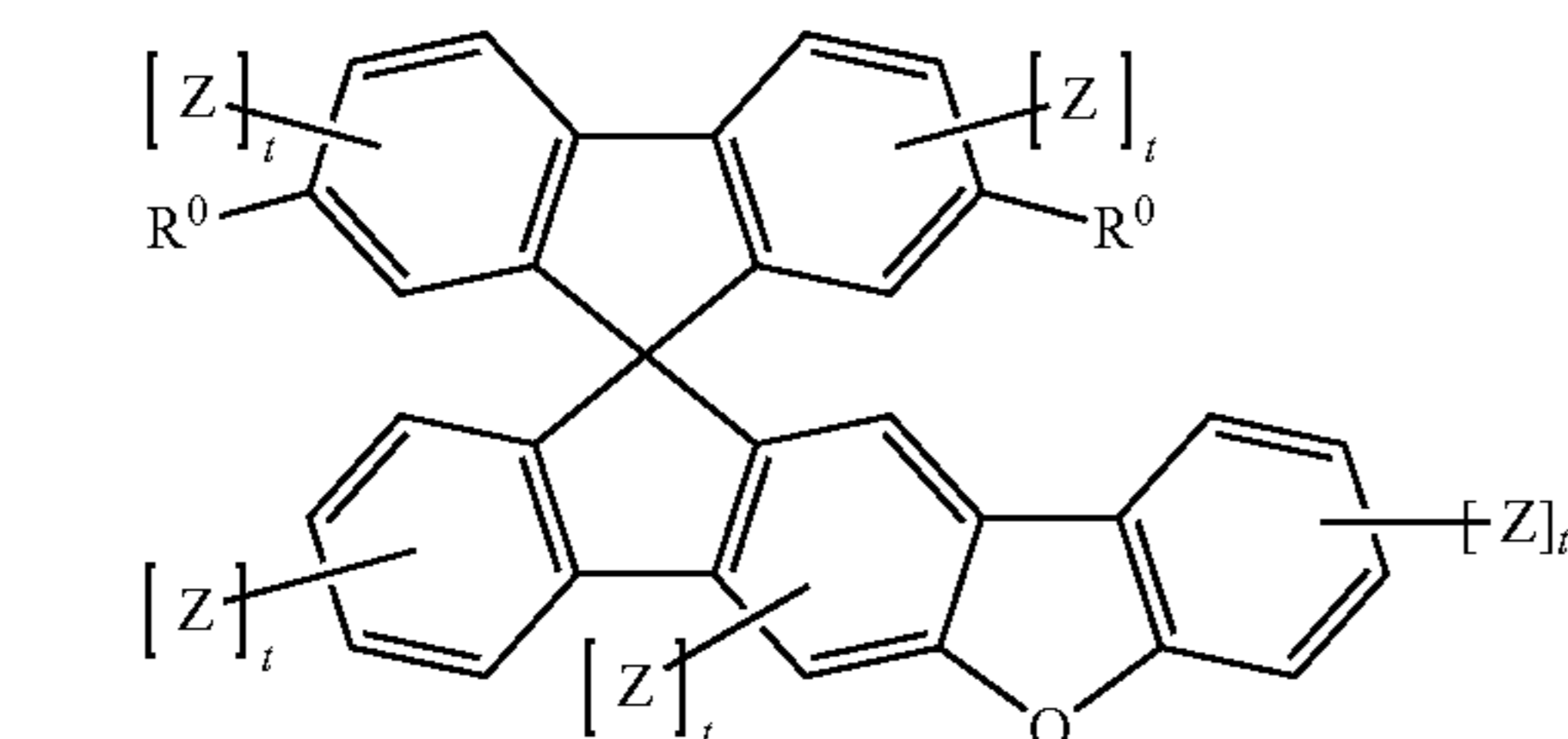
formula (II-5)
