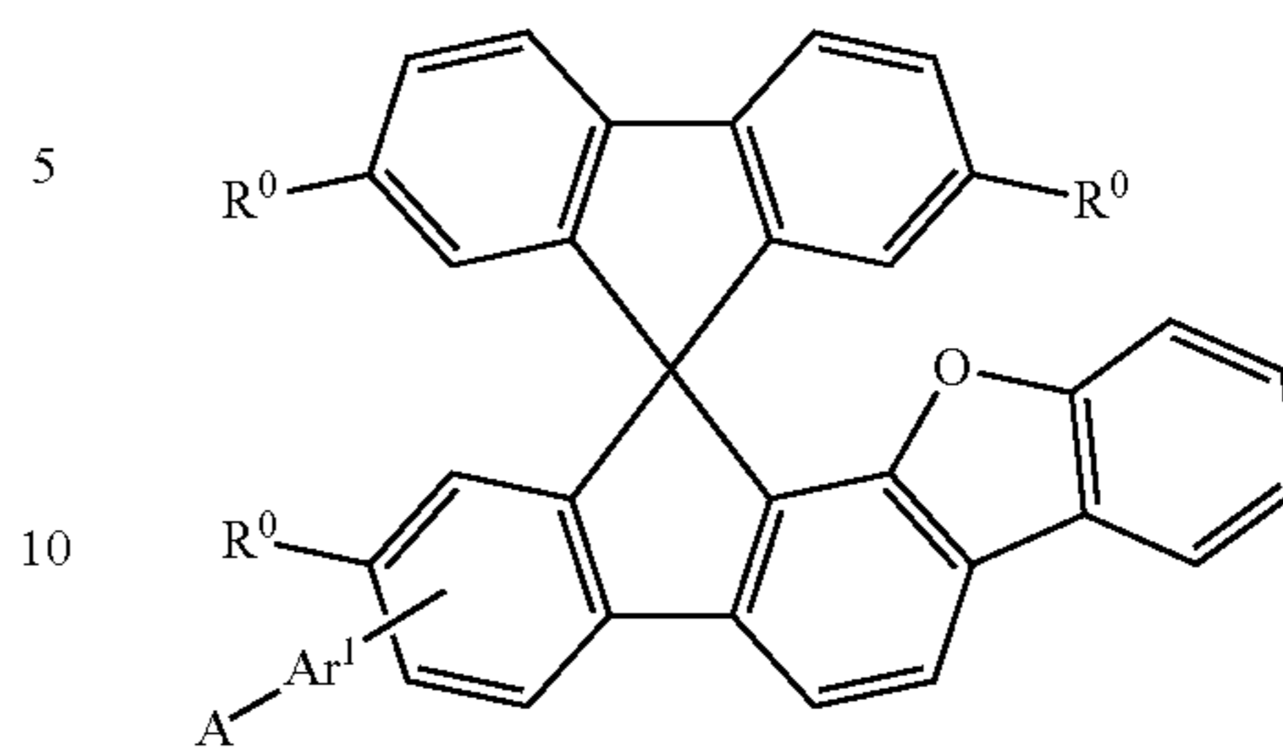
formula (I-8-A)
