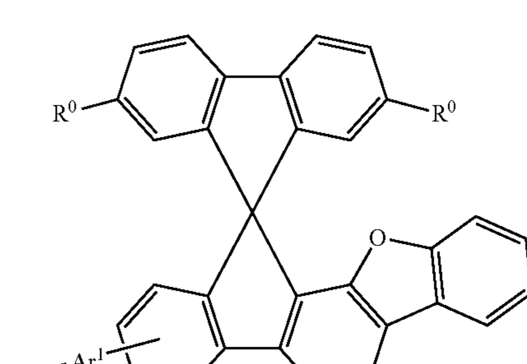
formula (I-17)
