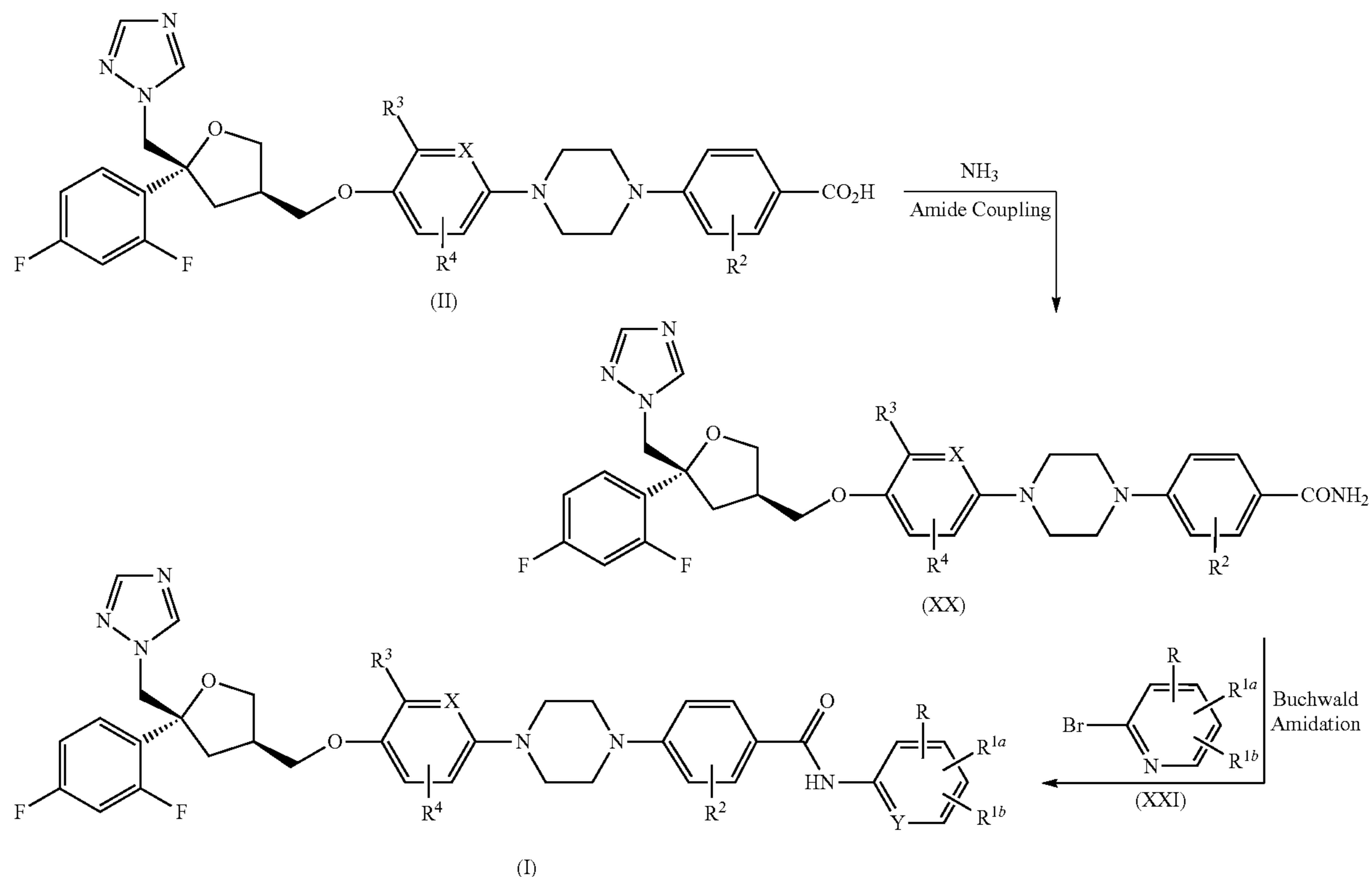
Scheme 3
