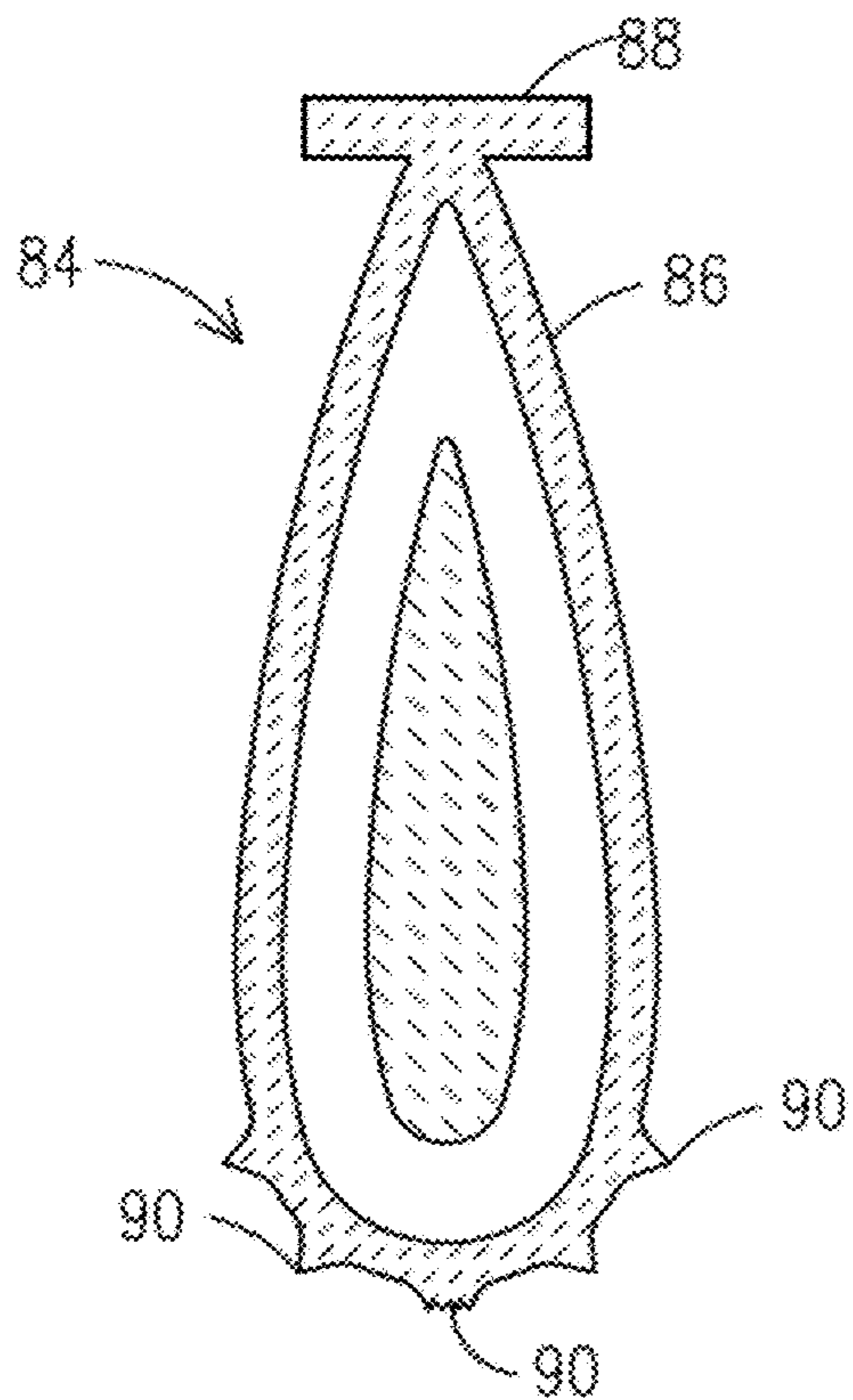
FIG. 9 PRIOR ART
