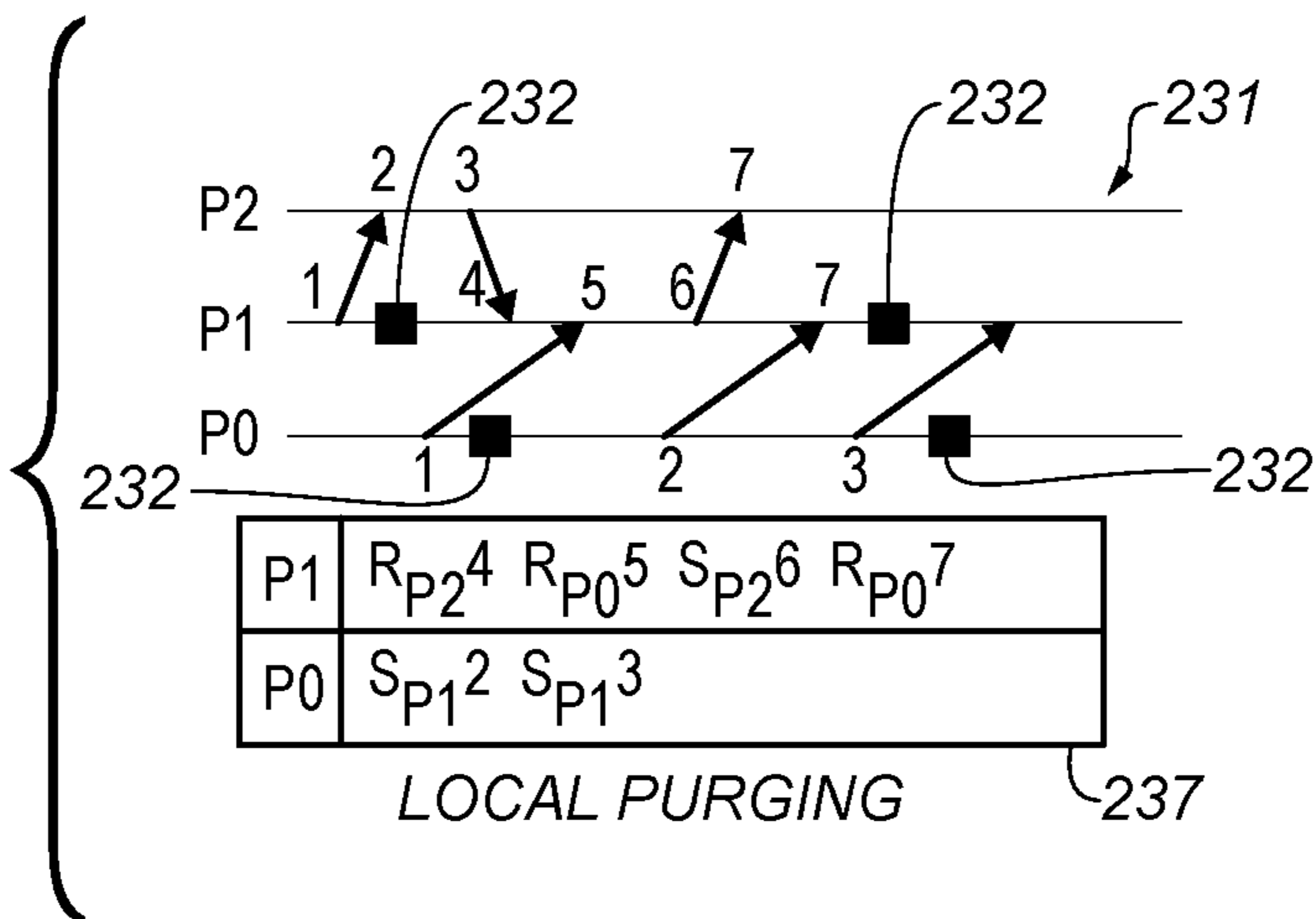
FIG. 2C PRIOR ART
