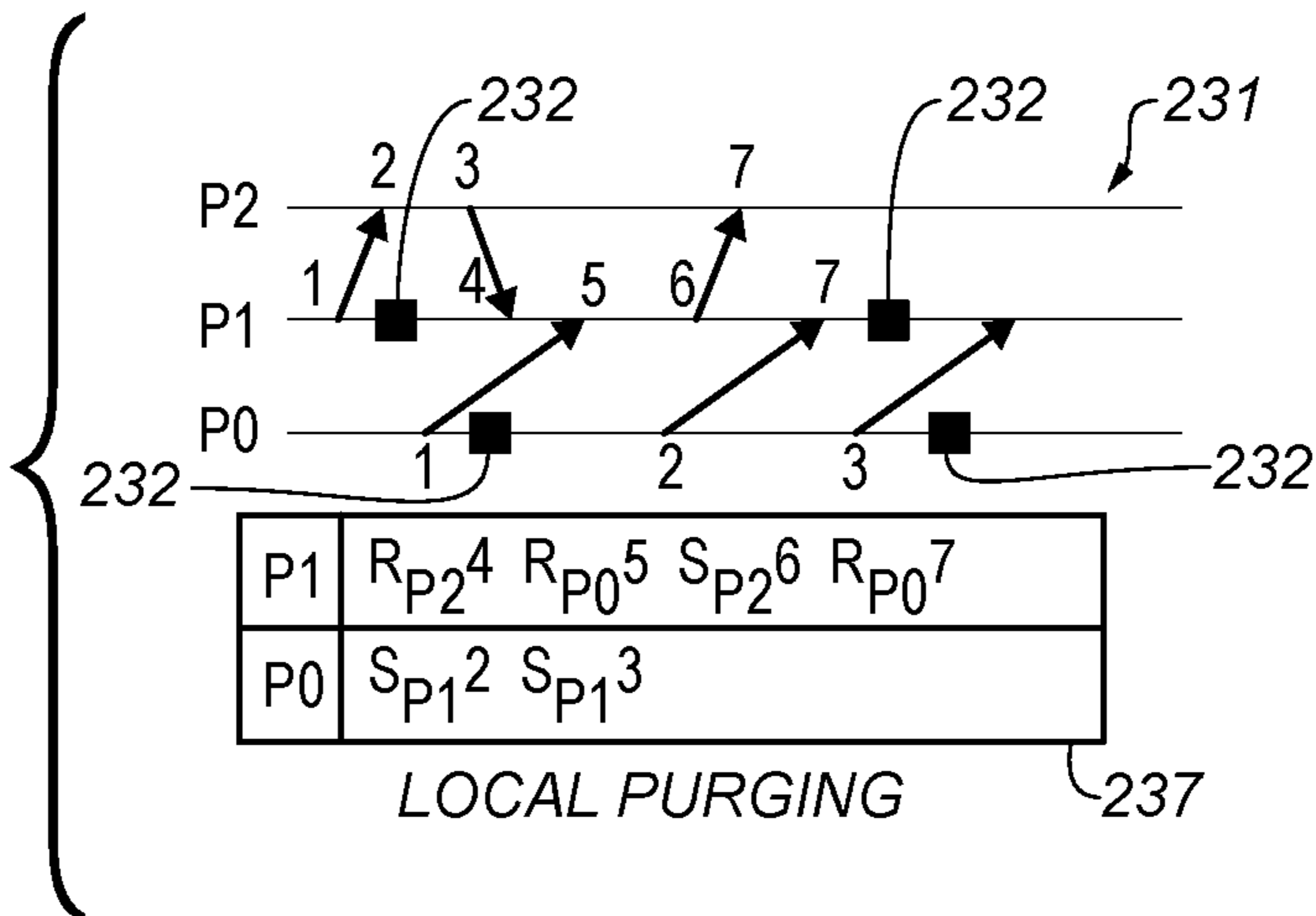
FIG. 2C PRIOR ART
