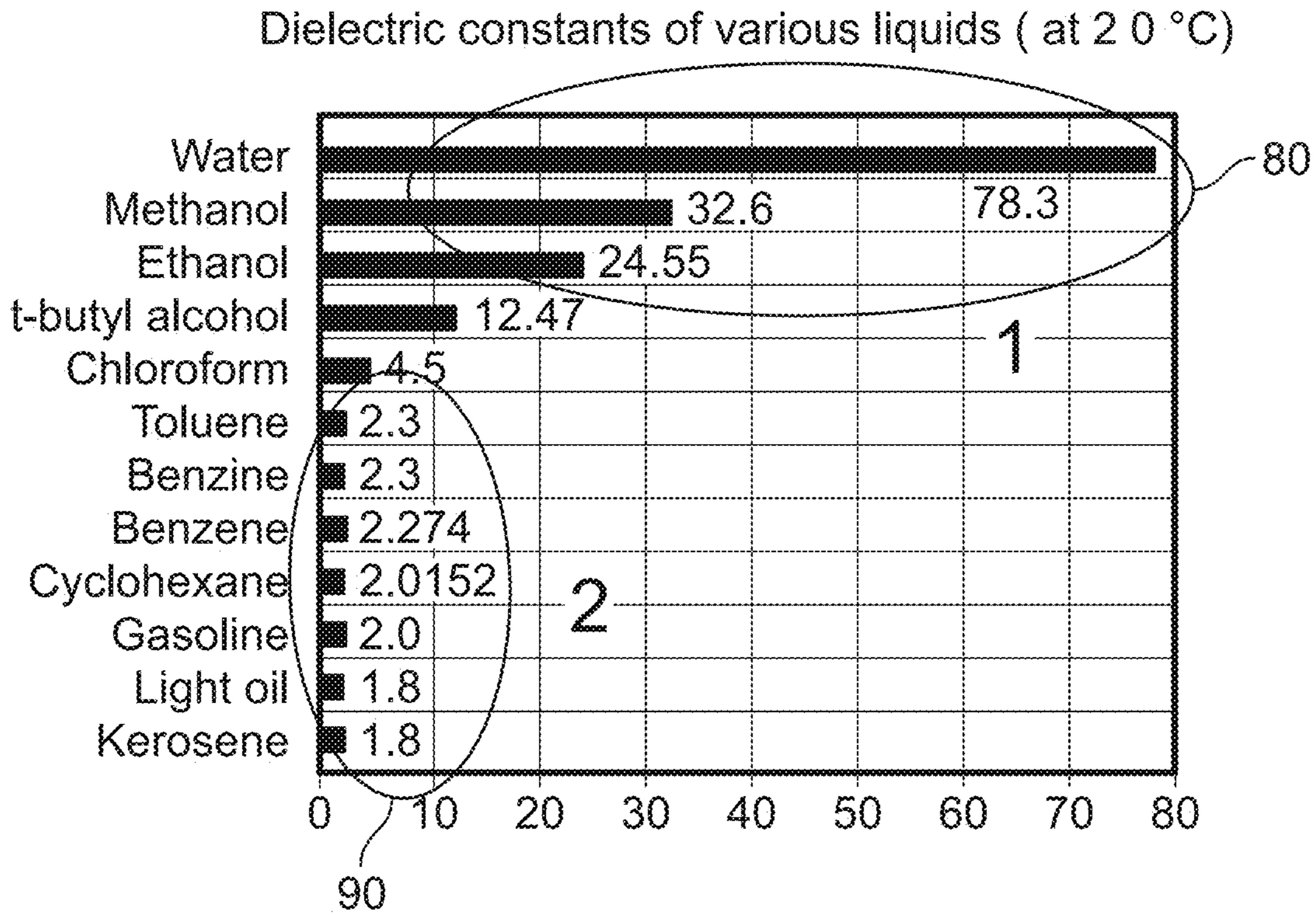
FIG. 3 Prior Art
