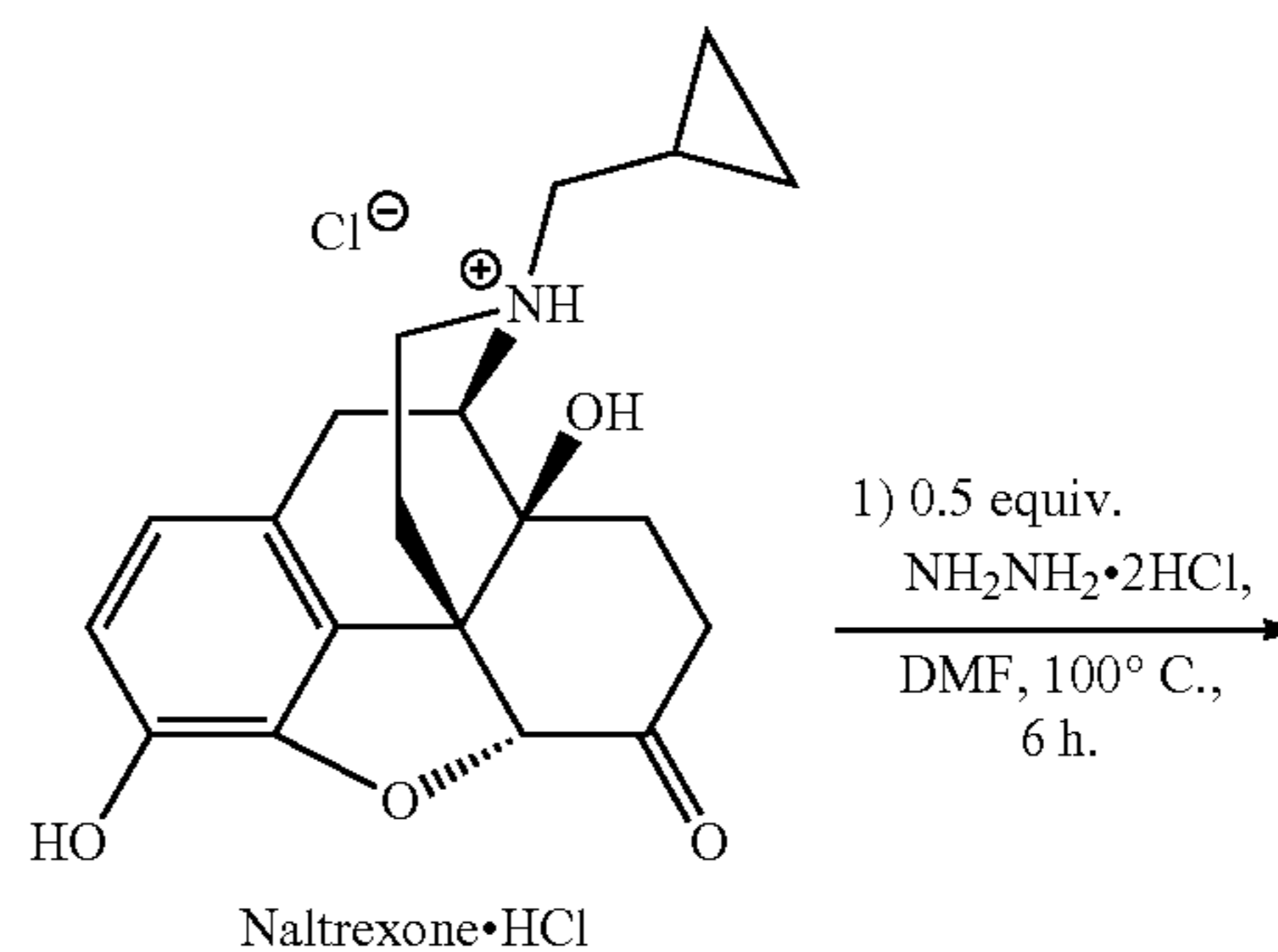
Scheme 1
