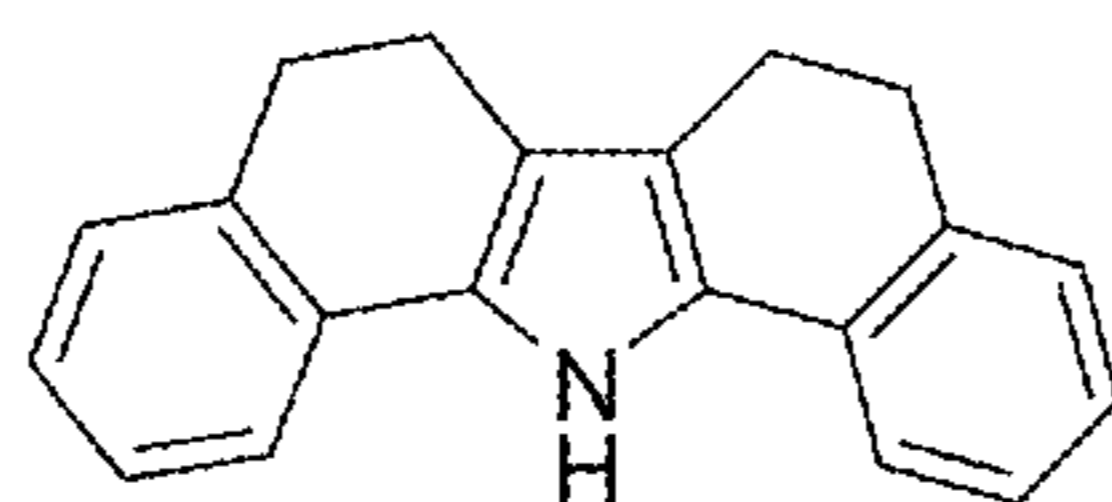
6,7,8,13-Tetrahydro-5H-dibenzo[a,b]carbazole
