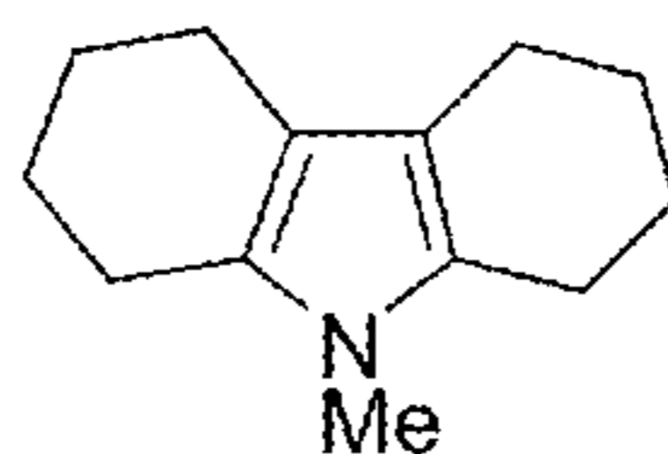
9-Methyl-2,3,4,5,6,7,8,9-octahydro-1H-carbazole
