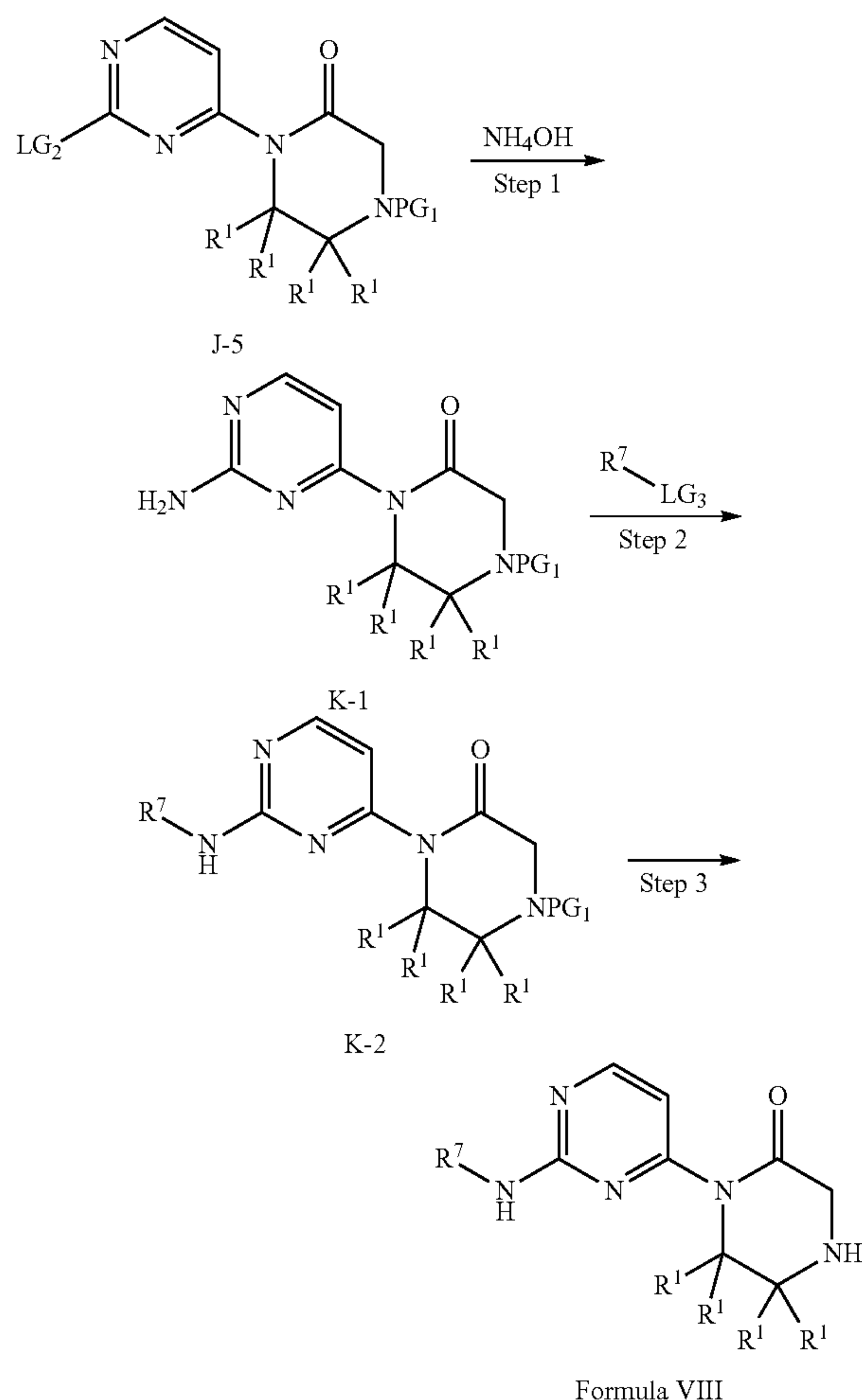
Scheme 11
