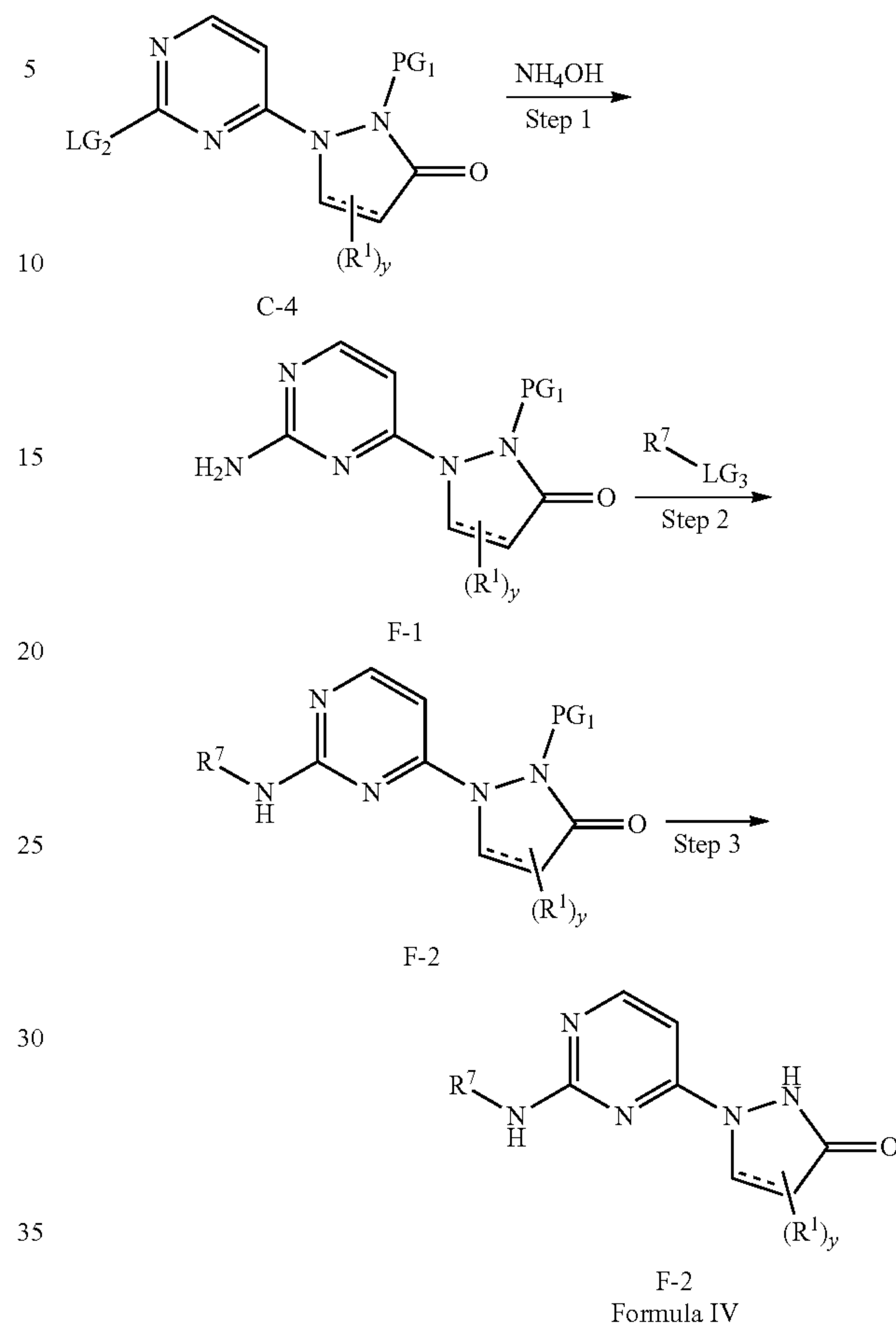
Scheme 6
