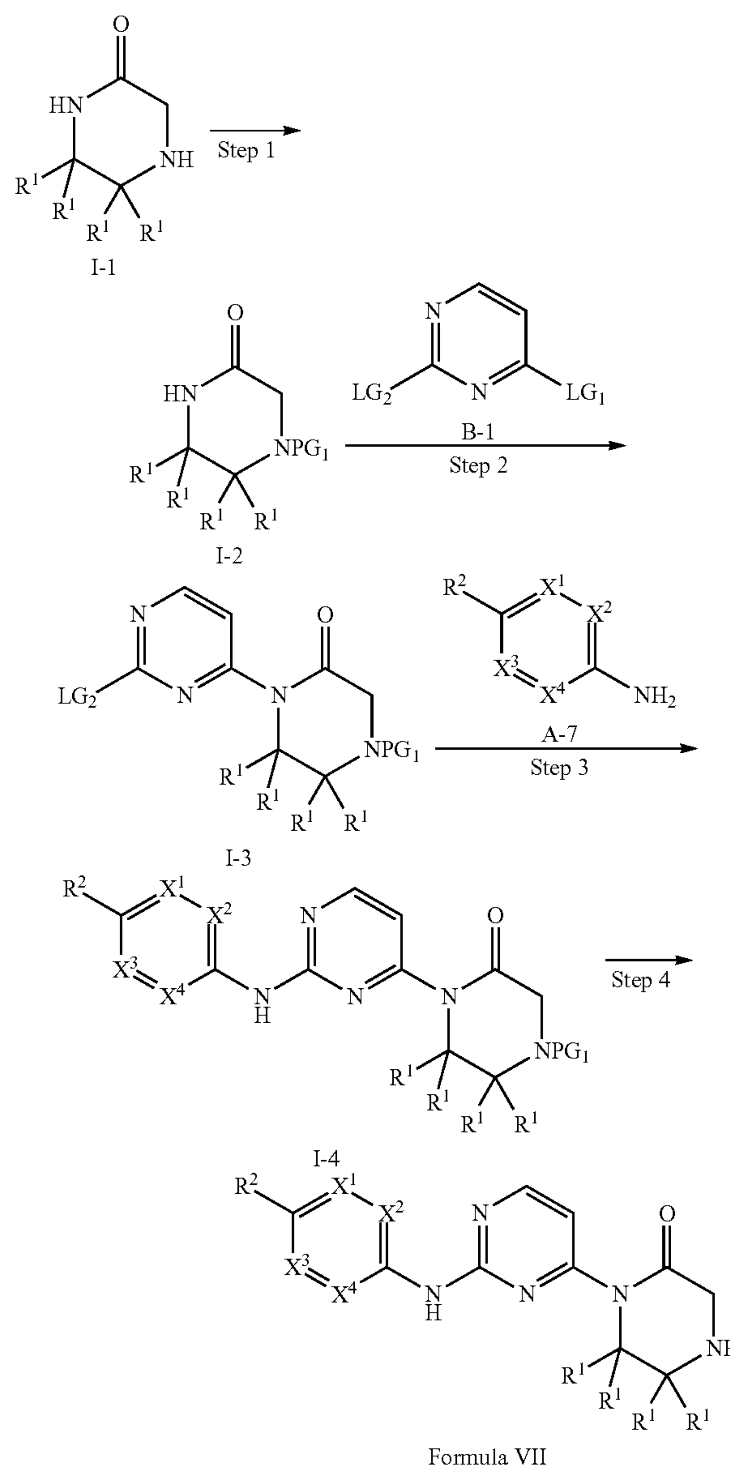
Scheme 9
