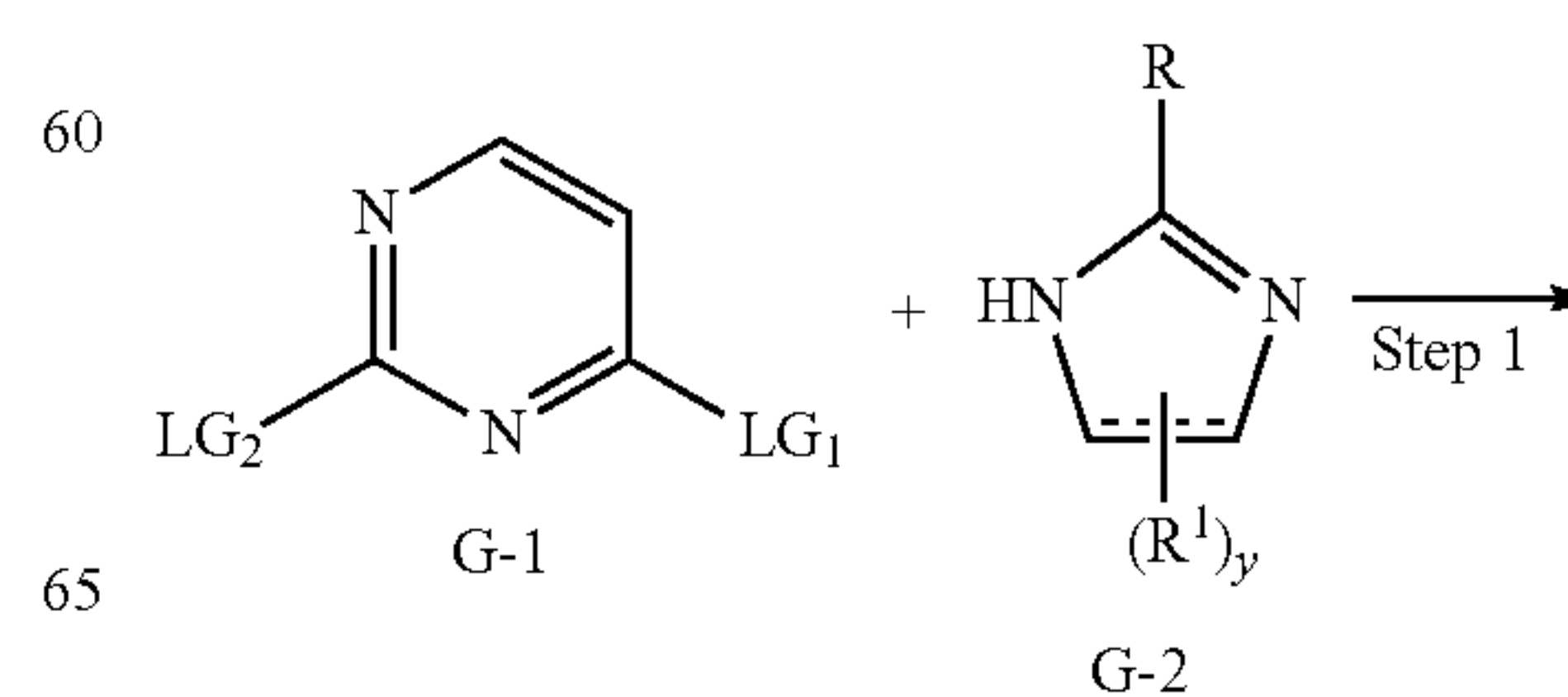
Scheme 7
