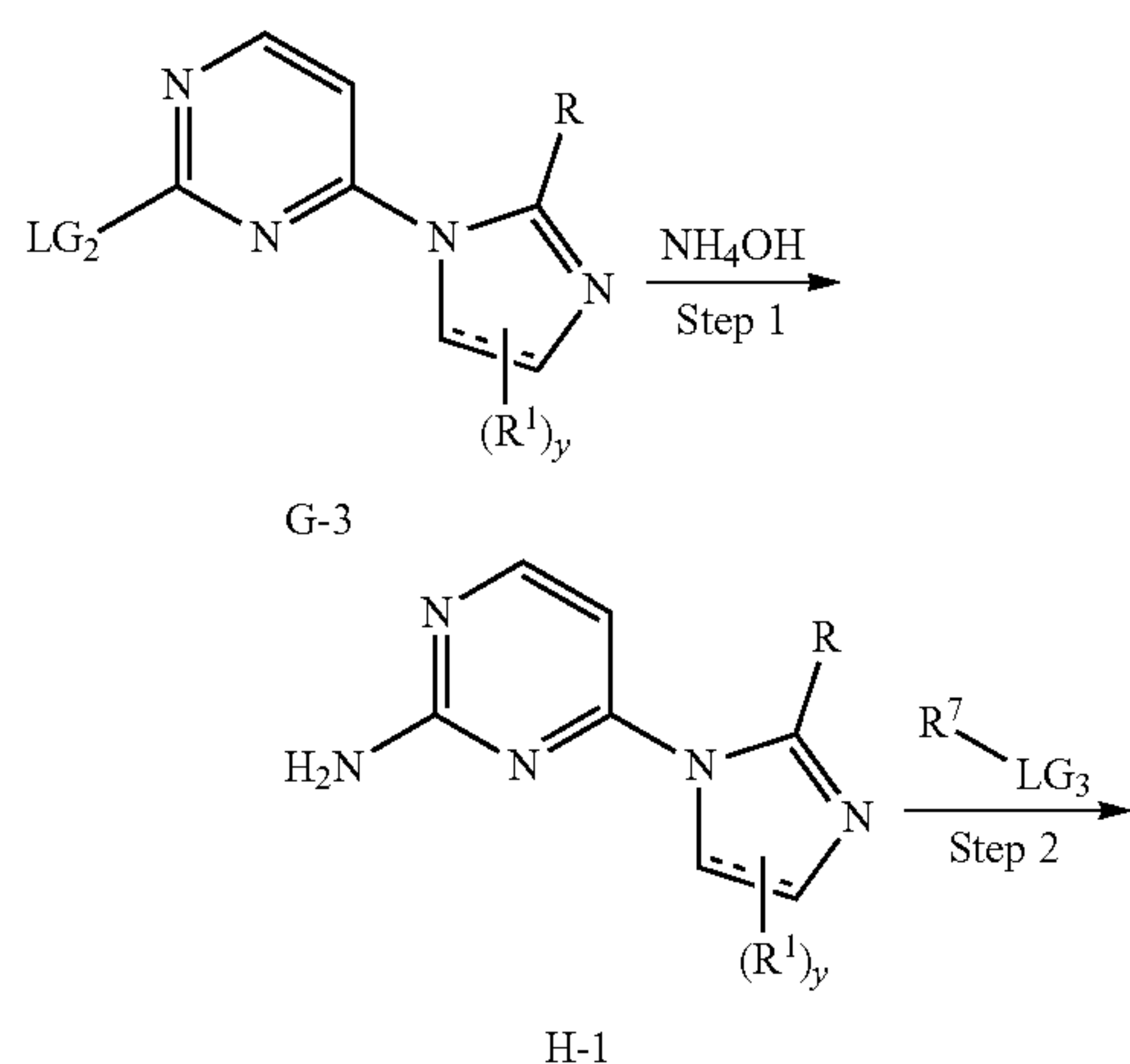
Scheme 8
