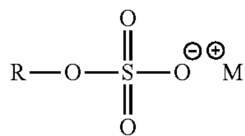
Alkyl sulfates
