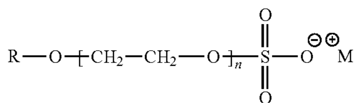
Alkyl ether sulfates
