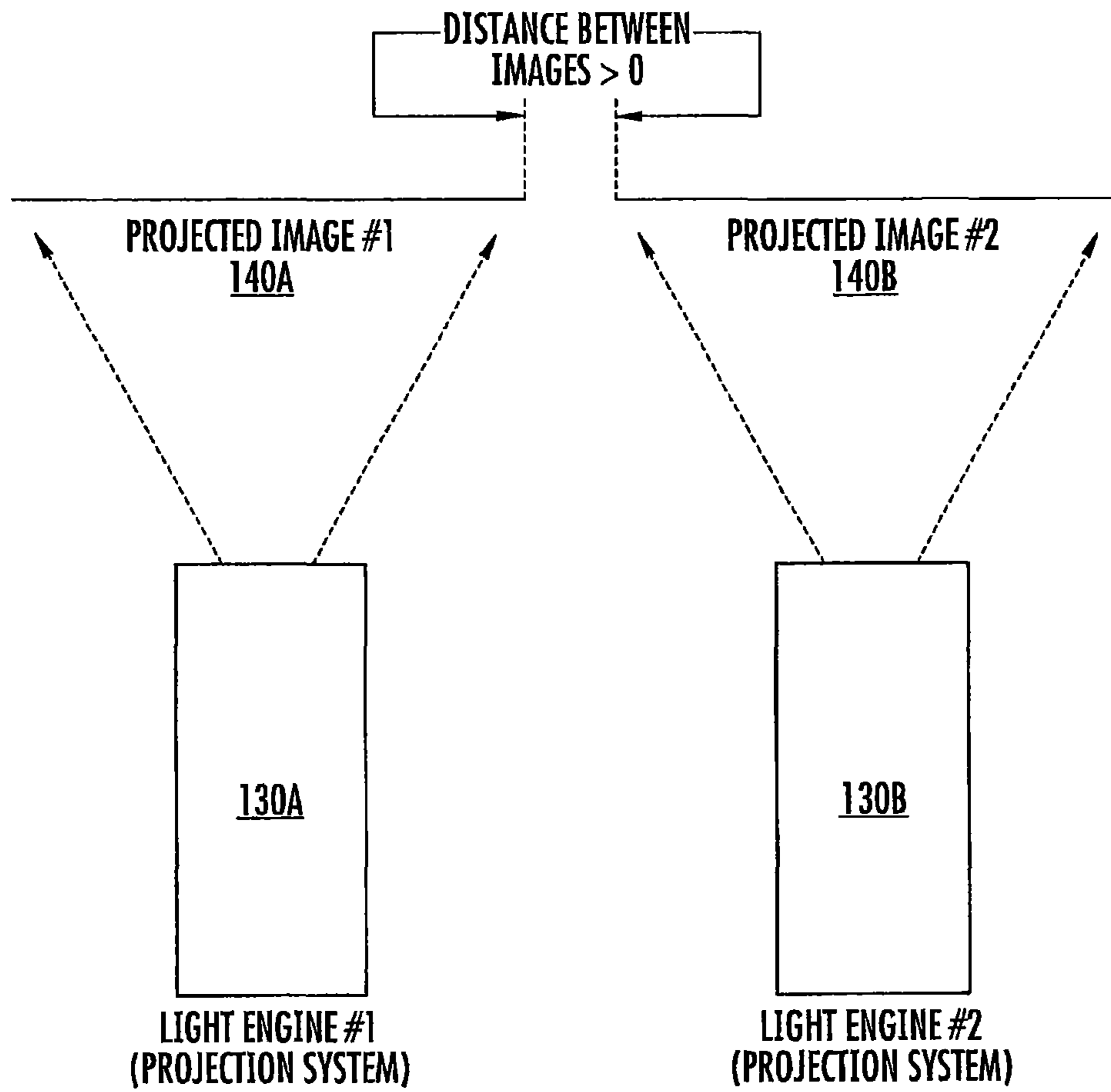
SIDE VIEW TWO LIGHT ENGINES
