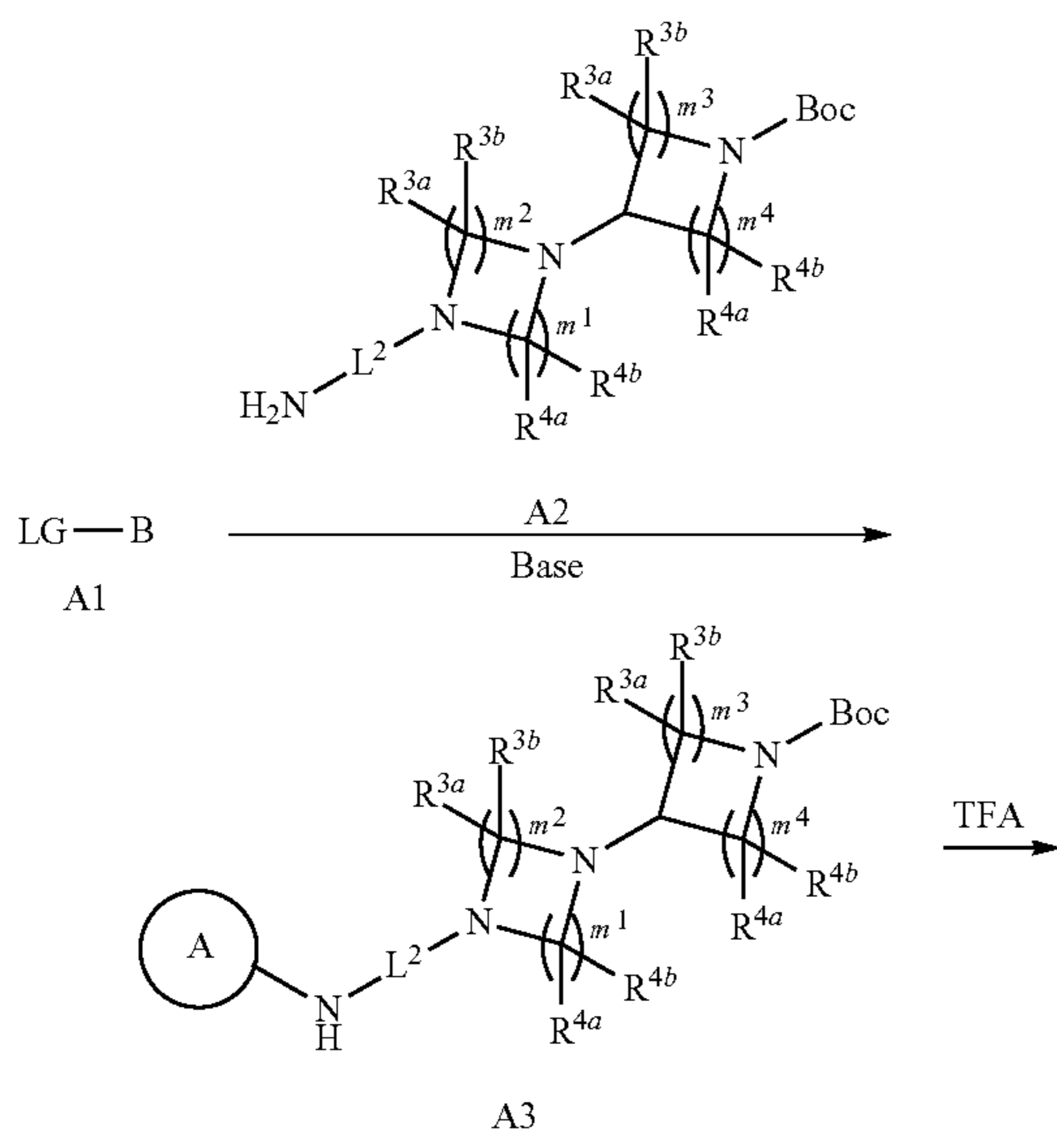
General Reaction Scheme 1
