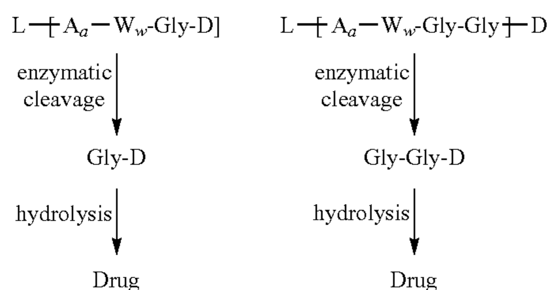
Scheme 1
