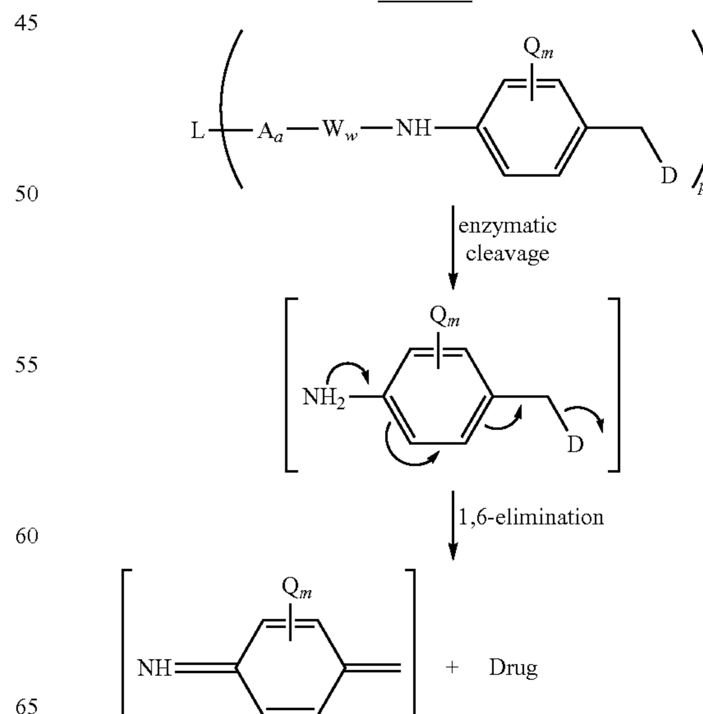
Scheme 3
