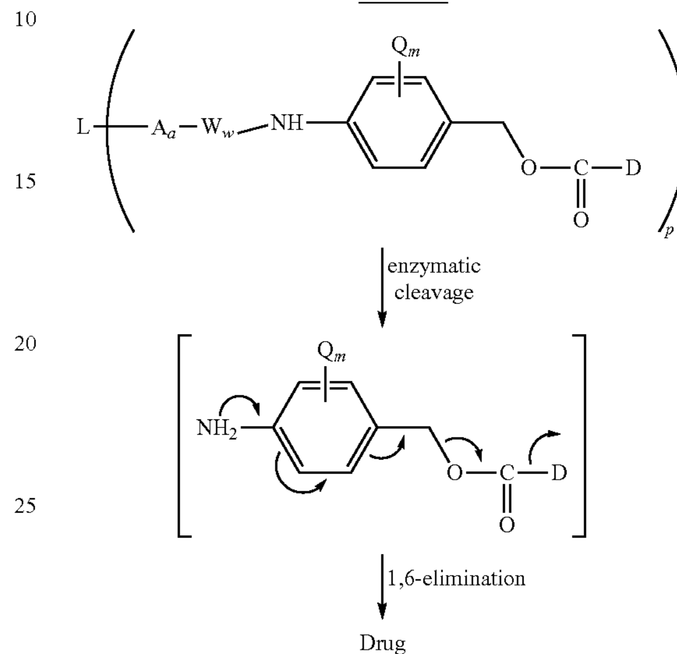
Scheme 2
