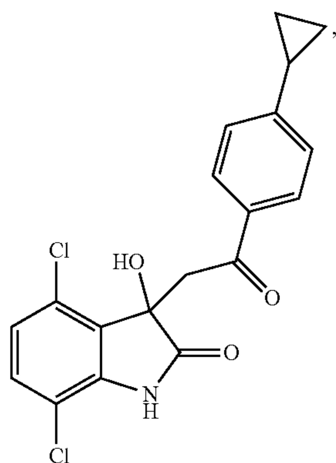
TK216
