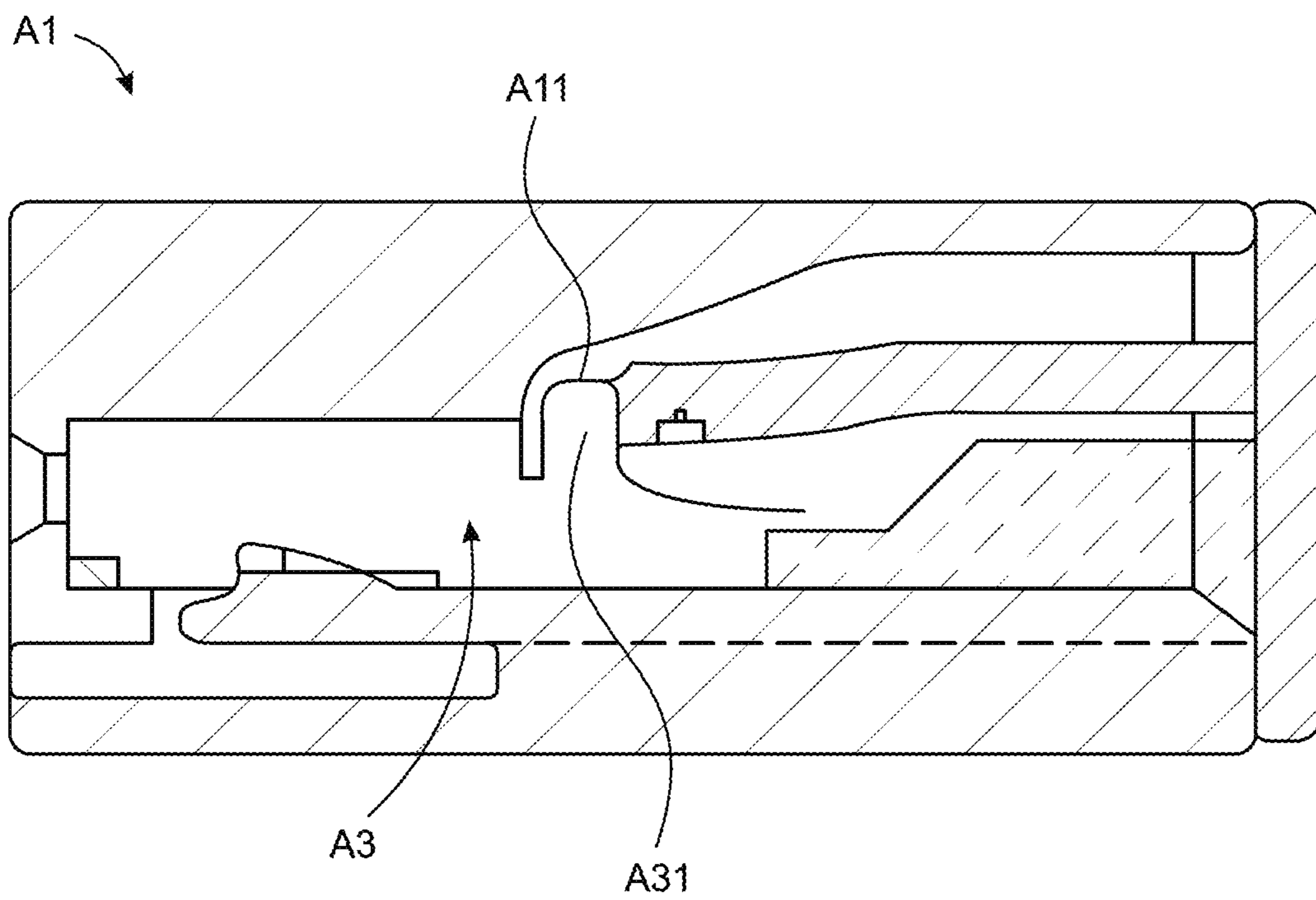
FIG. 2 (Prior Art)
