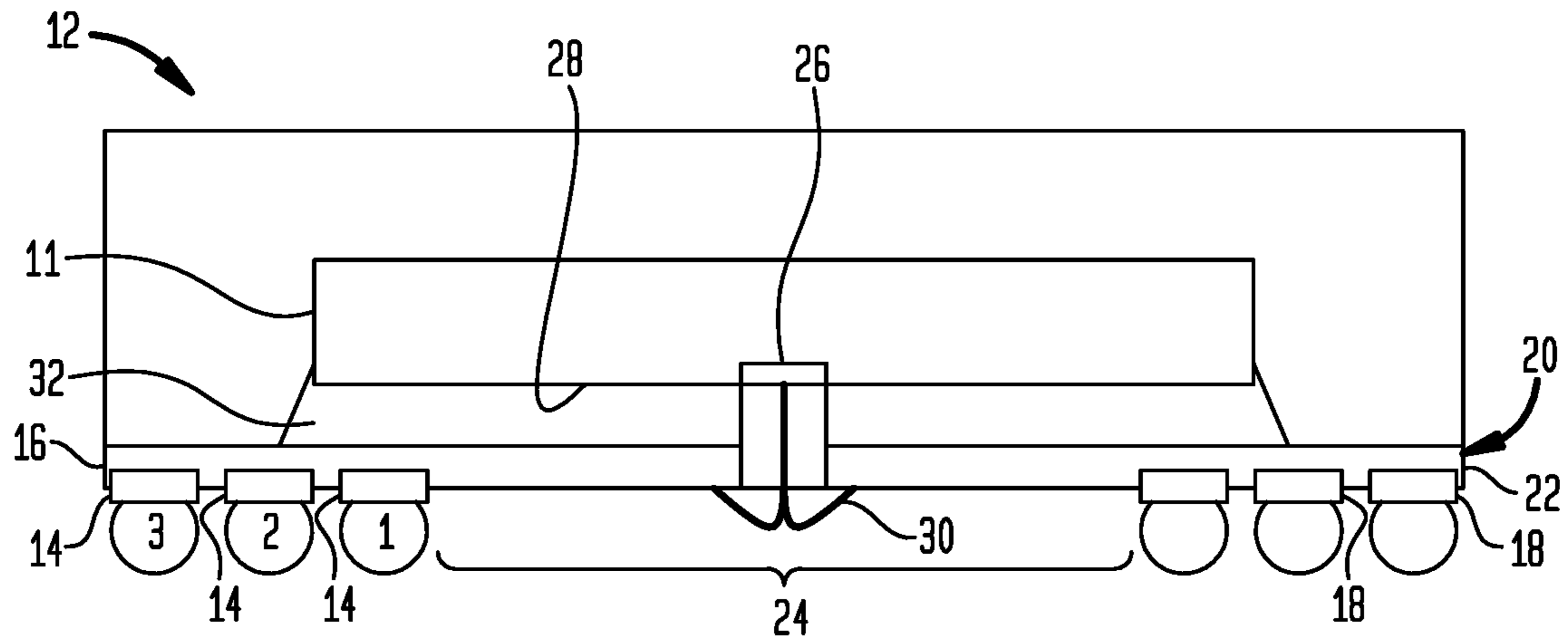
FIG. 1 (PRIOR ART)
