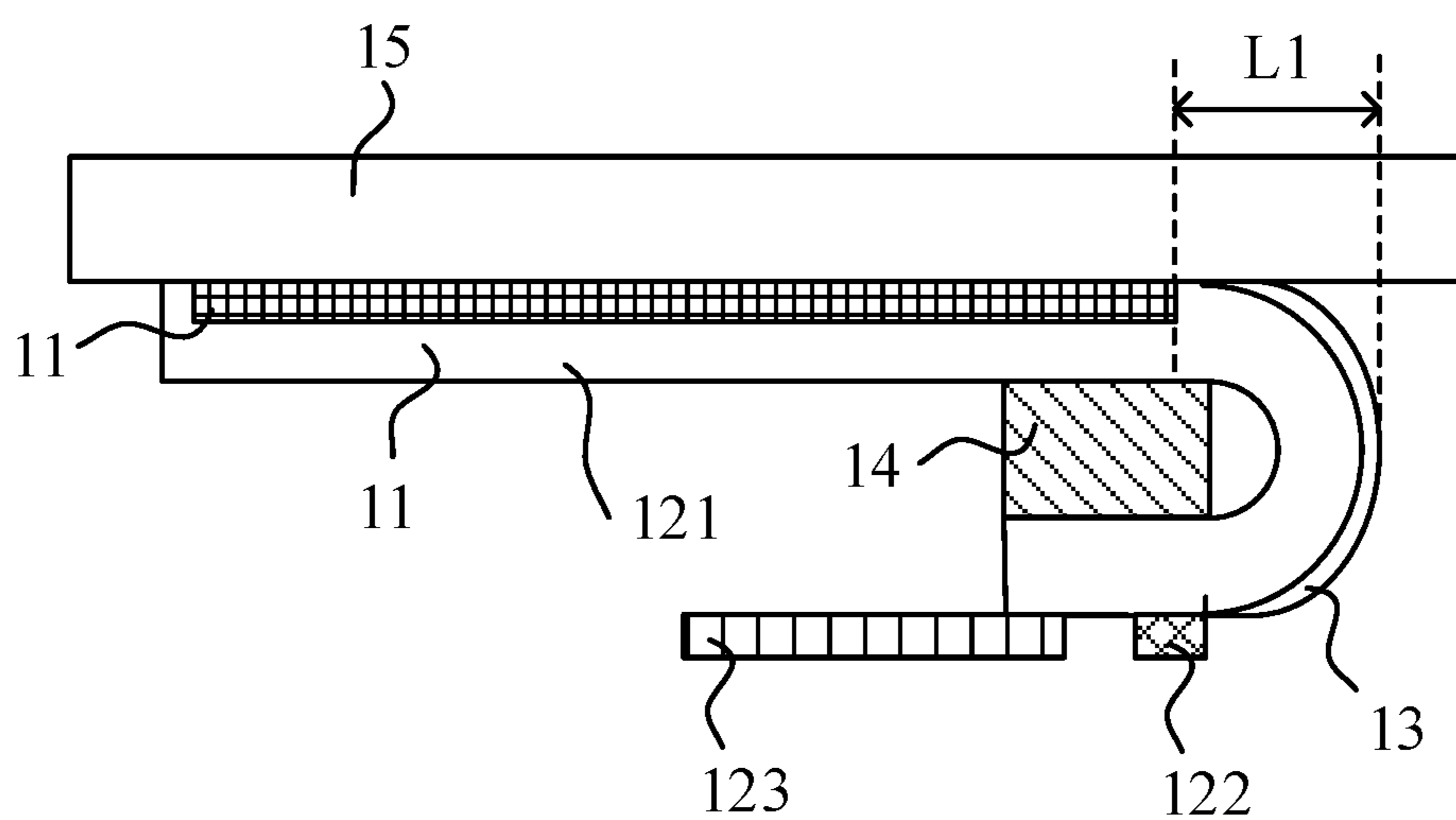
Fig. 10 (related art)
