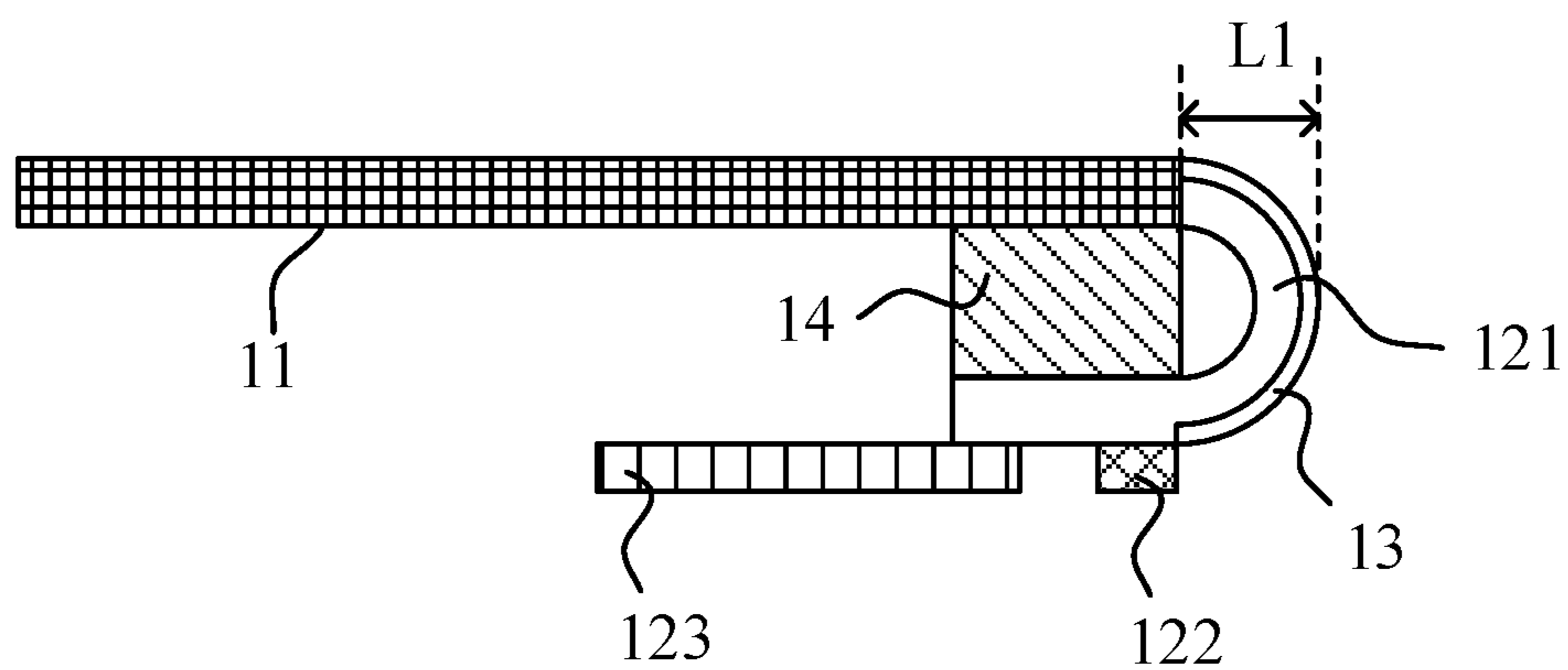
Fig. 9 (related art)
