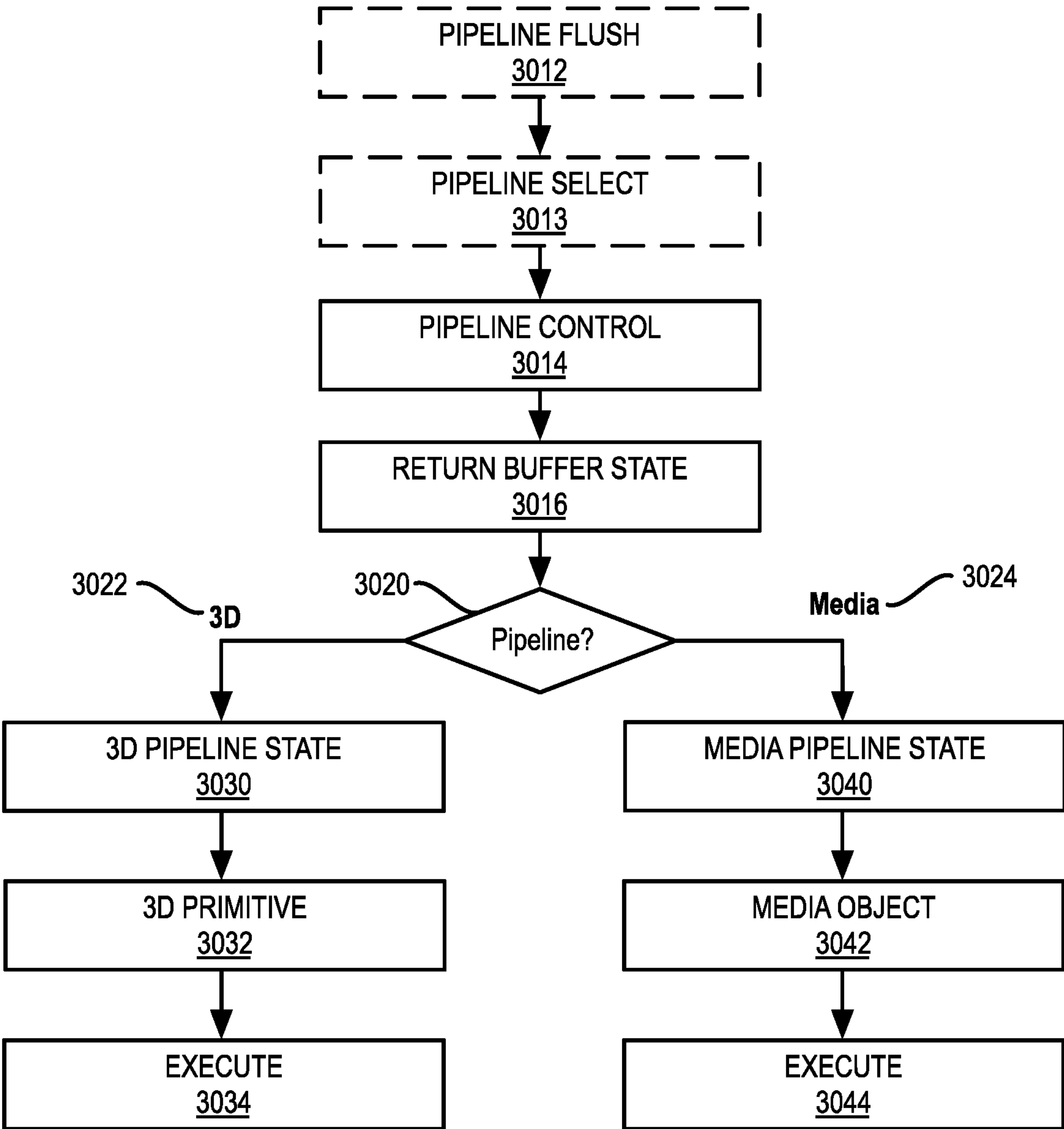
FIG. 30B GRAPHICS PROCESSOR COMMAND SEQUENCE 3010
