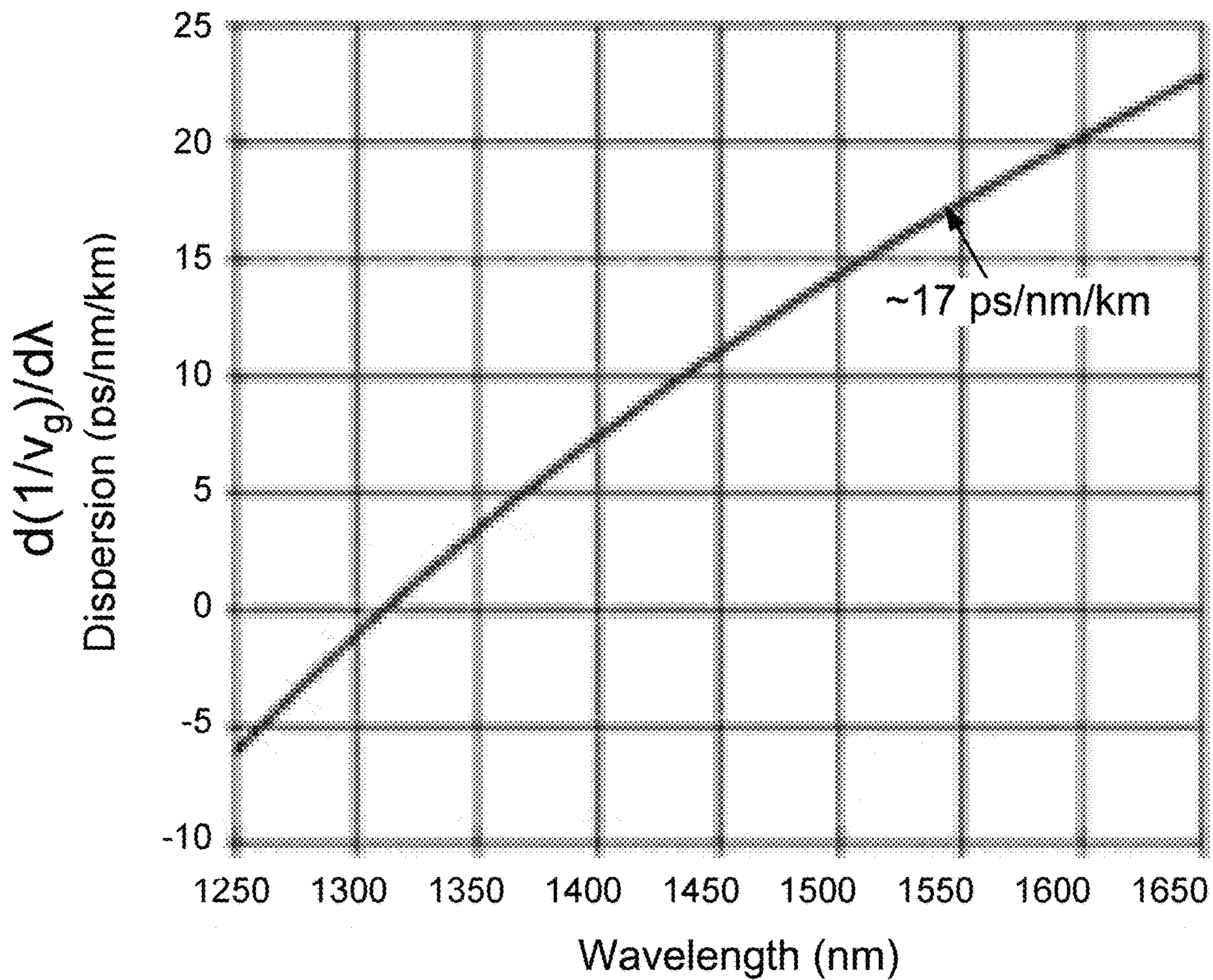
FIG. 2 (related art)
