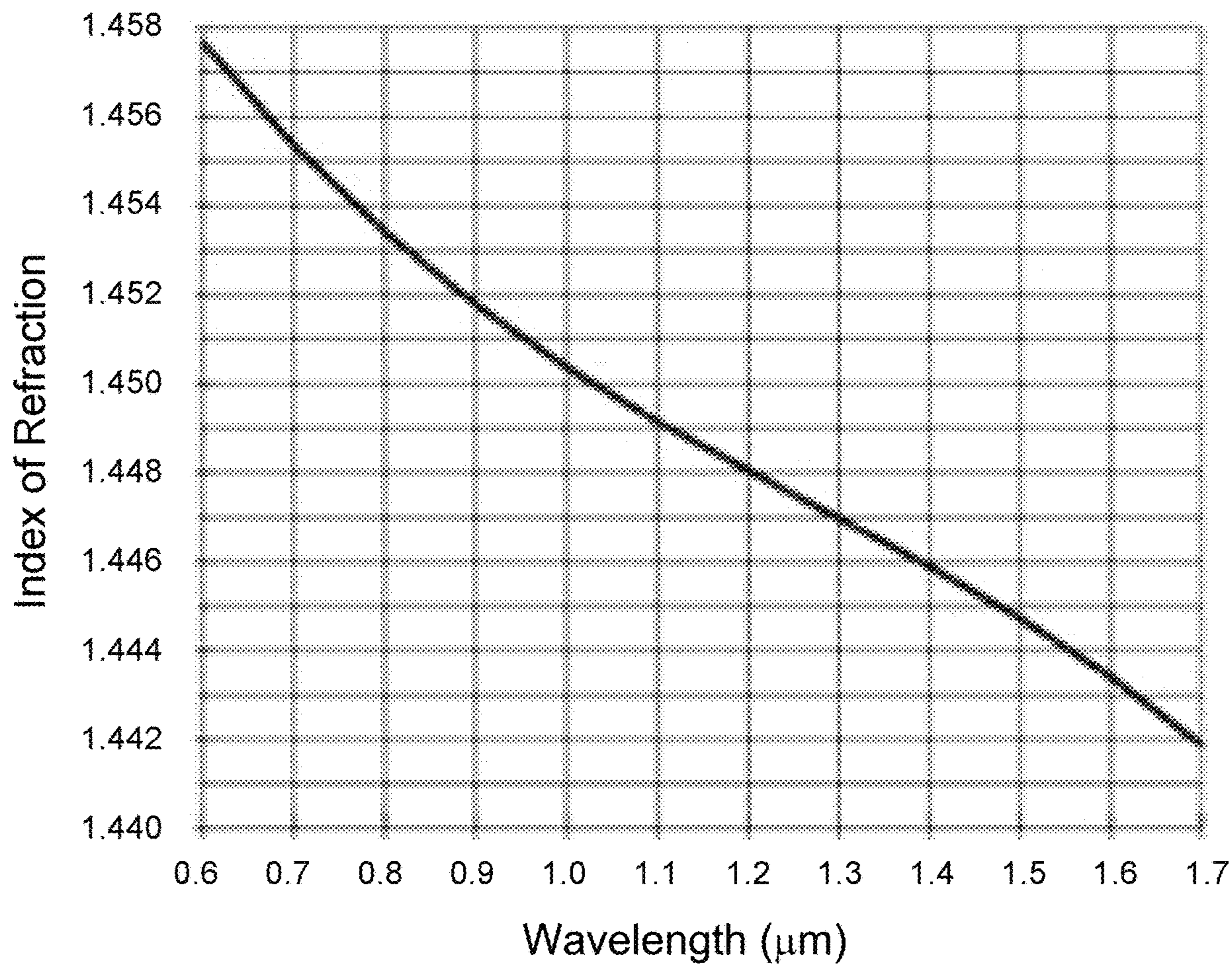
FIG. 1 (related art)
