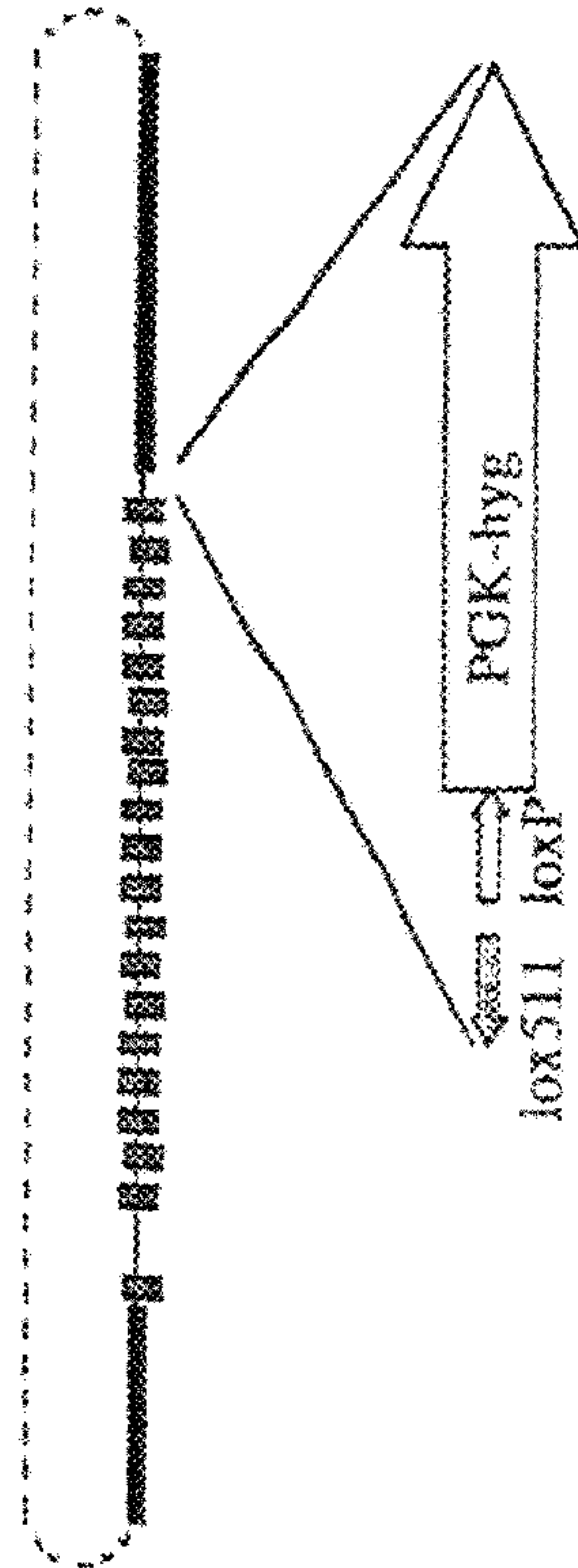
Figure 4C LTVEC2:
