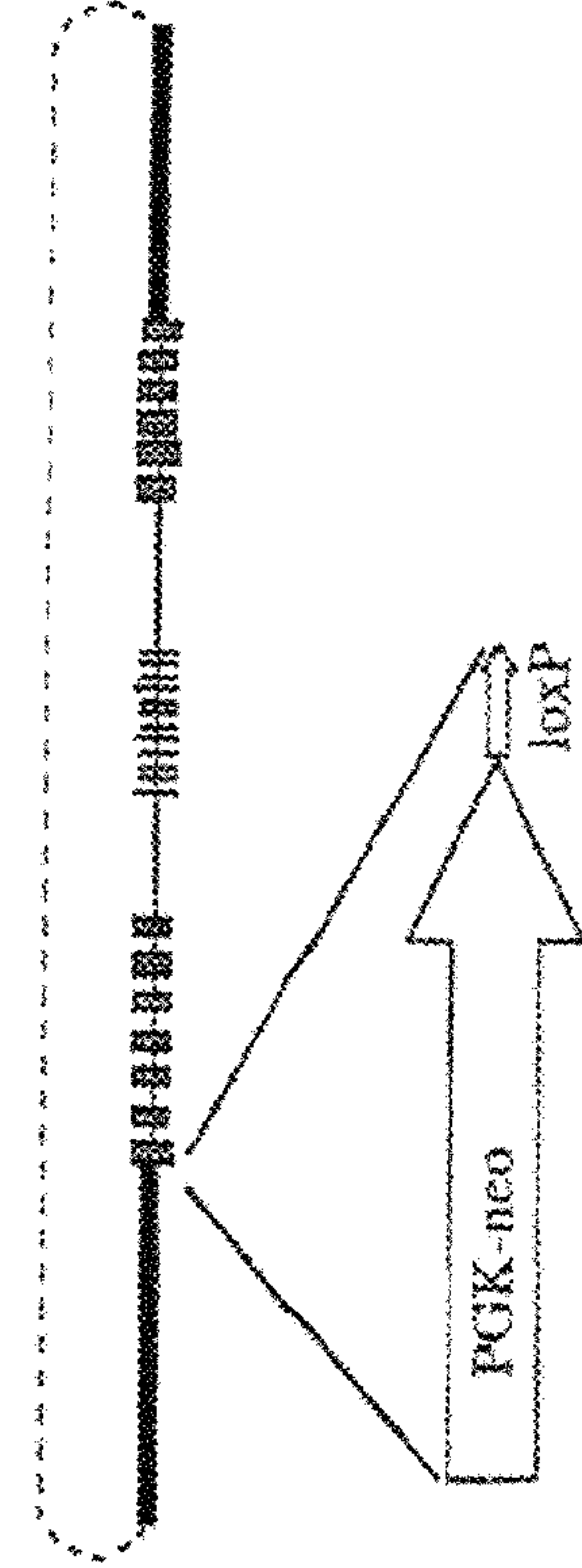
Figure 4D LTVECI:
