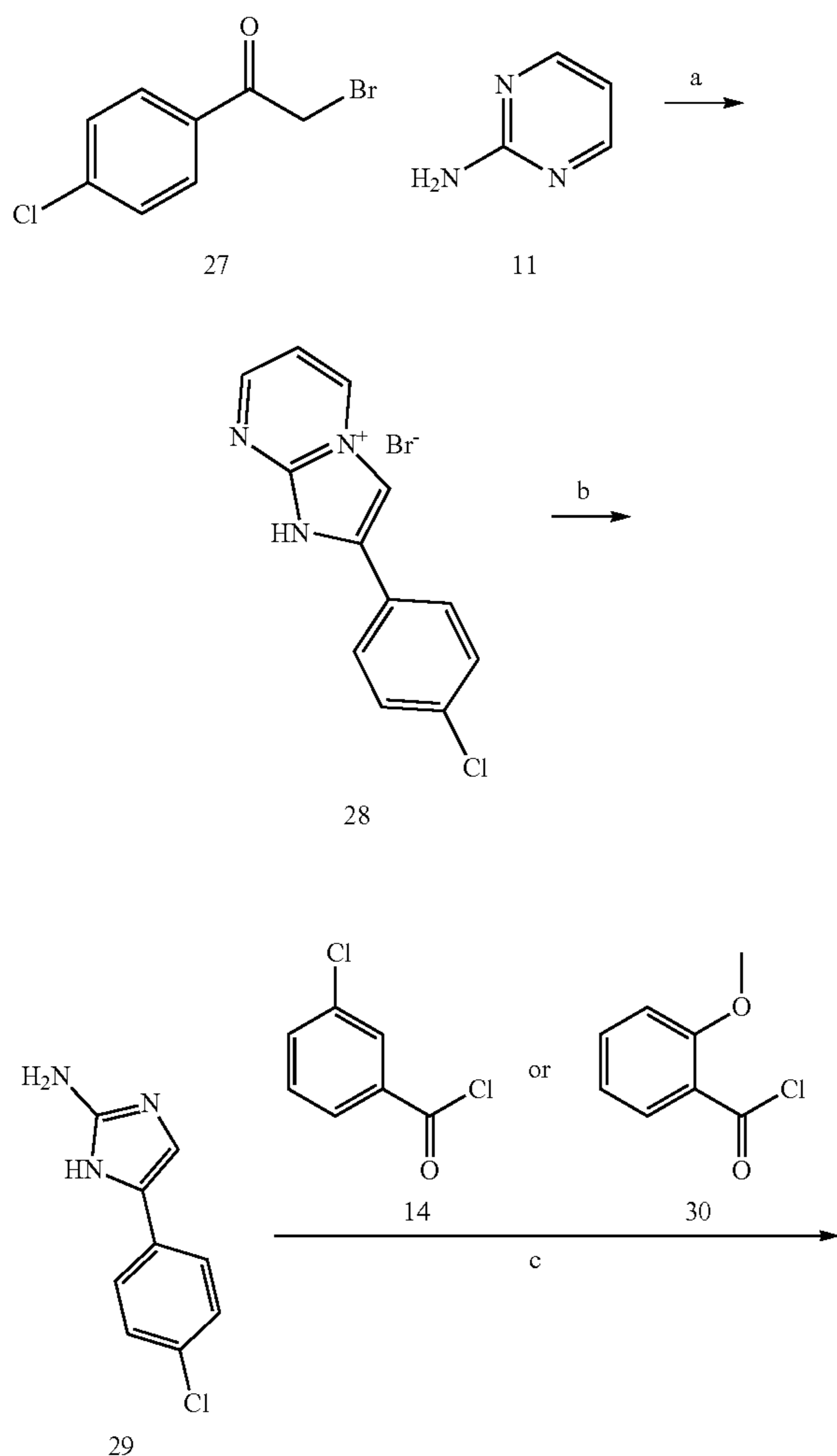
Scheme 5. Synthesis of Series II compounds 31a-
