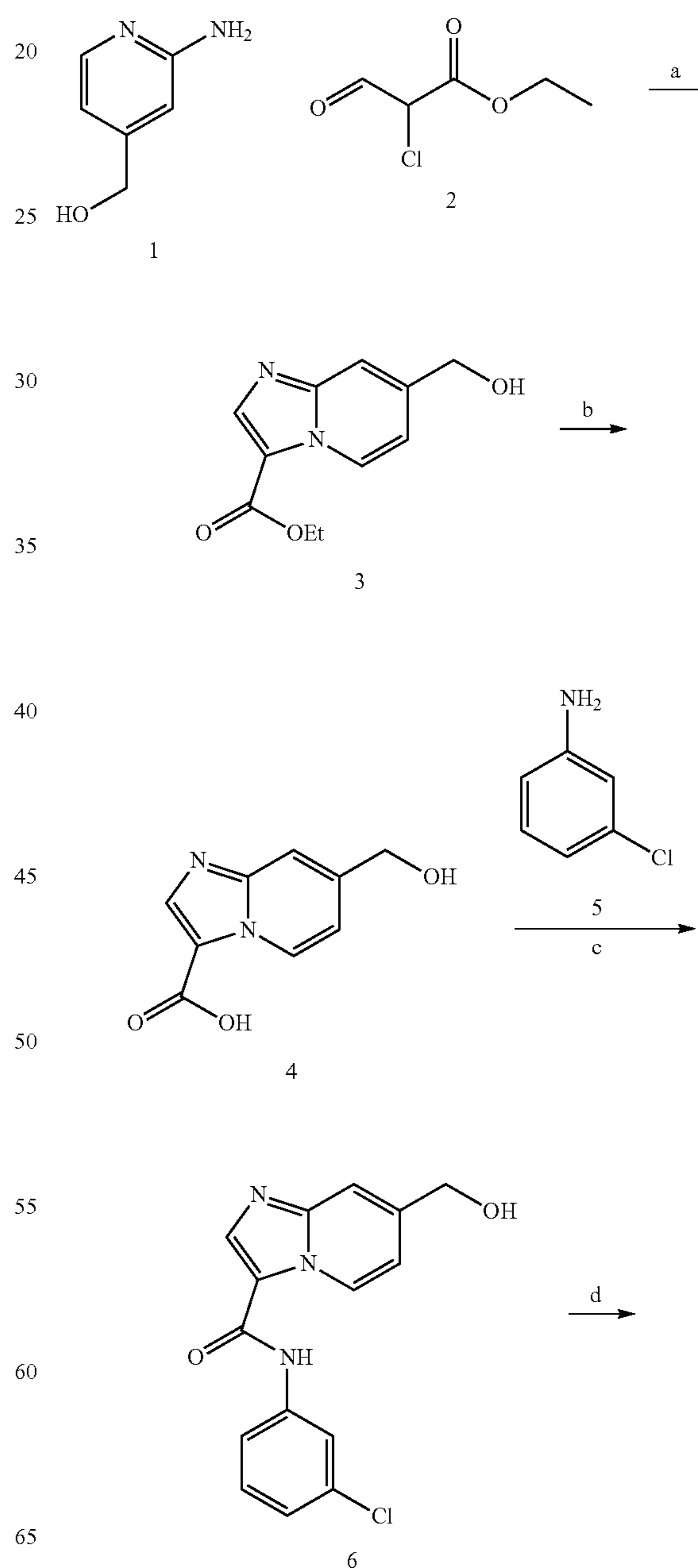
Scheme 1. Synthesis of Series I compounds 9a-d.
