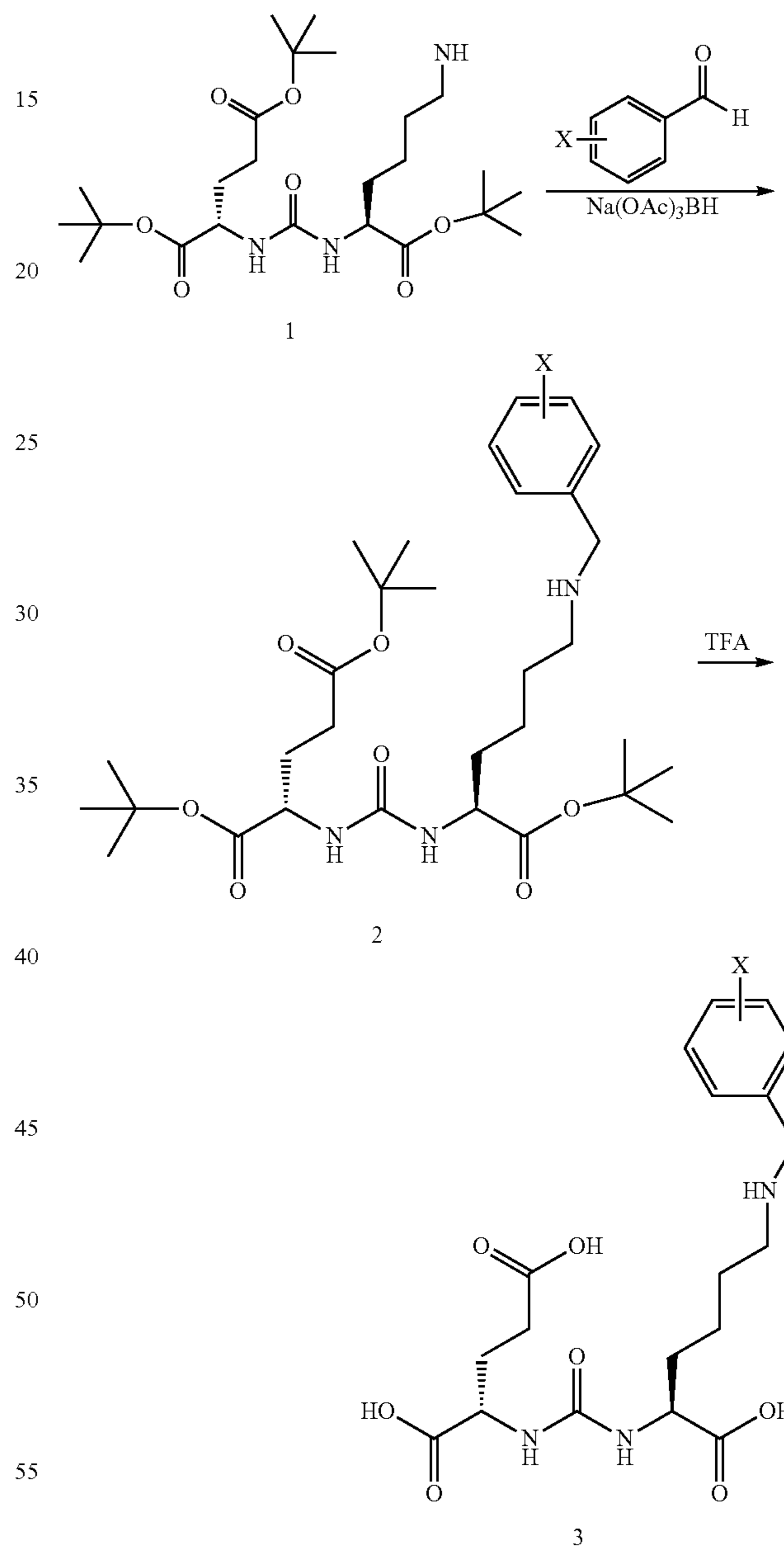
Scheme A. General pathway for the synthesis of halogenated Glu-Urea-Lys(N-benzyl-X) analogs (3).
