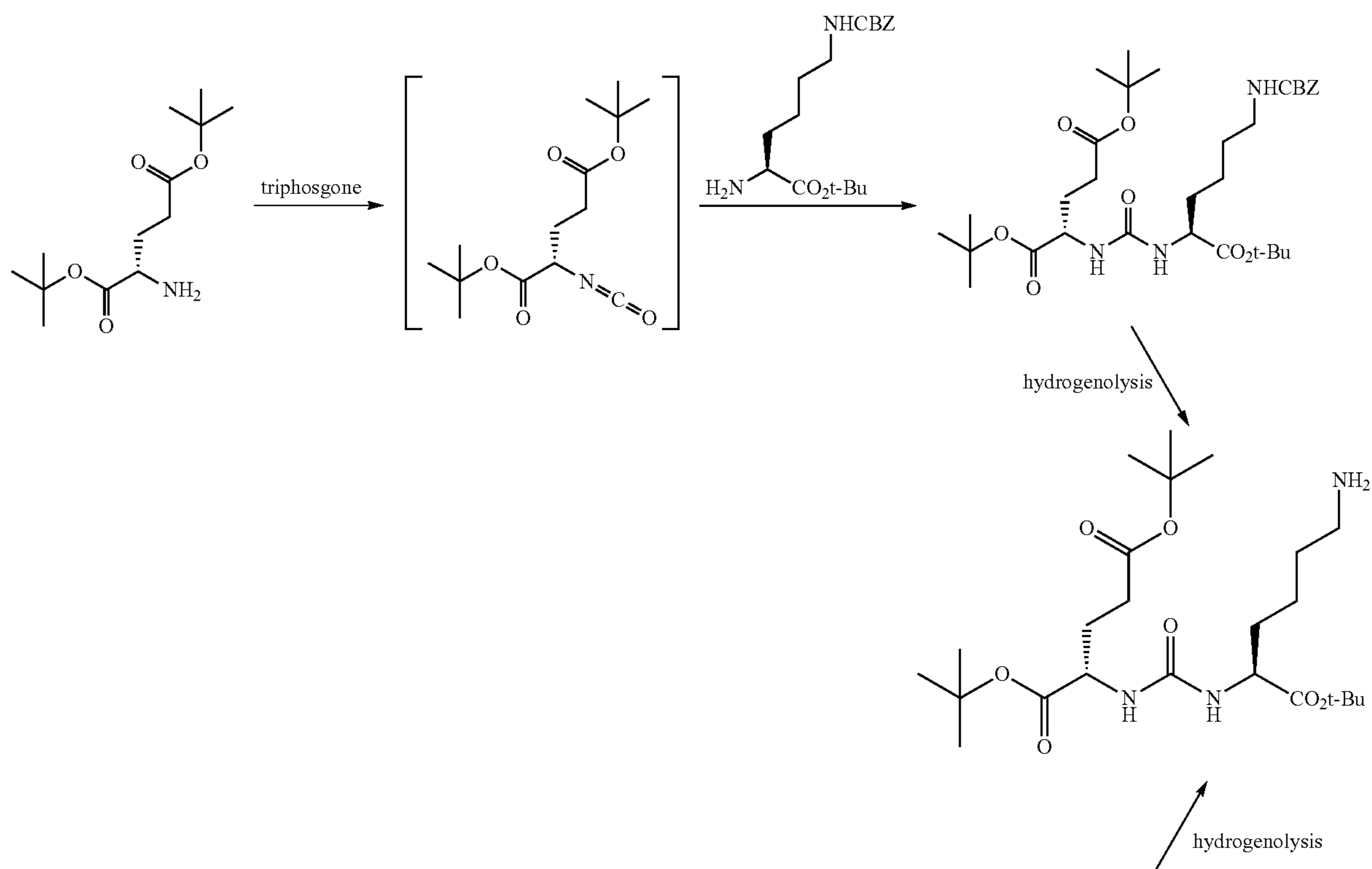
Scheme 2.
