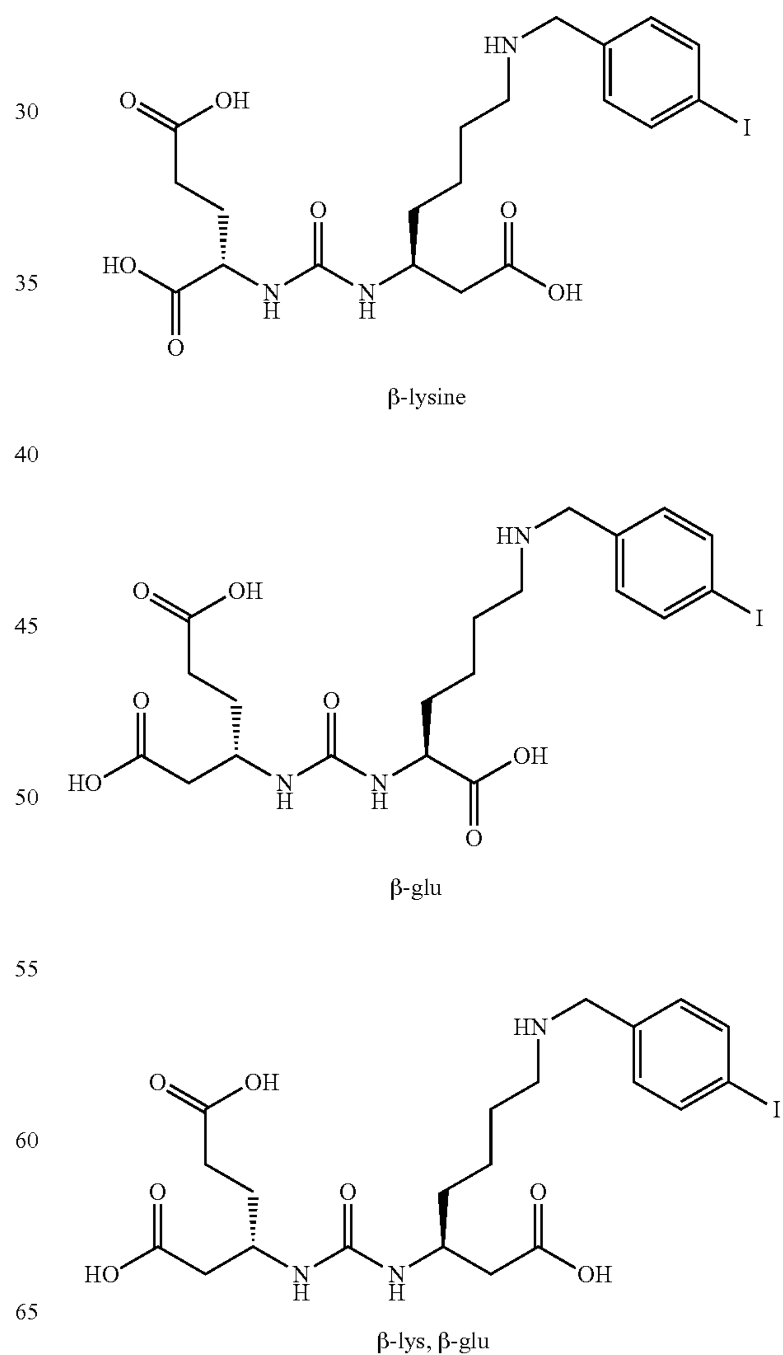
MIP-1072 β-amino acid analogs
