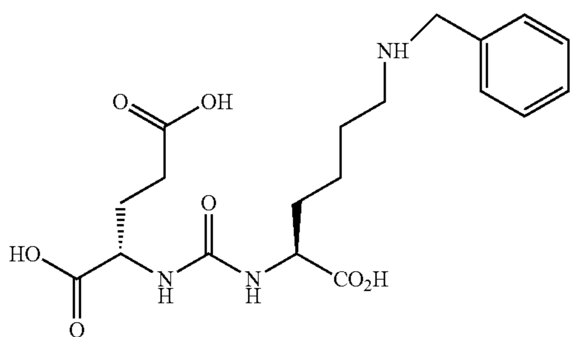
2-(3-{1-Carboxy-5-[3-(phenyl)-ureido]-pentyl}-ureido)-pentanedioic acid (11) (MIP 1111)
