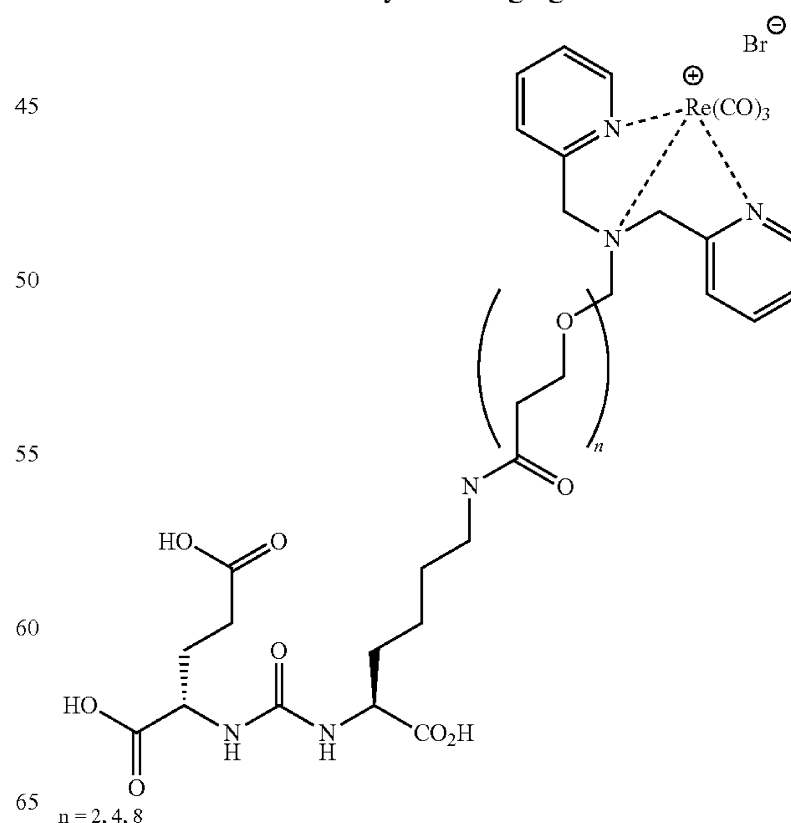
(19S,23S)-2-(4-iodobenzyl)-1-(4-iodophenyl)-13,21-dioxo-2,14,20,22-tetraazapentacosane-19,23,25-tricarboxylic acid (16) (MIP-1130)
