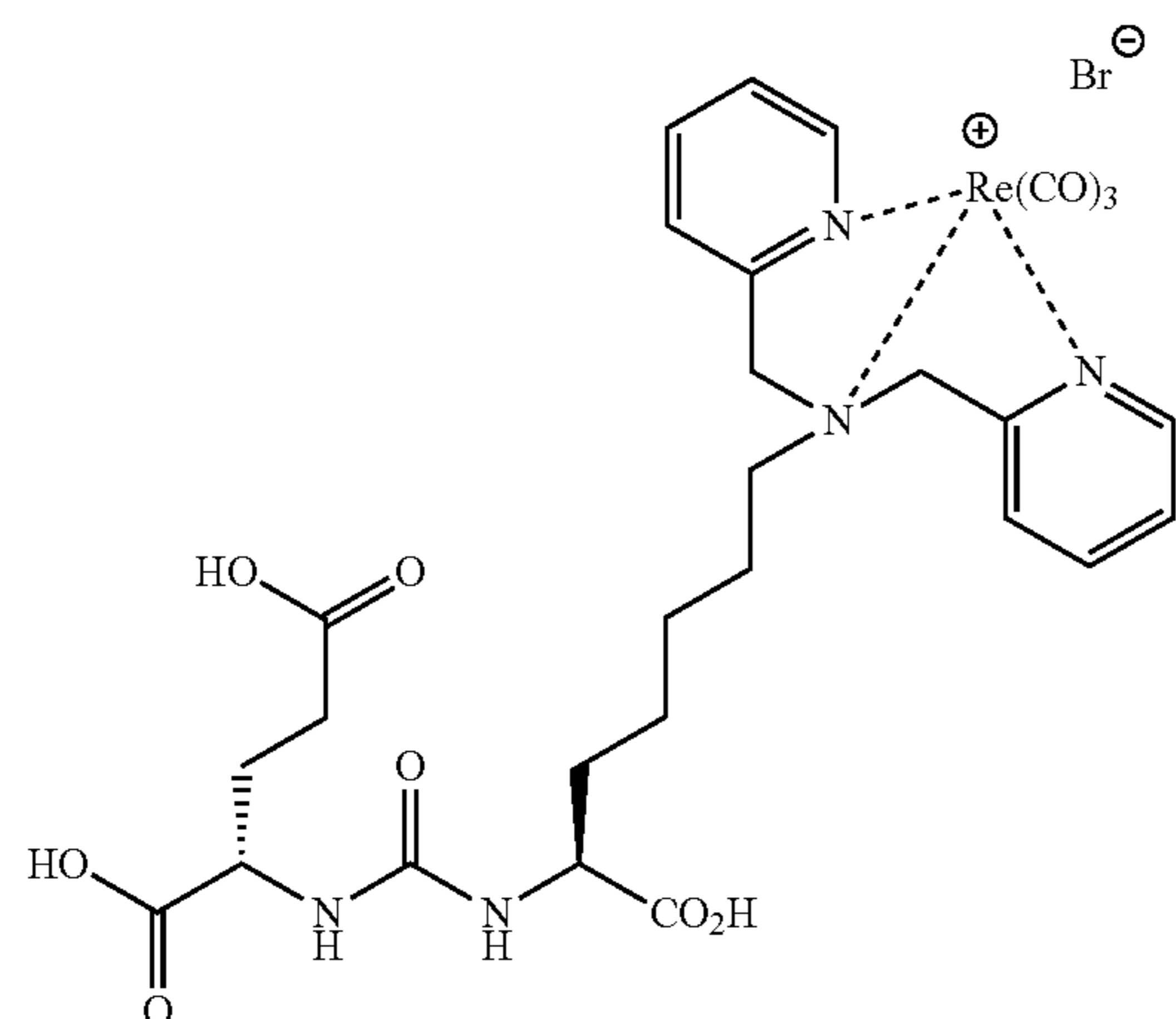
2-{3-[1-Carboxy-5-(carboxymethyl-pyridin-2-ylmethyl-amino)-pentyl]-ureido}-pentanedioic acid (26)
