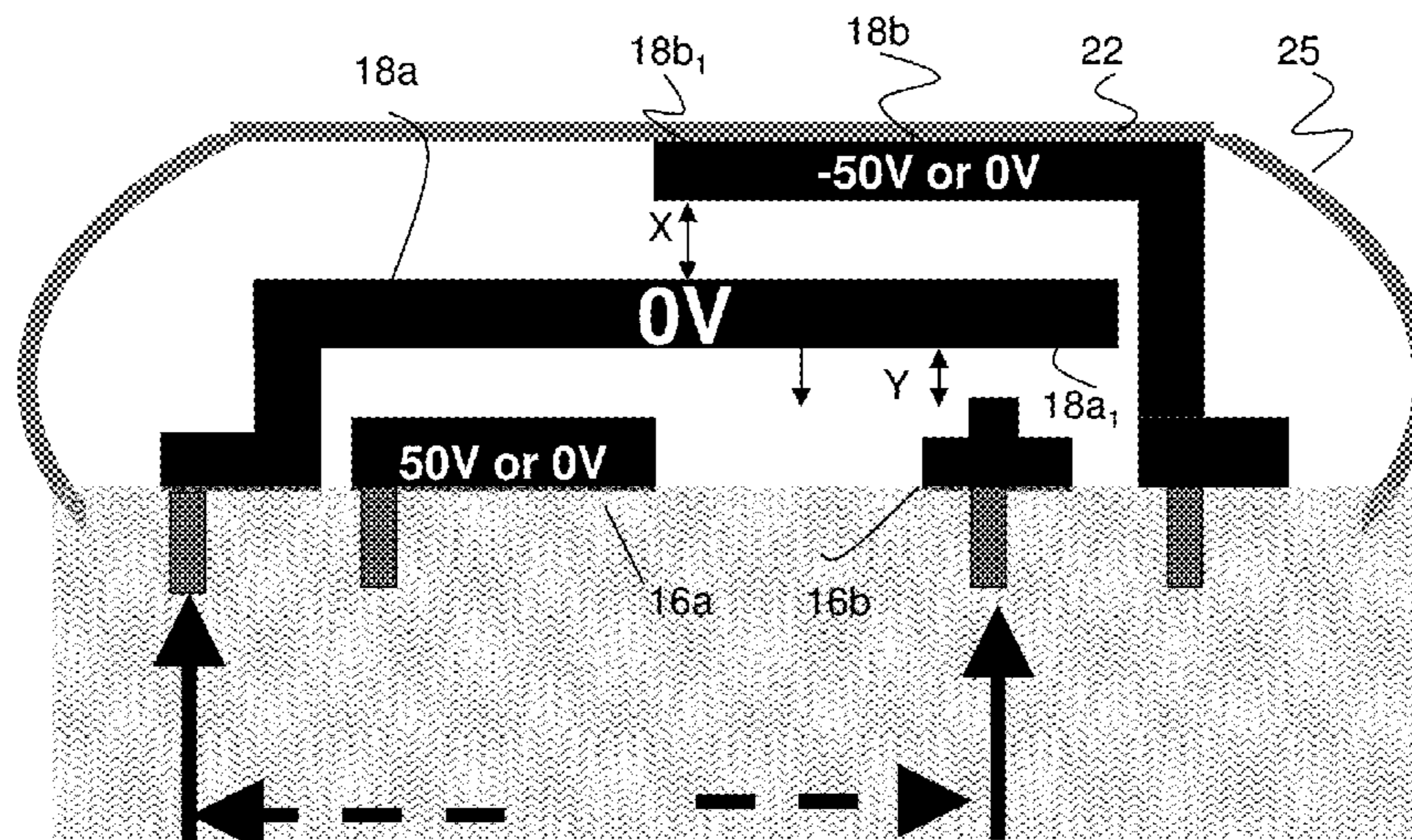
Sense open or closed switch
