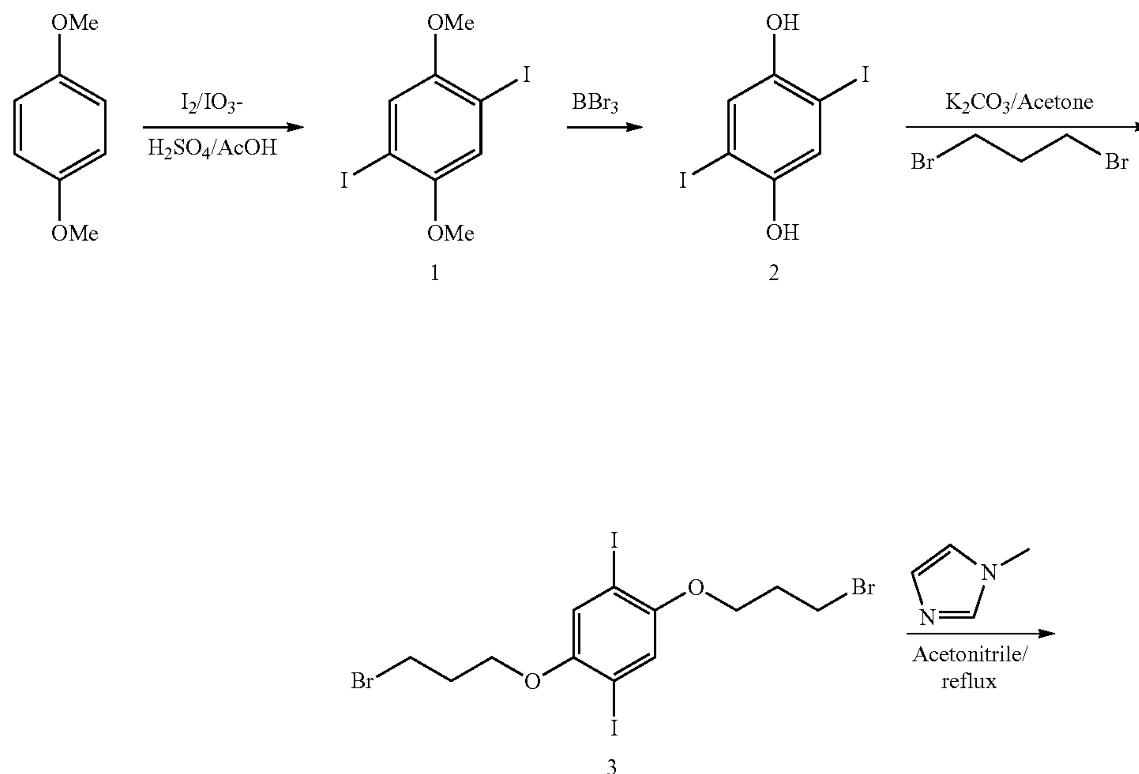
Scheme 1.
