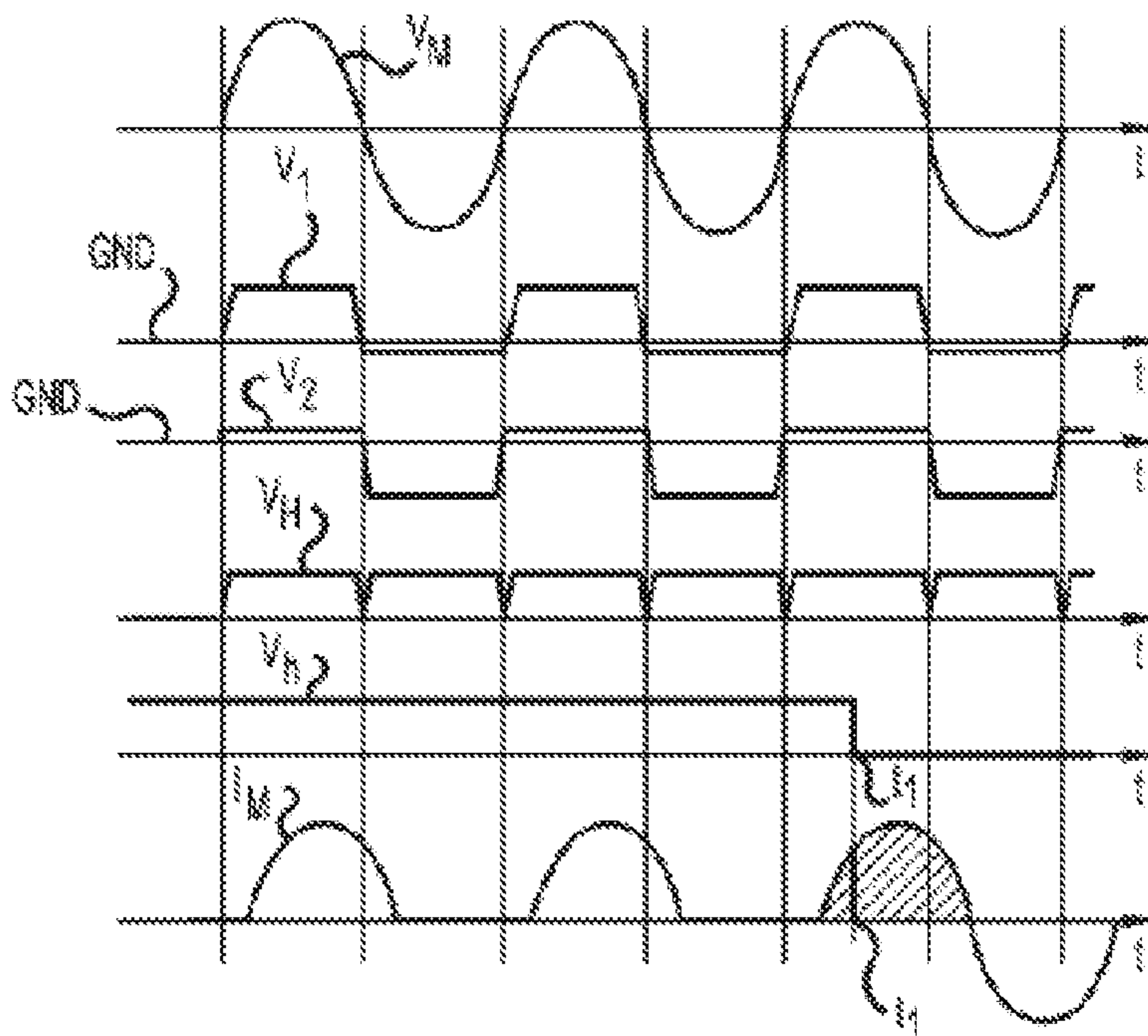
FIG. 2 (PRIOR ART)
