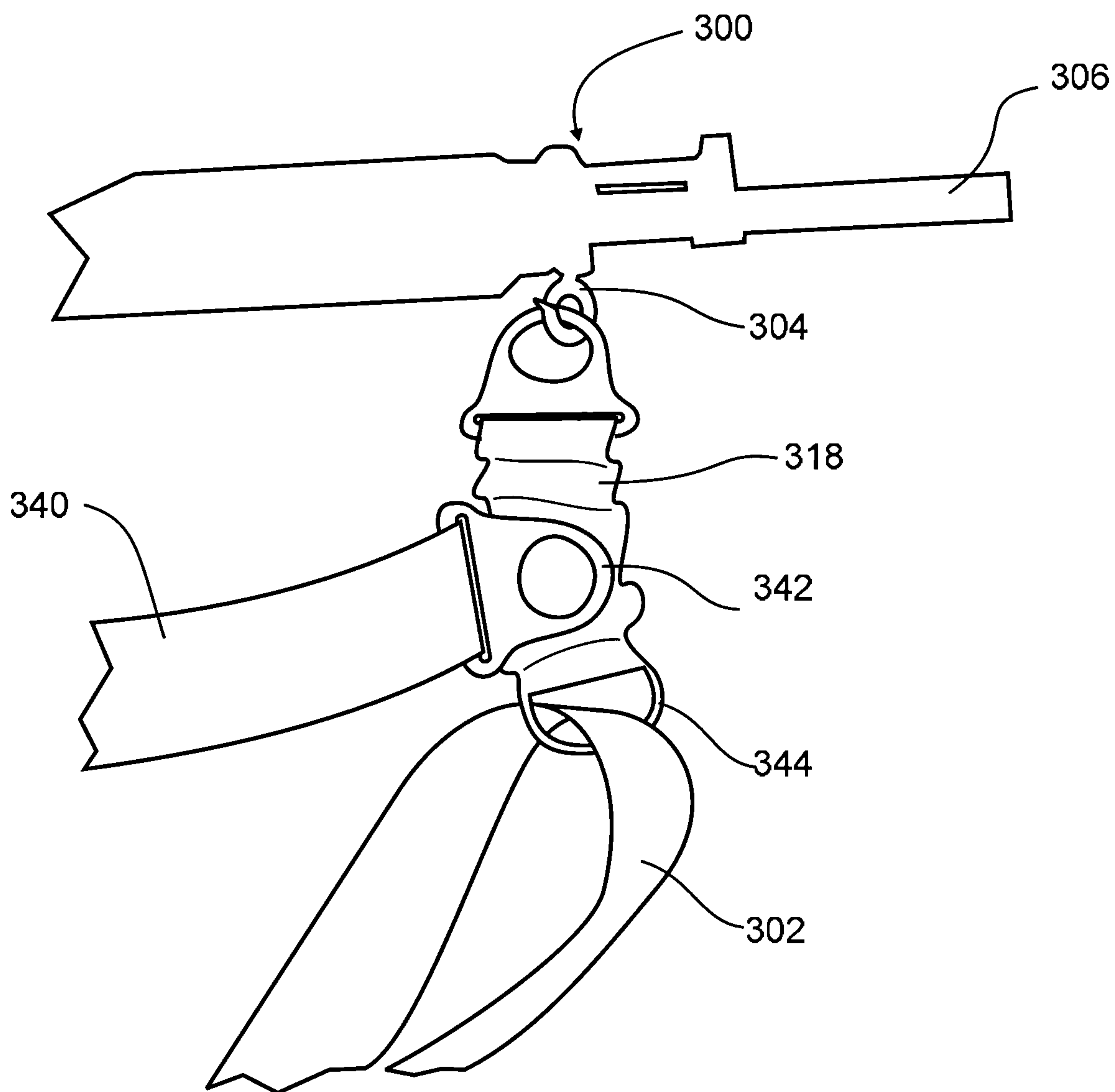
Fig. 20 (Prior Art)
