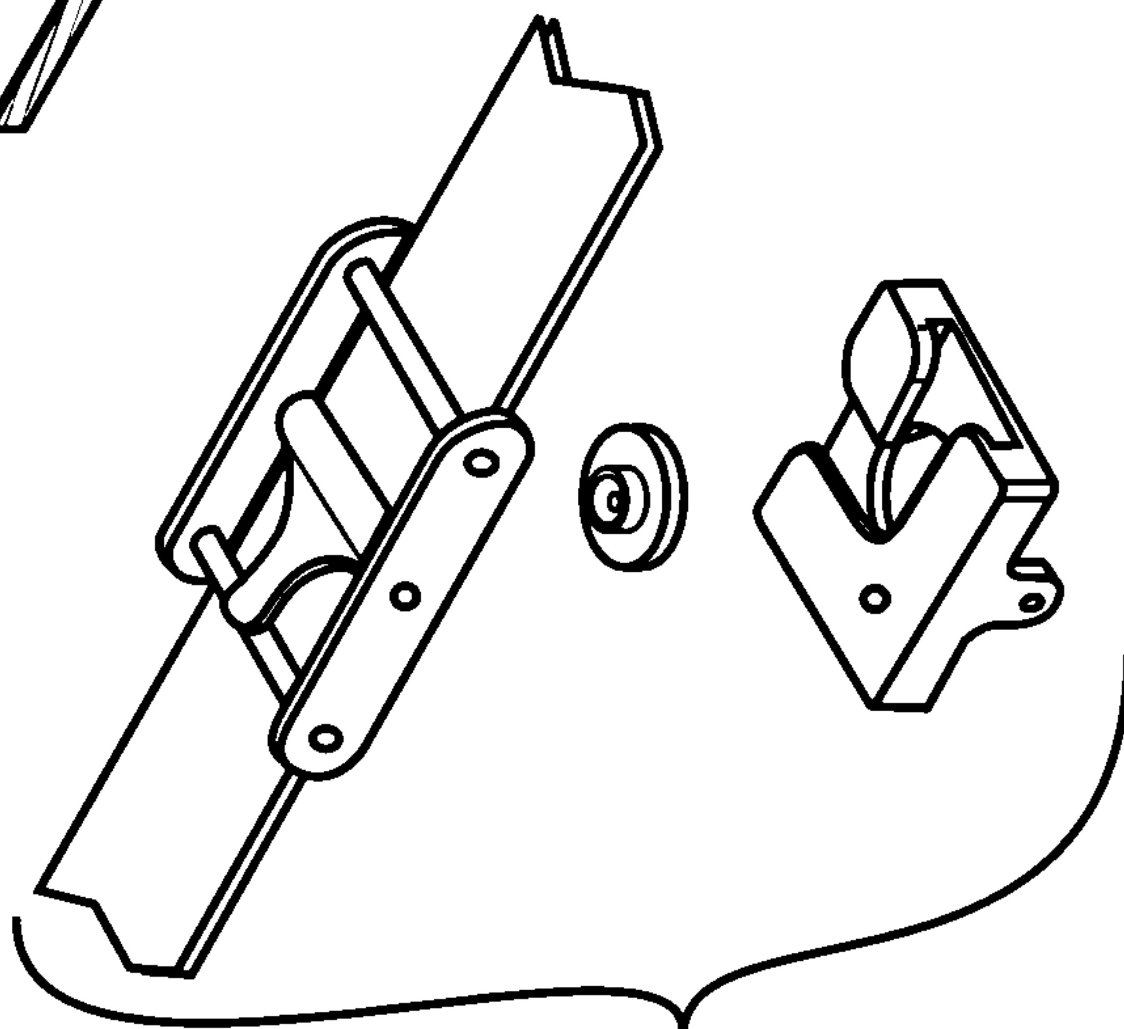
FIG. 33 (Prior Art)
