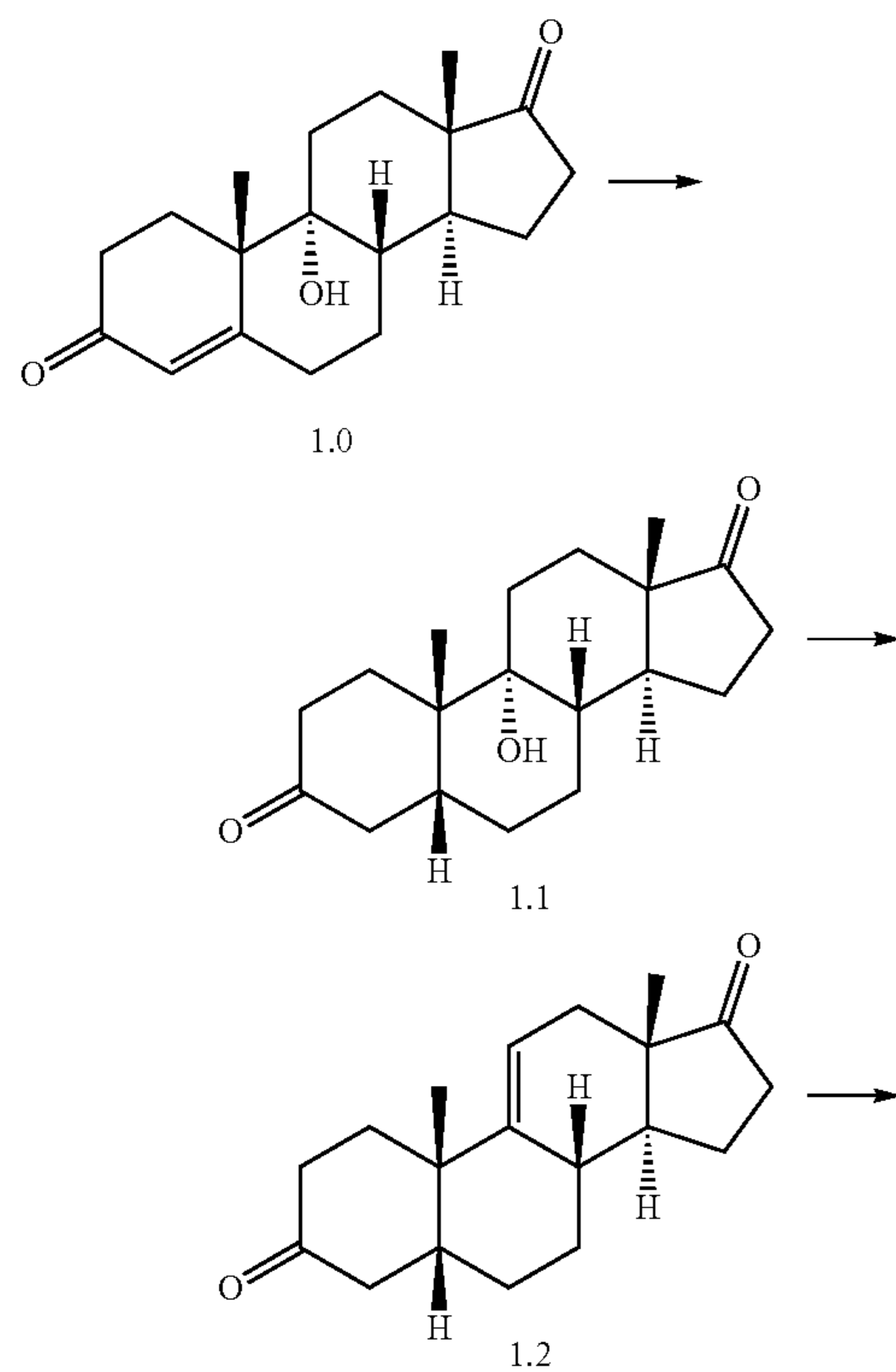
Scheme 1. Synthesis of Deoxycholic Acid (DCA)
