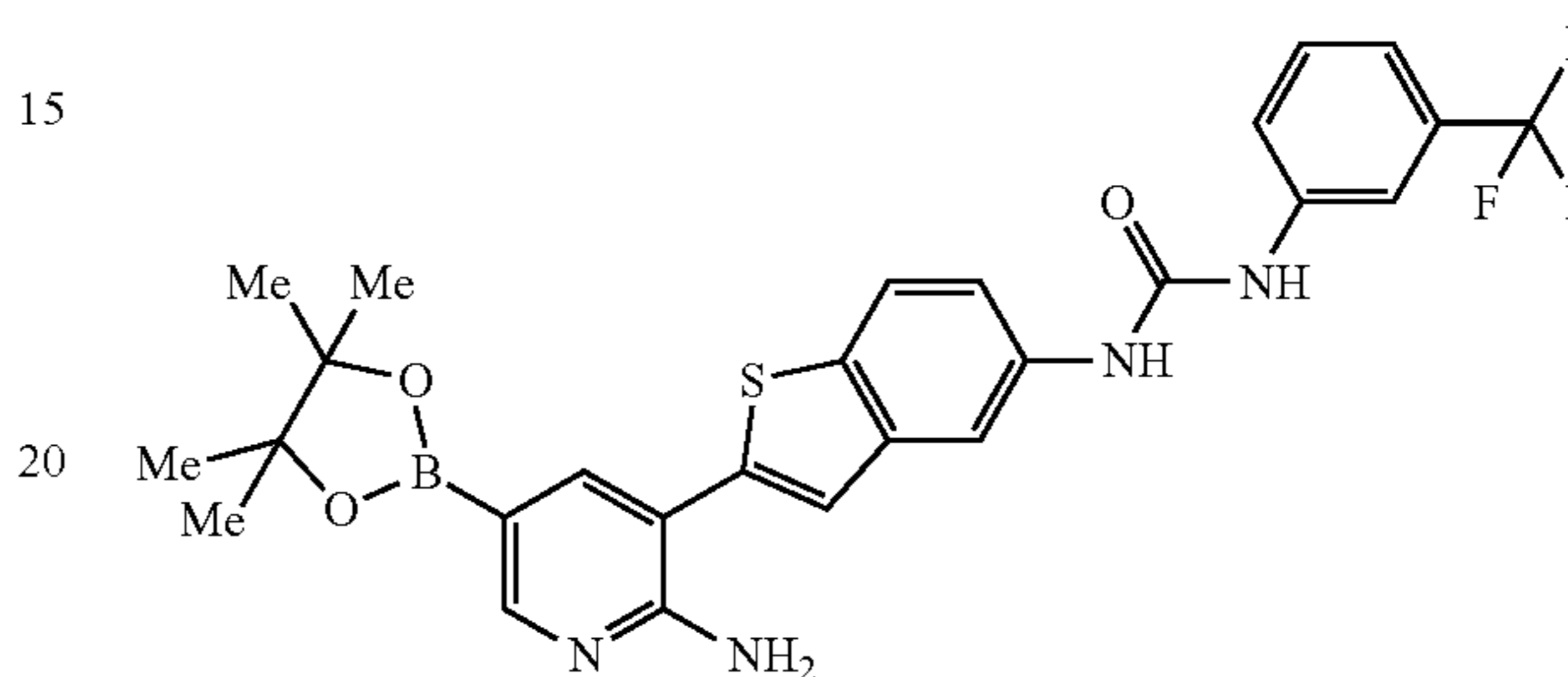
1-{2-[2-amino-5-(4,4,5,5-tetramethyl-1,3,2-dioxaborolan-2-yl)pyridin-3-yl]-1-benzothien-5-yl}-3-[3-(trifluoromethyl)phenyl]urea
