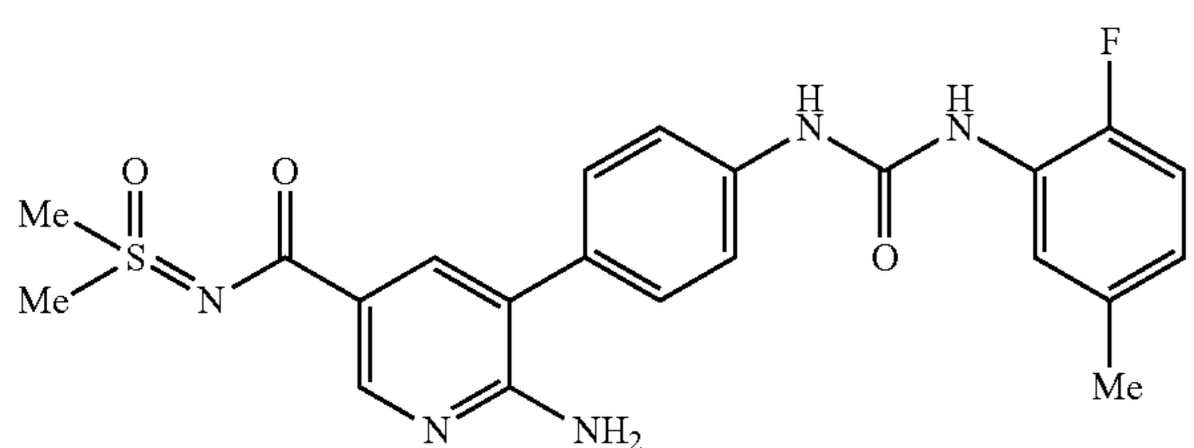
6-amino-N-[dimethyl(oxido)- \lambda^4 -sulfanylidene]-5-[4-((2-fluoro-5-methylphenyl)amino)carbonylamino]phenyl]nicotinamide
