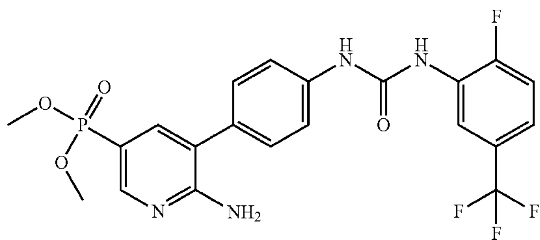
dimethyl {6-amino-5-[4-({[2-fluoro-5-(trifluoromethyl)phenyl]carbamoyl}amino)phenyl]pyridin-3-yl}phosphonate
