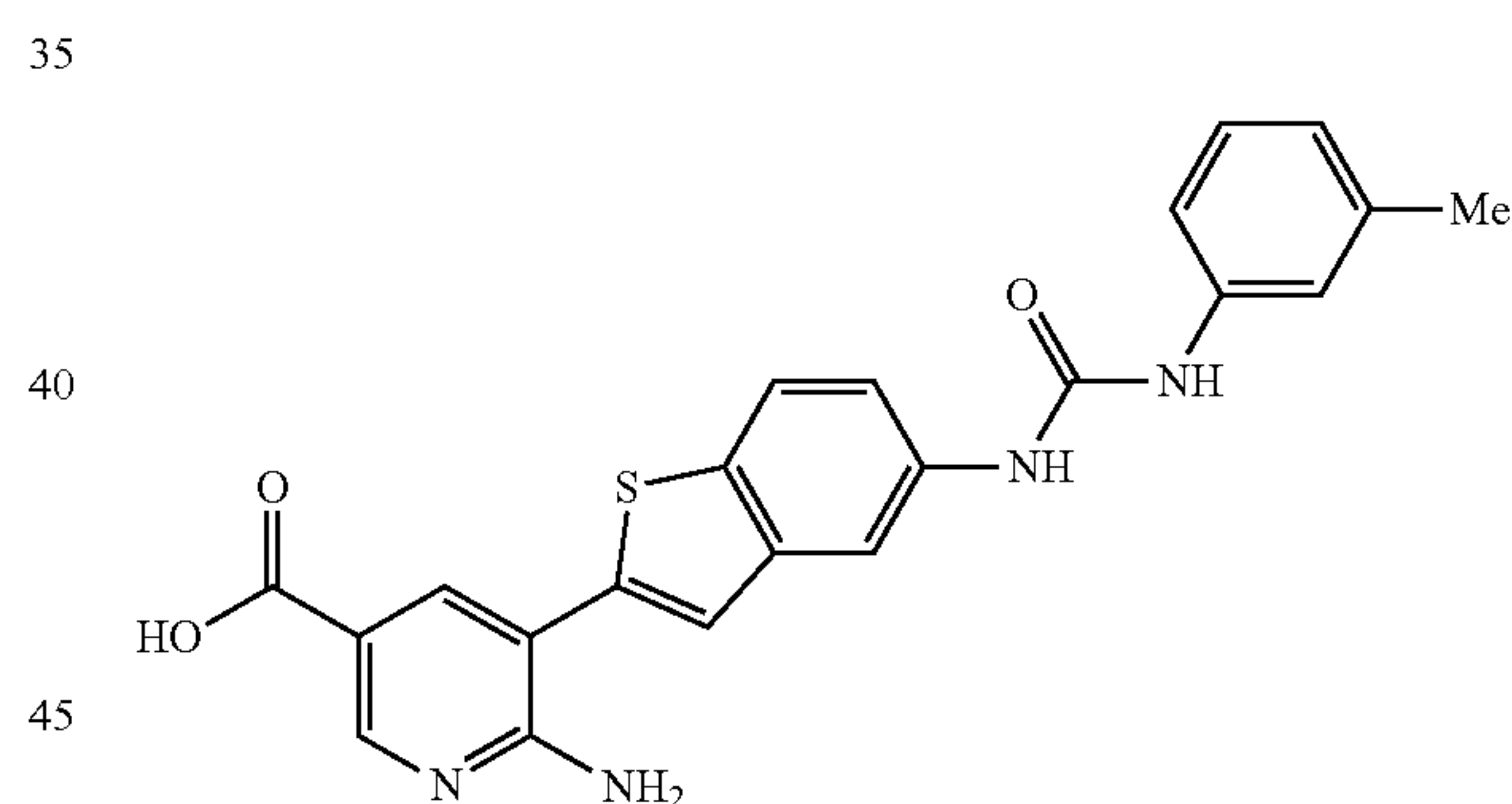
6-amino-5-[5-((3-methylphenyl)amino)carbonyl]amino-1-benzothien-2-yl]nicotinic acid
