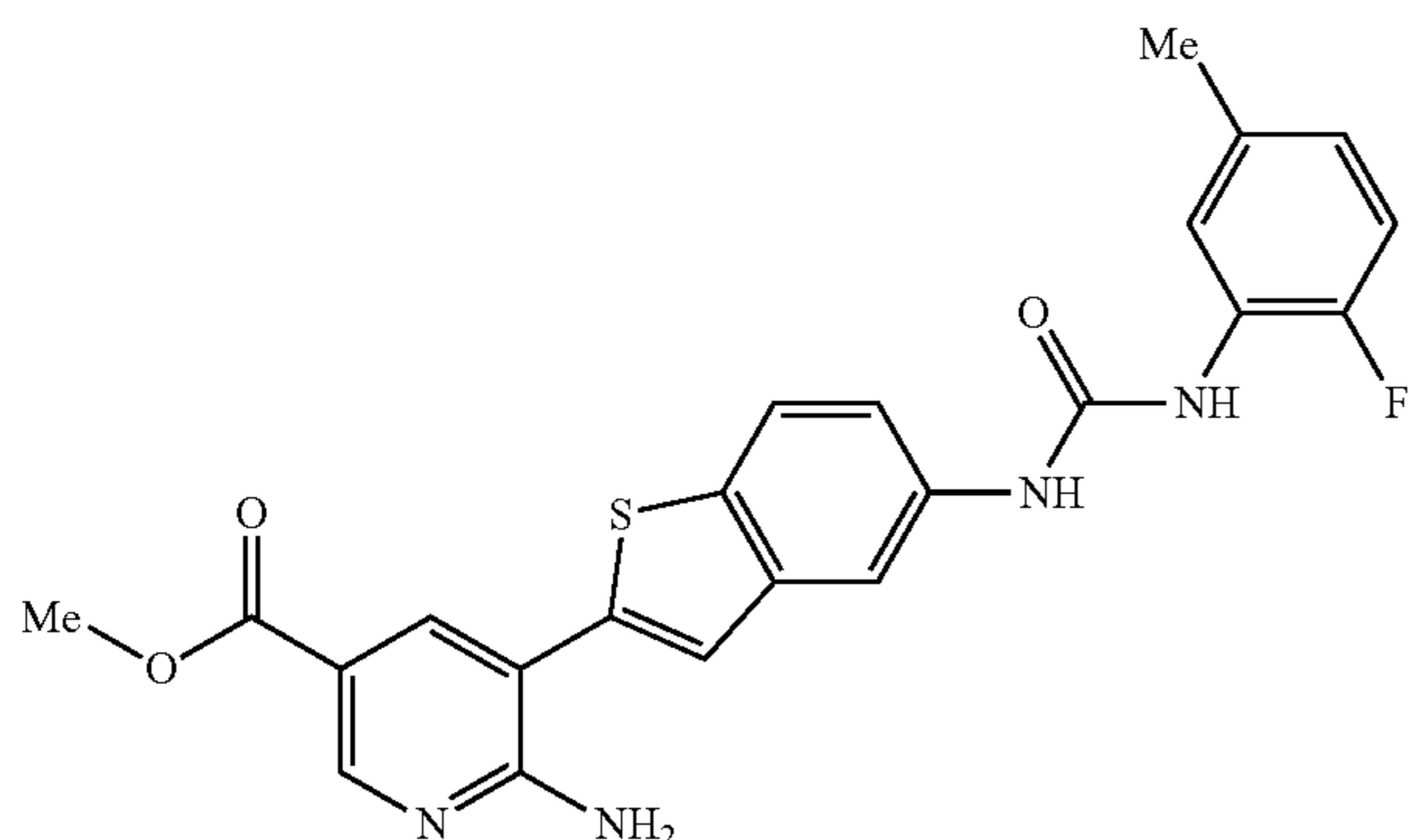
methyl 6-amino-5-[5-((2-fluoro-5-methylphenyl)amino)carbonyl]amino-1-benzothien-2-yl]nicotinate
