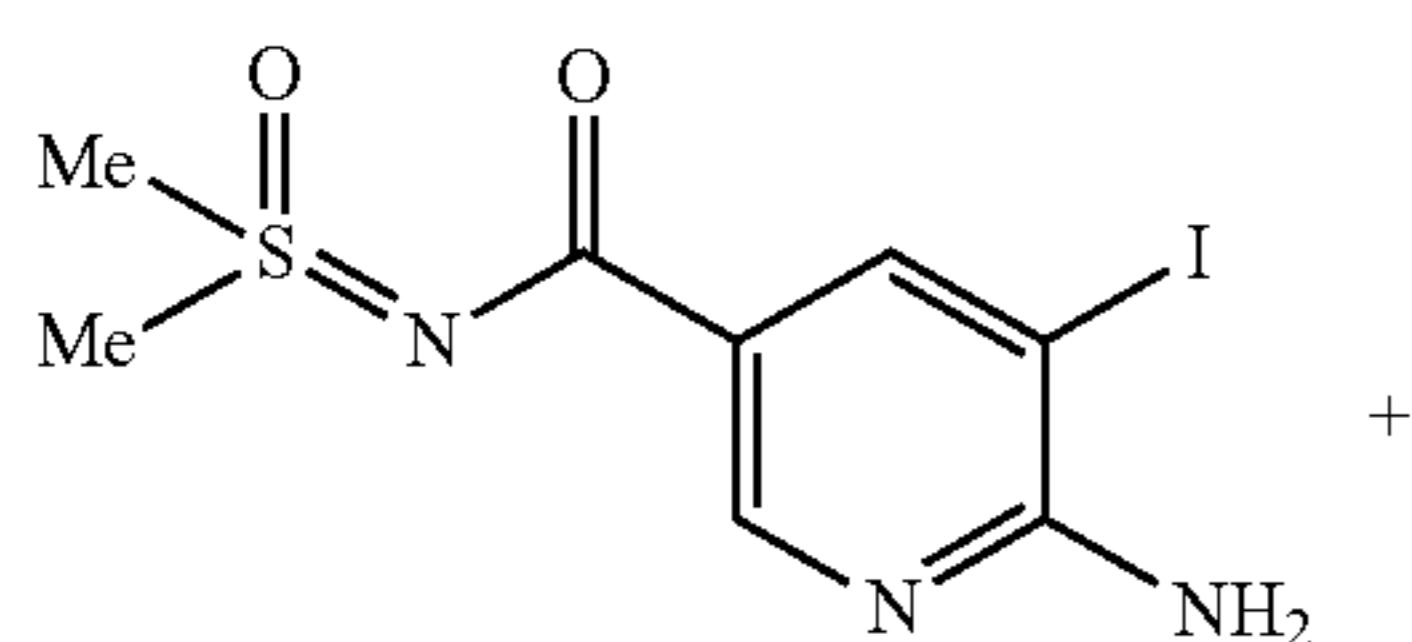
Scheme 1
