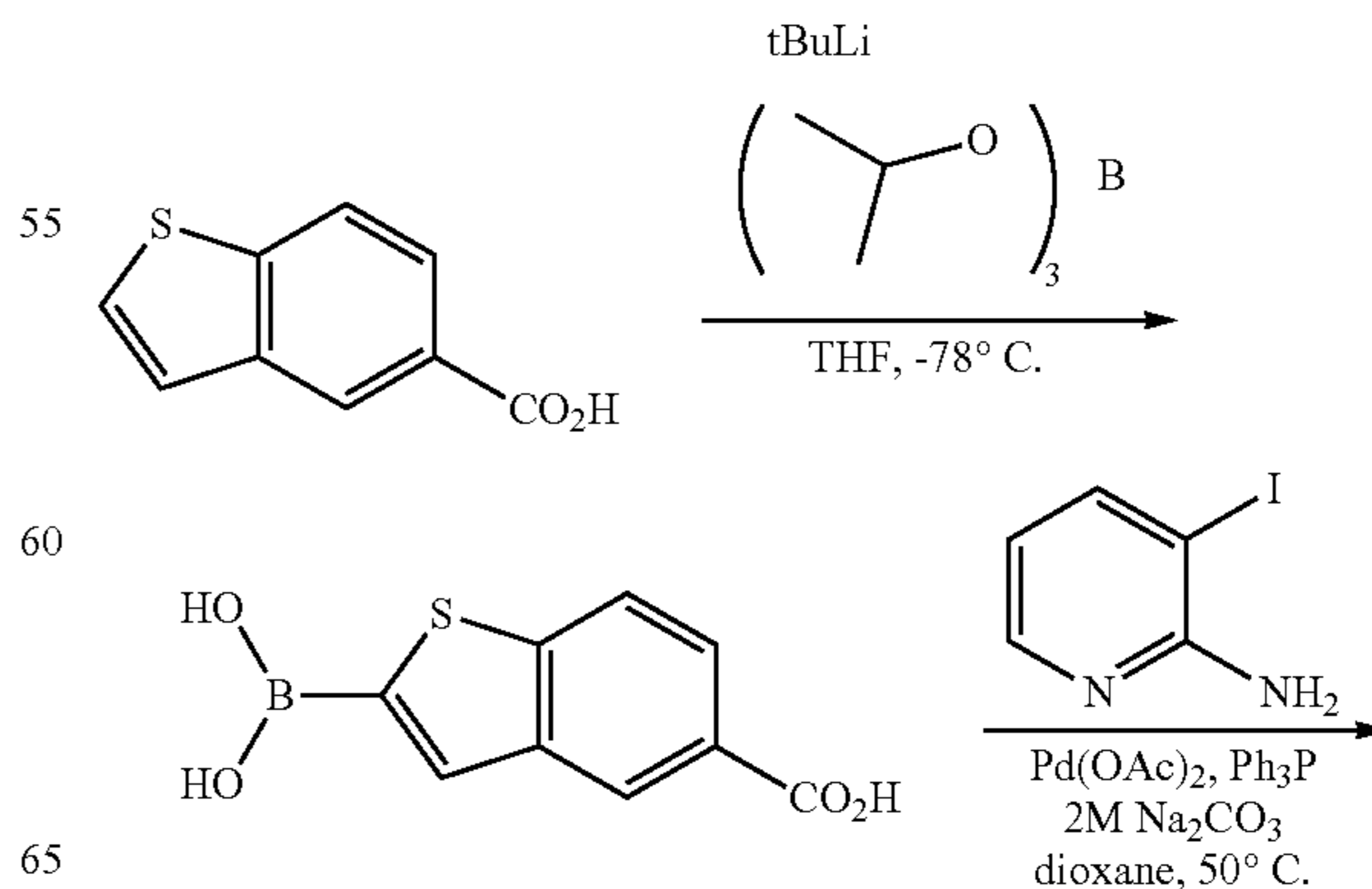
Scheme 8
