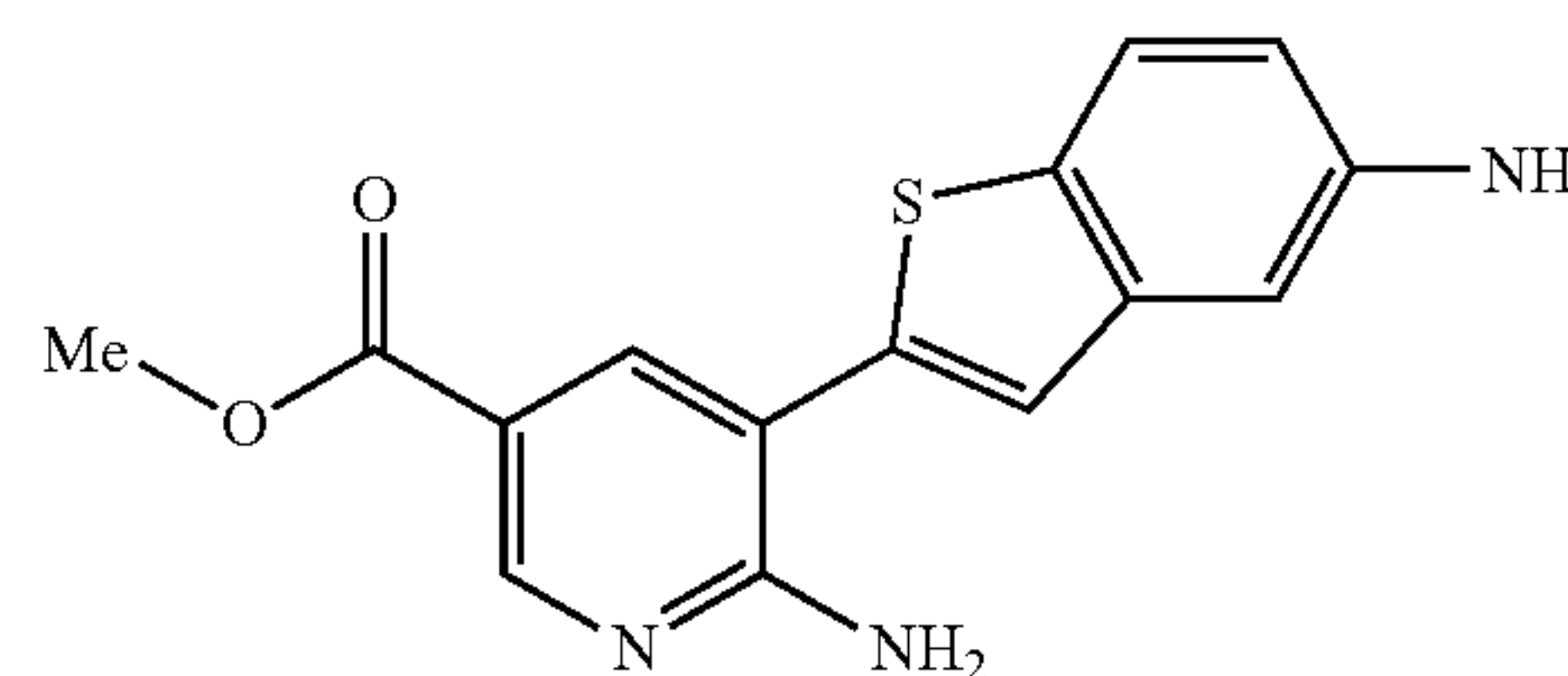
methyl 6-amino-5-(5-amino-1-benzothien-2-yl)nicotinate
