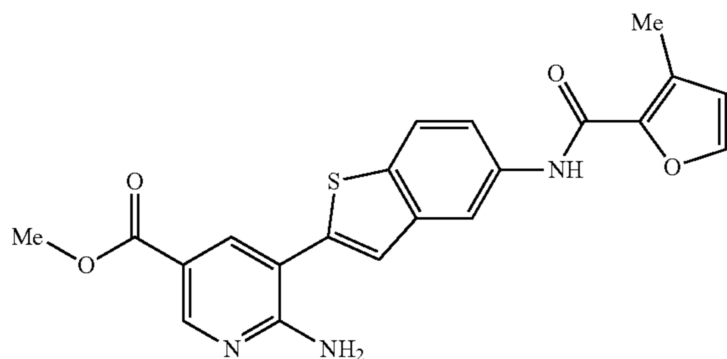
methyl 6-amino-5-{5-[(3-methyl-2-furoyl)amino]-1-benzothien-2-yl}nicotinate
