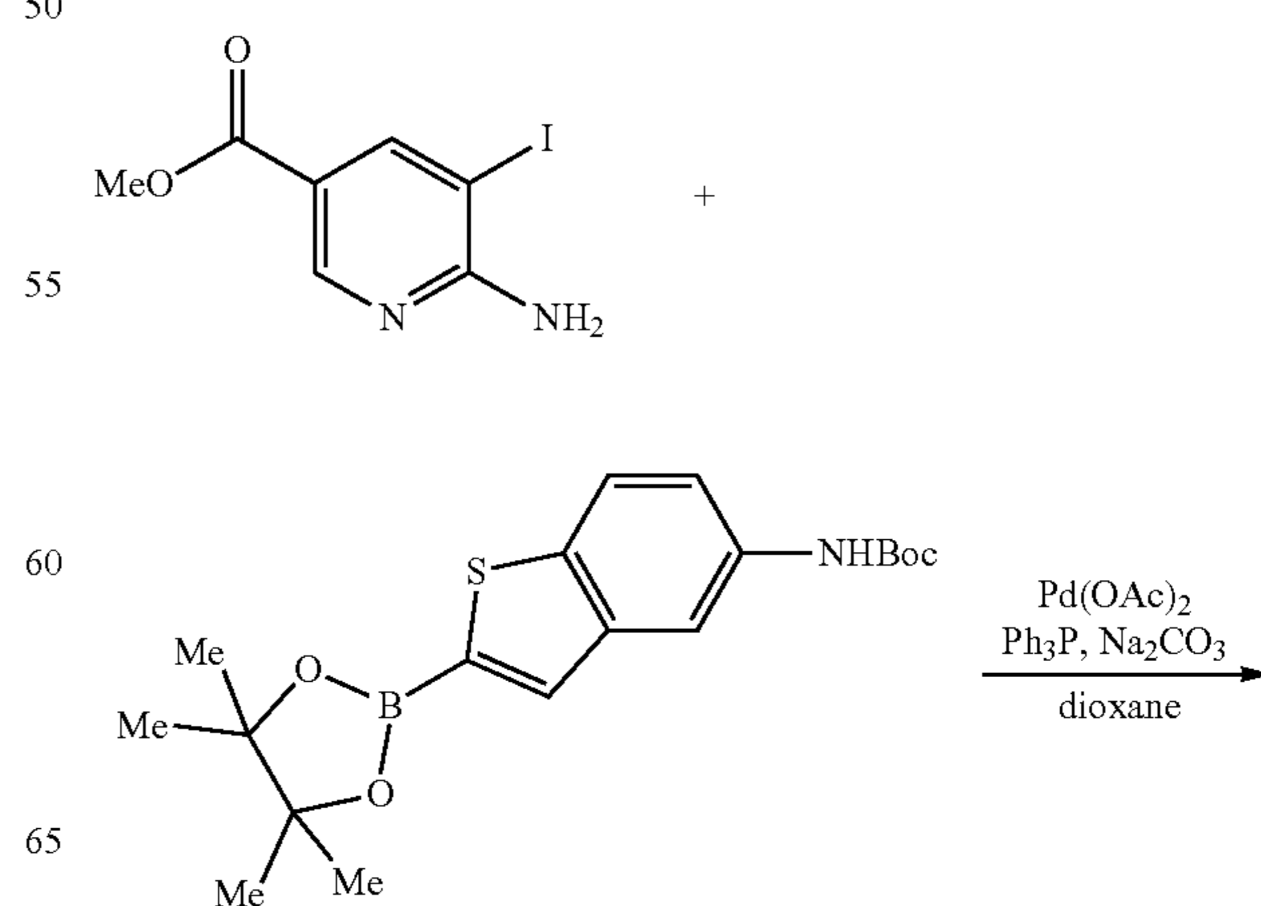
Scheme 2
