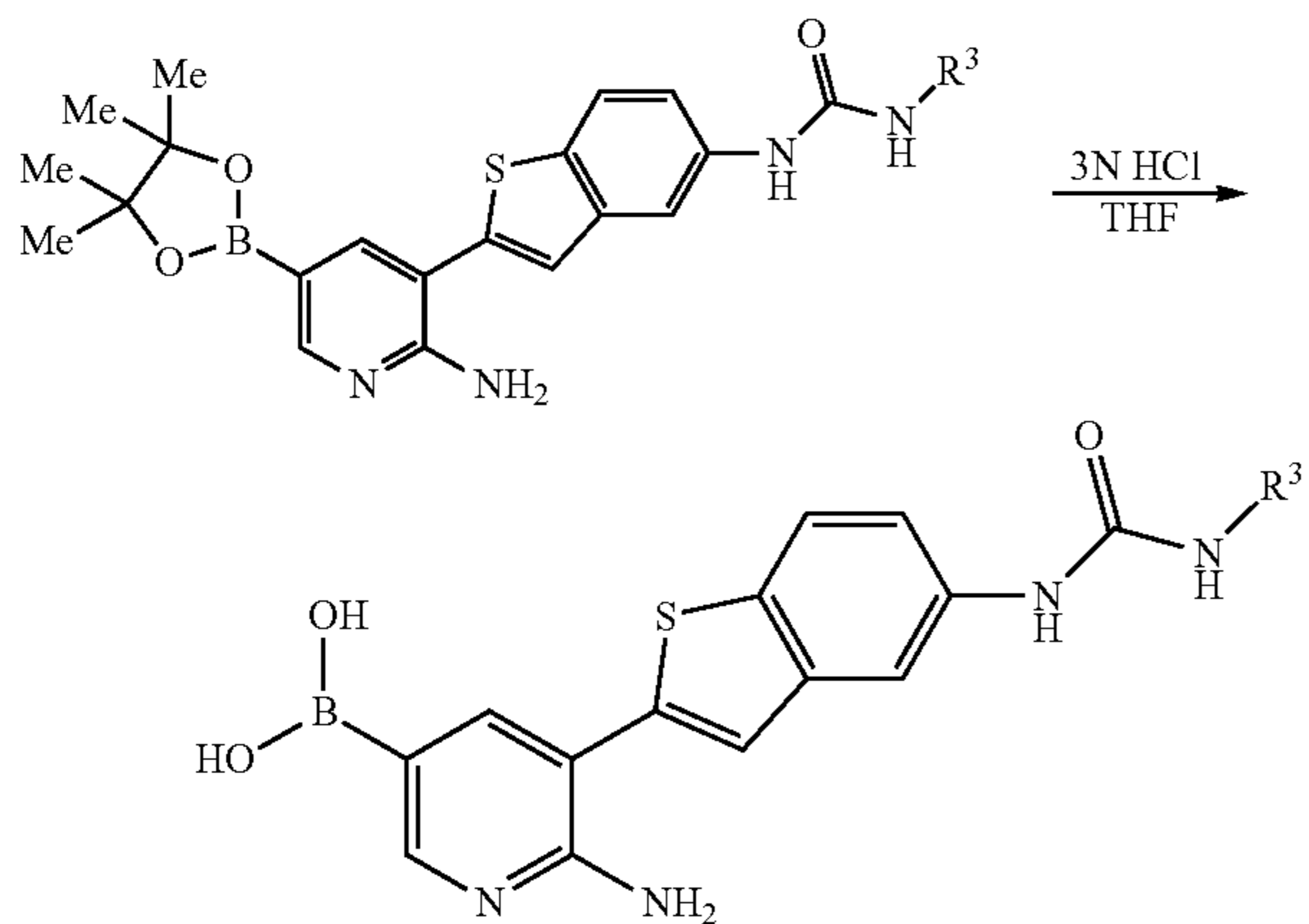
Scheme 5
