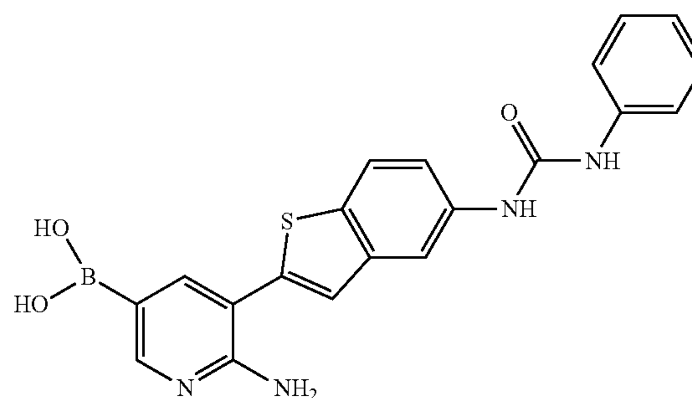
(6-amino-5-[5-((anilino)carbonyl)amino]-1-benzothien-2-yl]pyridin-3-yl)boronic acid
