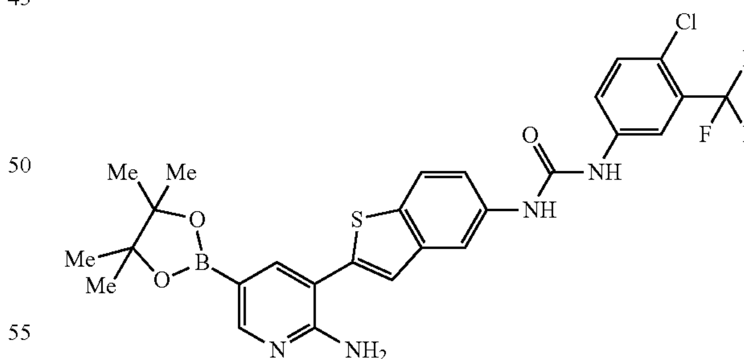
1-{2-[2-amino-5-(4,4,5,5-tetramethyl-1,3,2-dioxaborolan-2-yl)pyridin-3-yl]-1-benzothien-5-yl}-3-[4-chloro-3-(trifluoromethyl)phenyl]urea
