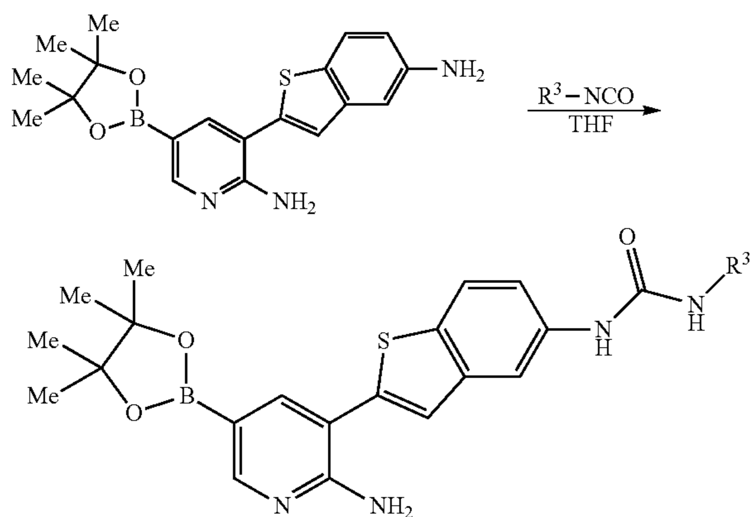
Scheme 4
