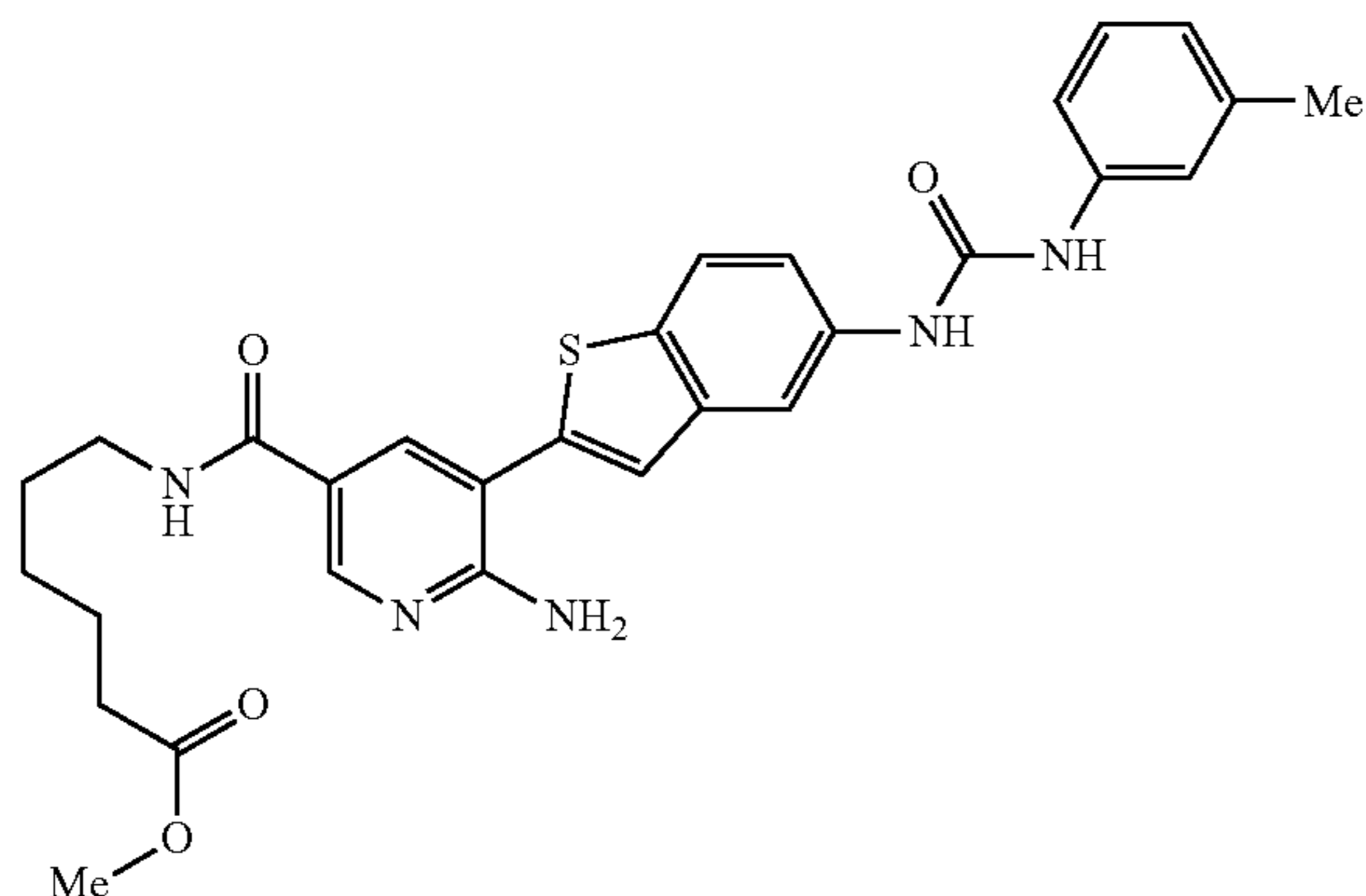
methyl 6-[(6-amino-5-[5-((3-methylphenyl)amino)carbonyl]amino)-1-benzothien-2-yl]pyridin-3-yl carbonyl amino hexanoate
