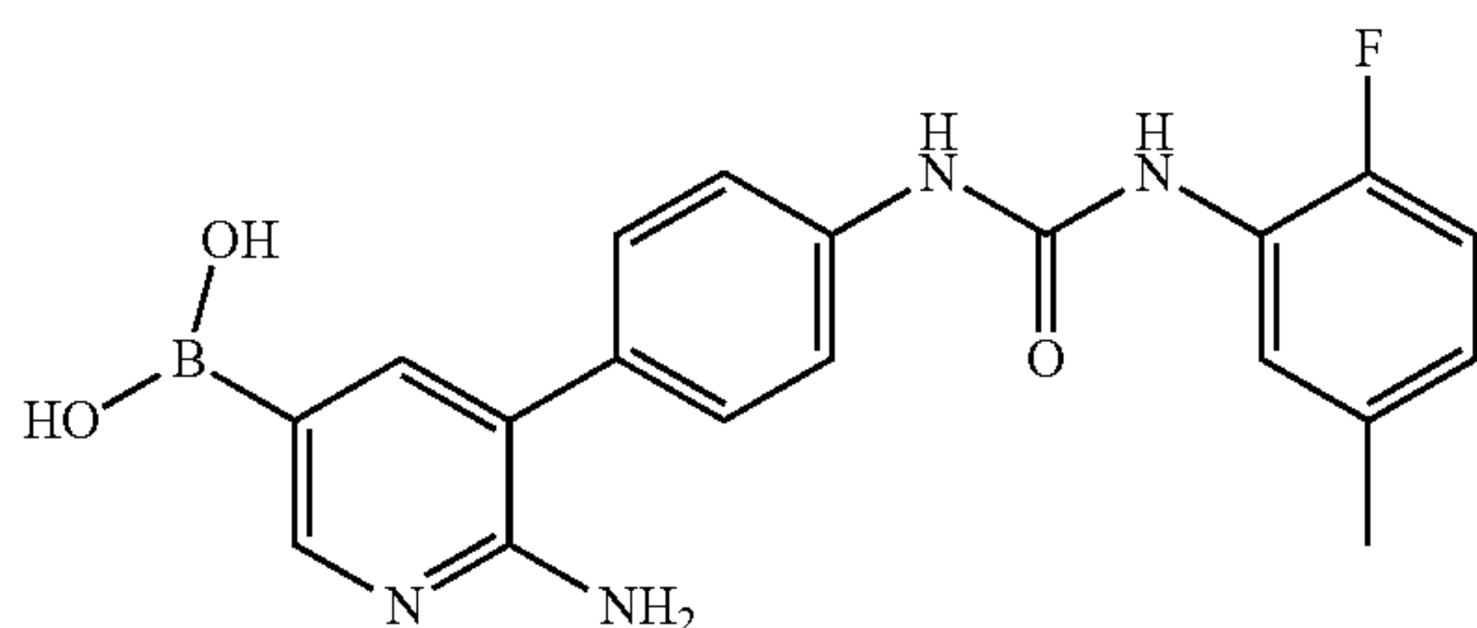
(6-amino-5-(4-(3-(2-fluoro-5-methylphenyl)ureido)phenyl)pyridin-3-yl)boronic acid
