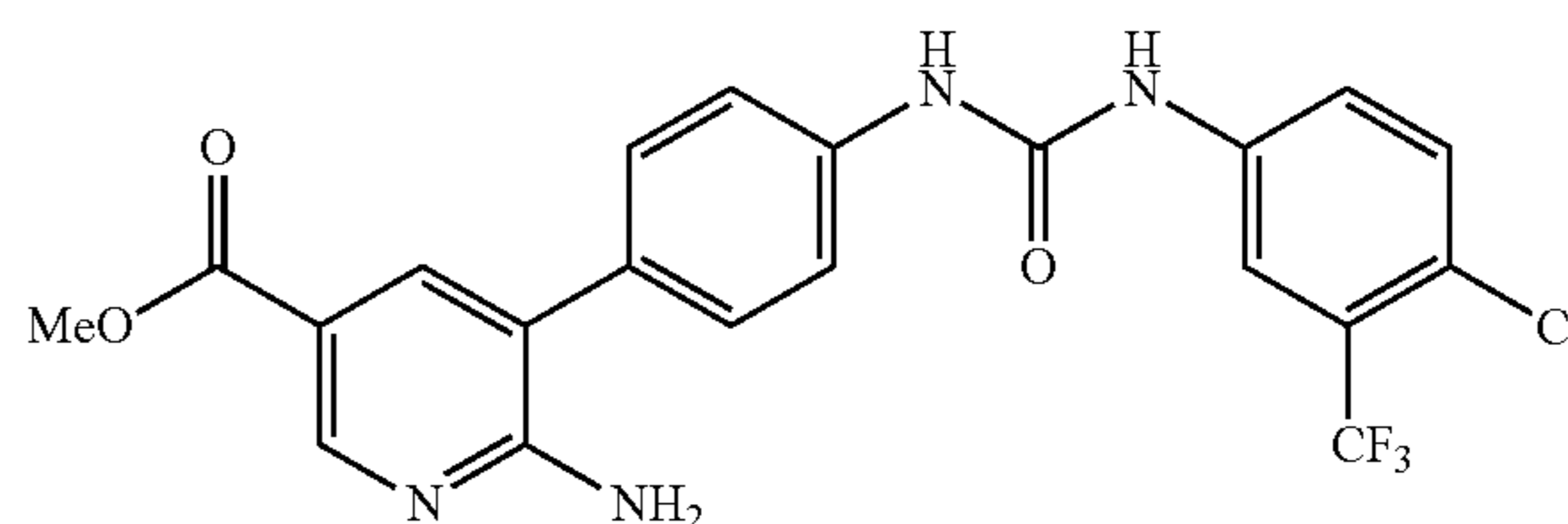
methyl 6-amino-5-[4-({(4-chloro-3-(trifluoromethyl)phenyl)carbonyl}amino)phenyl]pyridine-3-carboxylate
