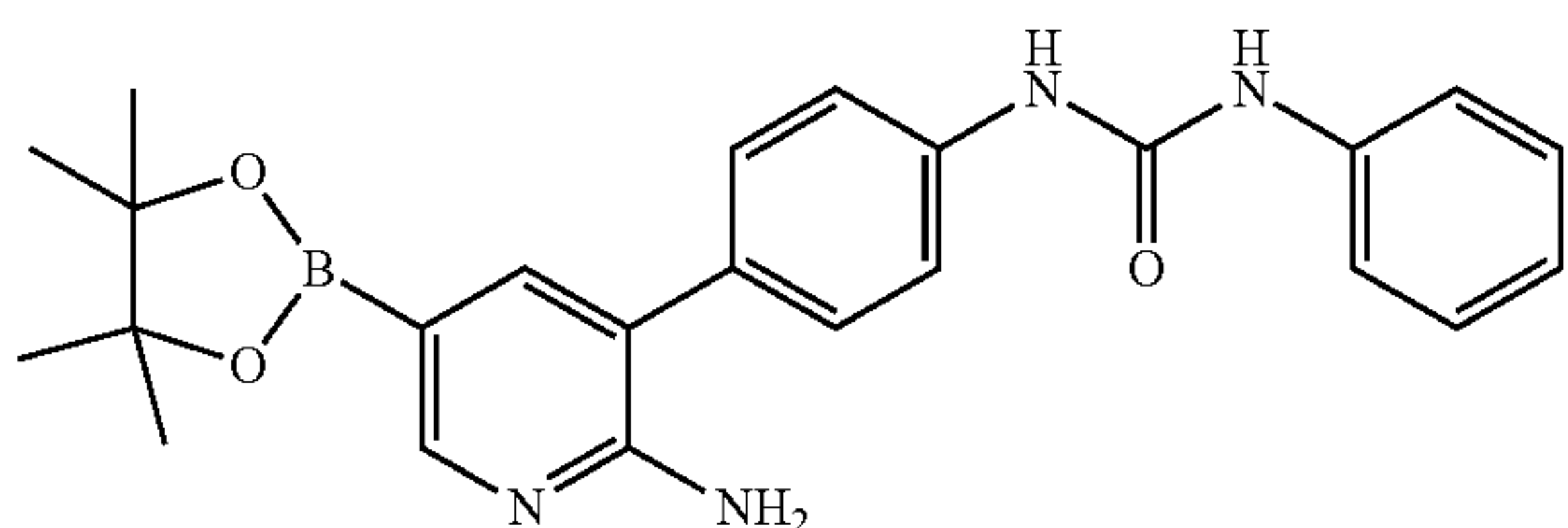
dimethyl 5,5'-(N-{{[6-amino-5-(4-{{[3-methylphenyl]carbamoyl}amino}phenyl)pyridin-3-yl]carbonyl}ulfonimidoyl}dipentanoate
