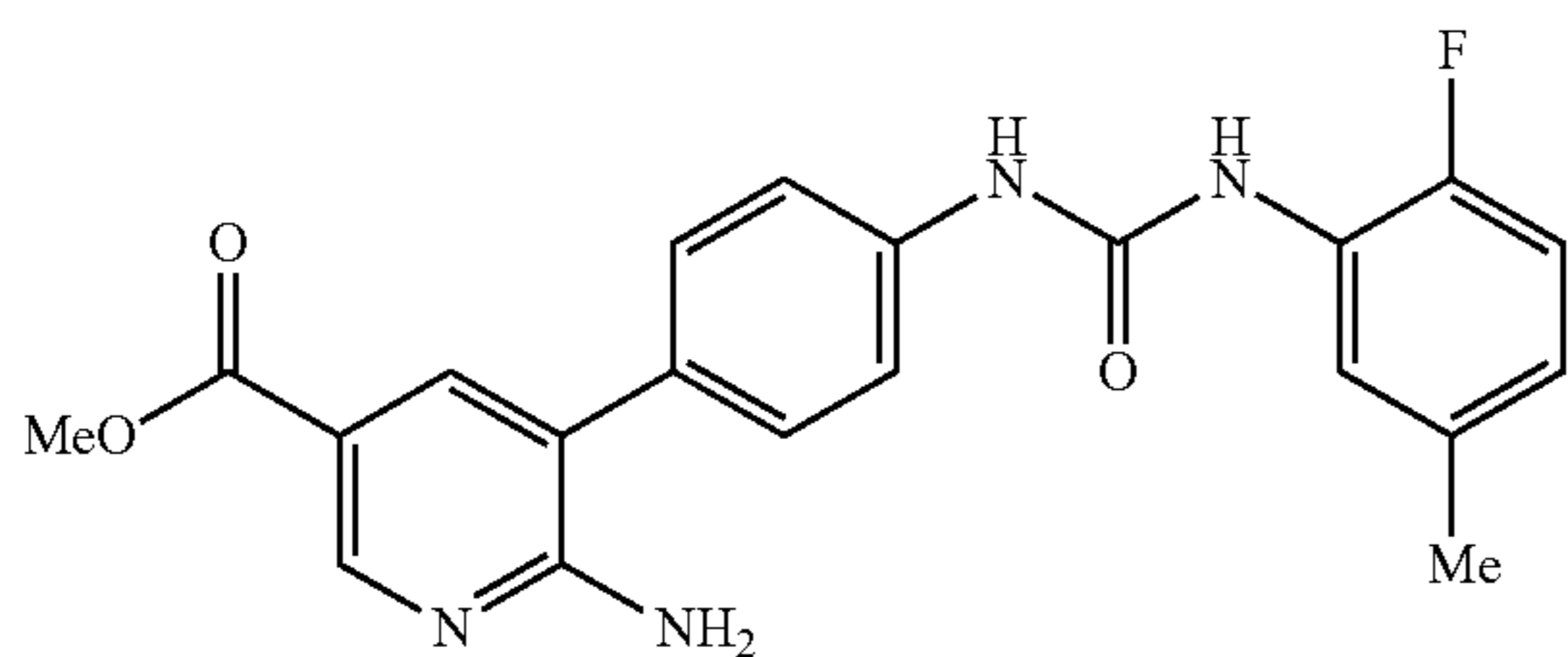
methyl 6-amino-5-(4-((2-fluoro-5-methylphenyl)carbamoyl)amino)phenylpyridine-3-carboxylate
