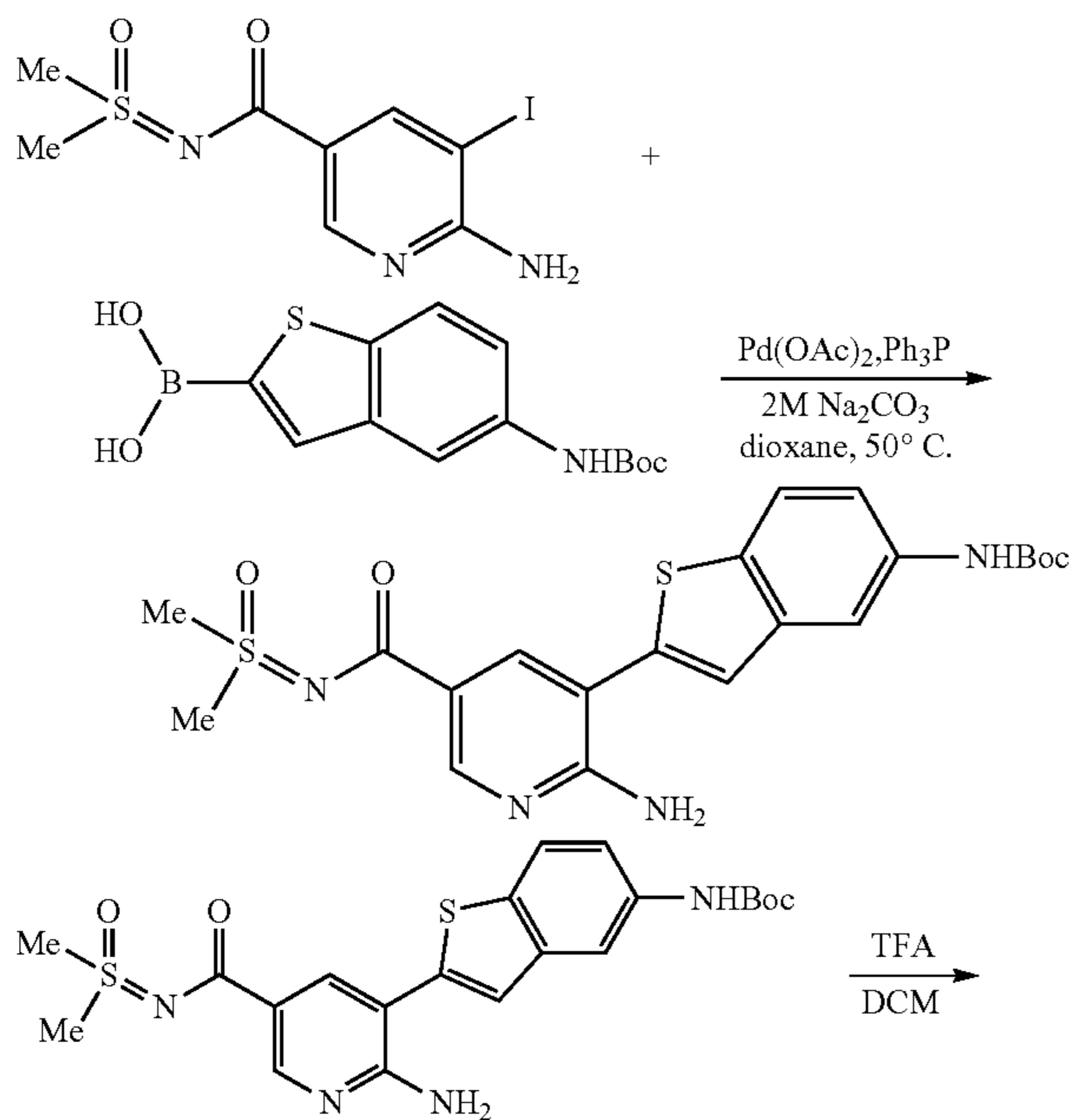
Scheme 6
