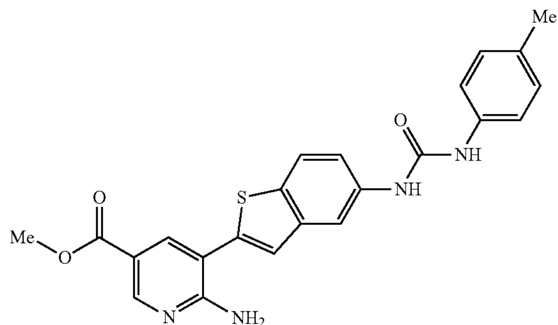
methyl 6-amino-5-[5-({[(4-methylphenyl)amino]carbonyl}amino)-1-benzothien-2-yl]nicotinate
