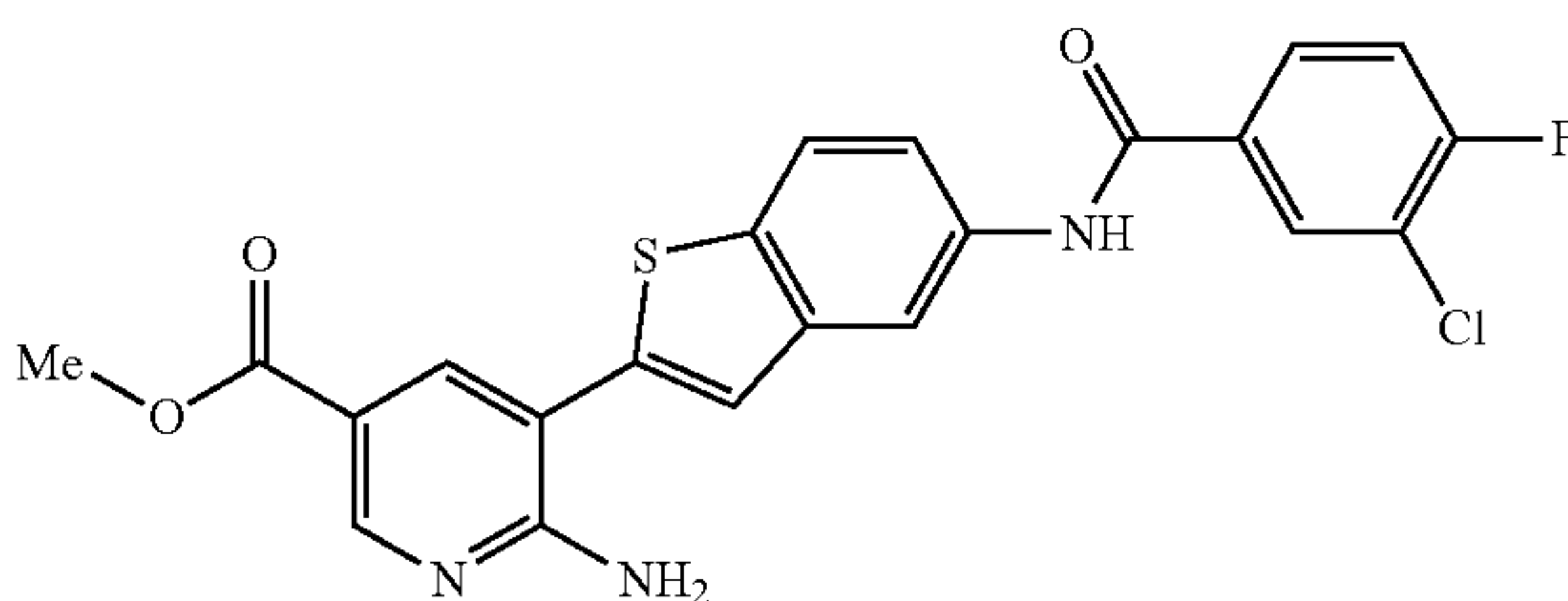
methyl 6-amino-5-[5-[(3-chloro-4-fluorobenzoyl)amino]-1-benzothien-2-yl]nicotinate
