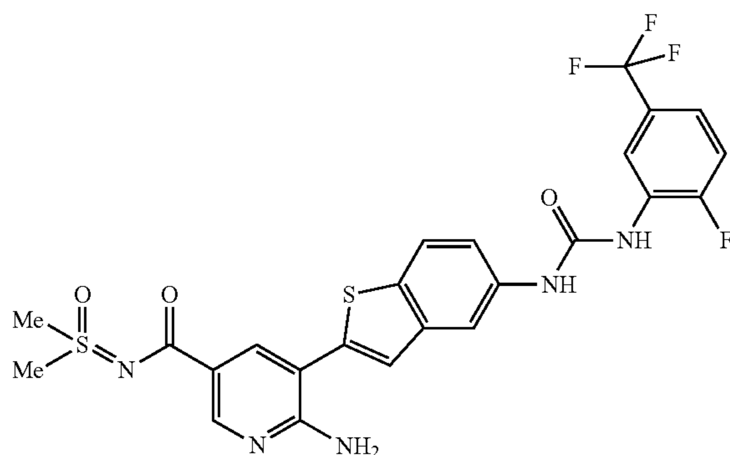
6-amino-N-[dimethyl(oxido)- \lambda^4 -sulfanylidene]-5-{5-[(2-fluoro-5-(trifluoromethyl)phenyl)amino]carbonylamino}-1-benzothien-2-yl}nicotinamide
