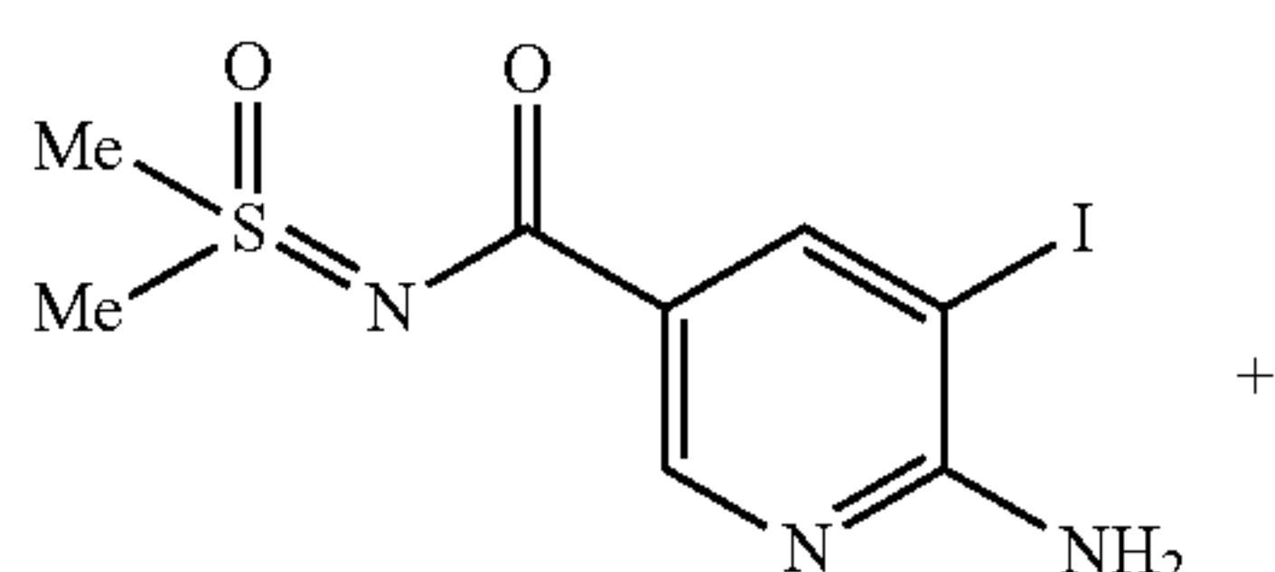
Scheme 1
