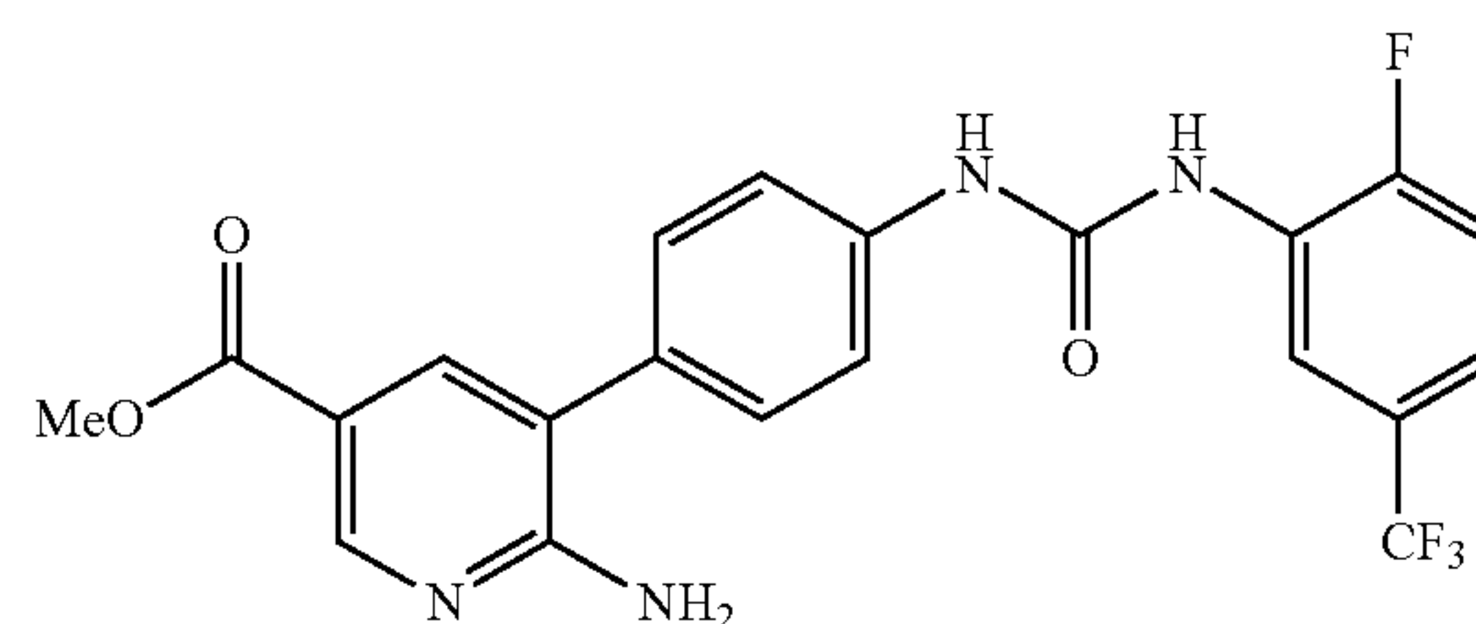
methyl 6-amino-5-[4-({(2-fluoro-5-(trifluoromethyl)phenyl)carbonyl}amino)phenyl]pyridine-3-carboxylate
