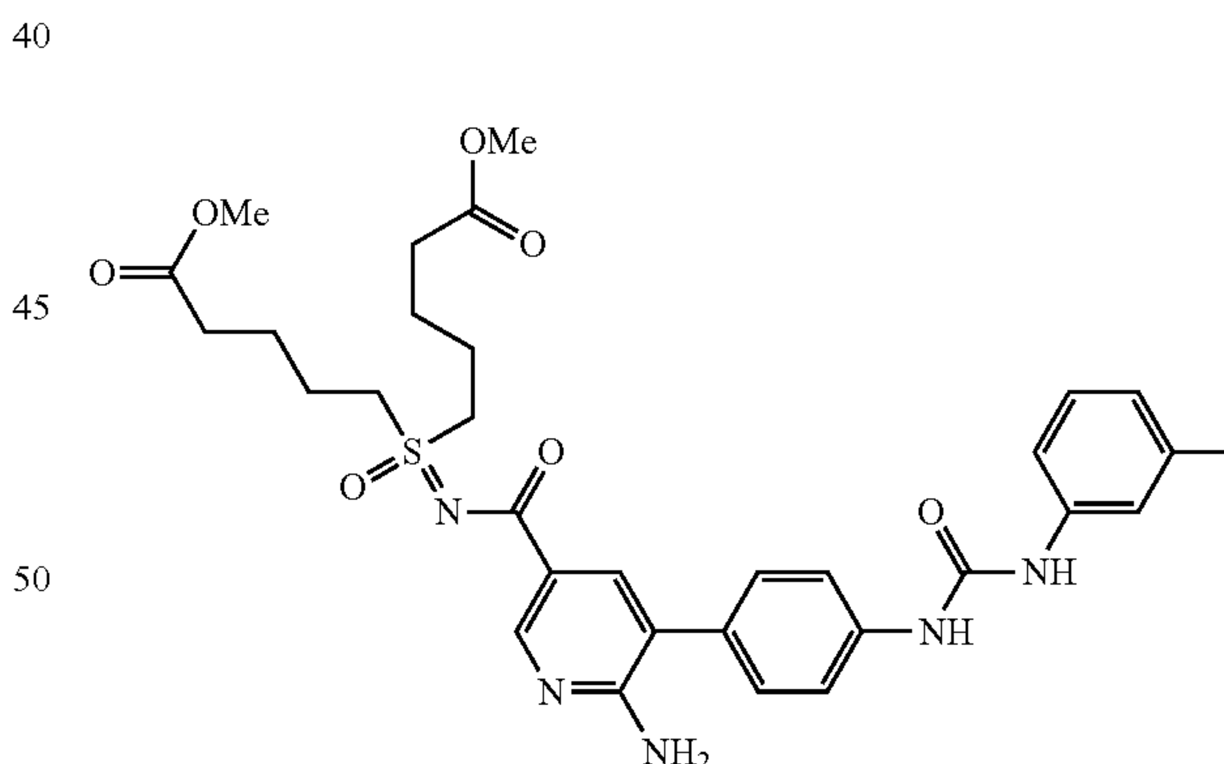
dimethyl 5,5'-(N-{{[6-amino-5-(4-{{[3-methylphenyl]carbamoyl}amino}phenyl)pyridin-3-yl]carbonyl}ulfonimidoyl}dipentanoate
