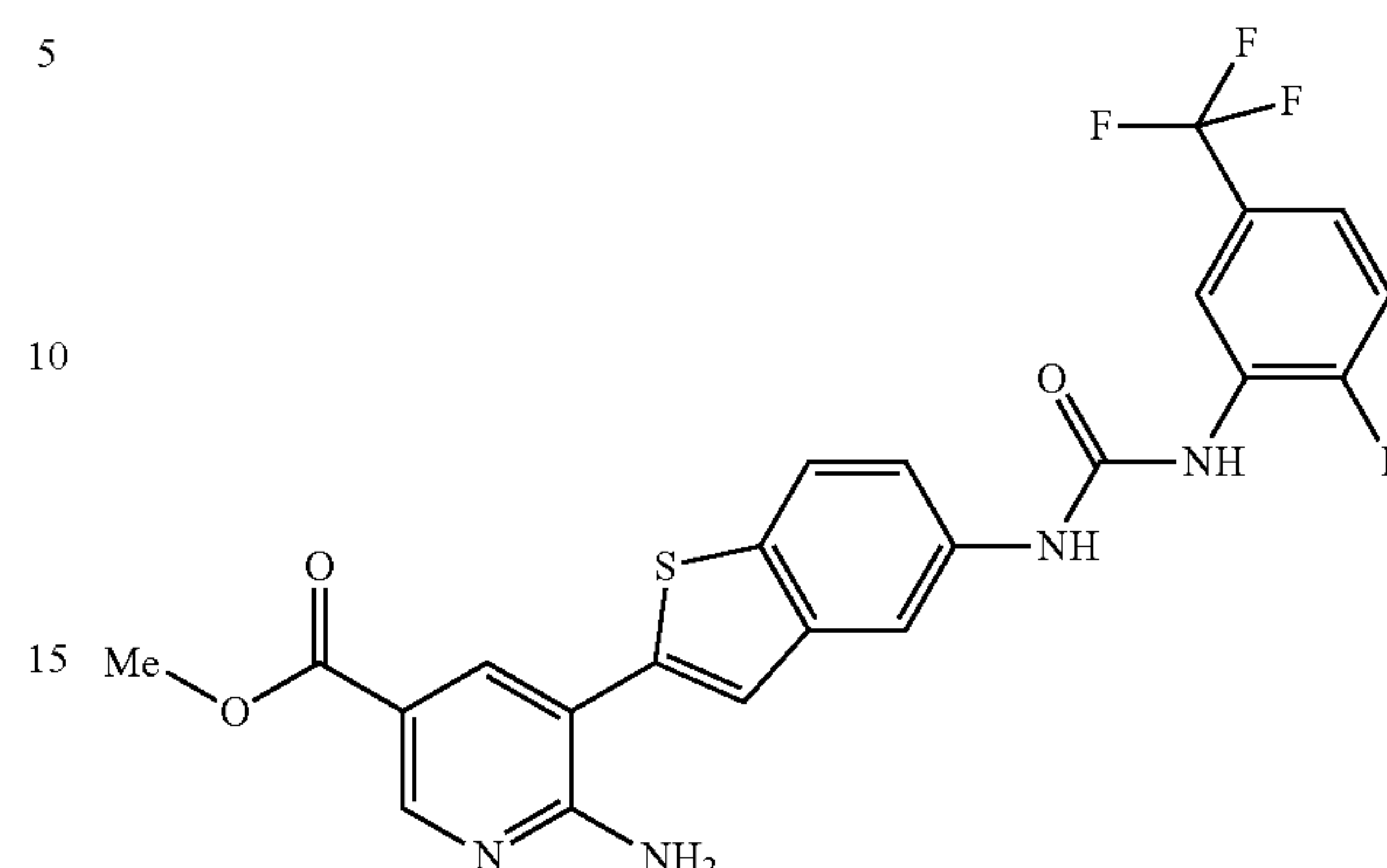
methyl 6-amino-5-{5-[(2-fluoro-5-(trifluoromethyl)phenyl)amino]carbonylamino}-1-benzothien-2-yl}nicotinate
