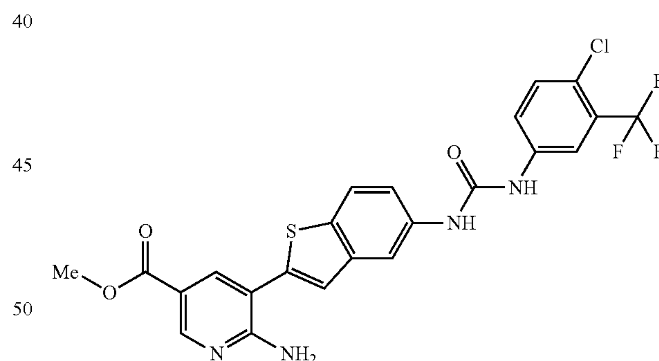
methyl 6-amino-5-{5-[(4-chloro-3-(trifluoromethyl)phenyl)amino]carbonylamino}-1-benzothien-2-yl}nicotinate
