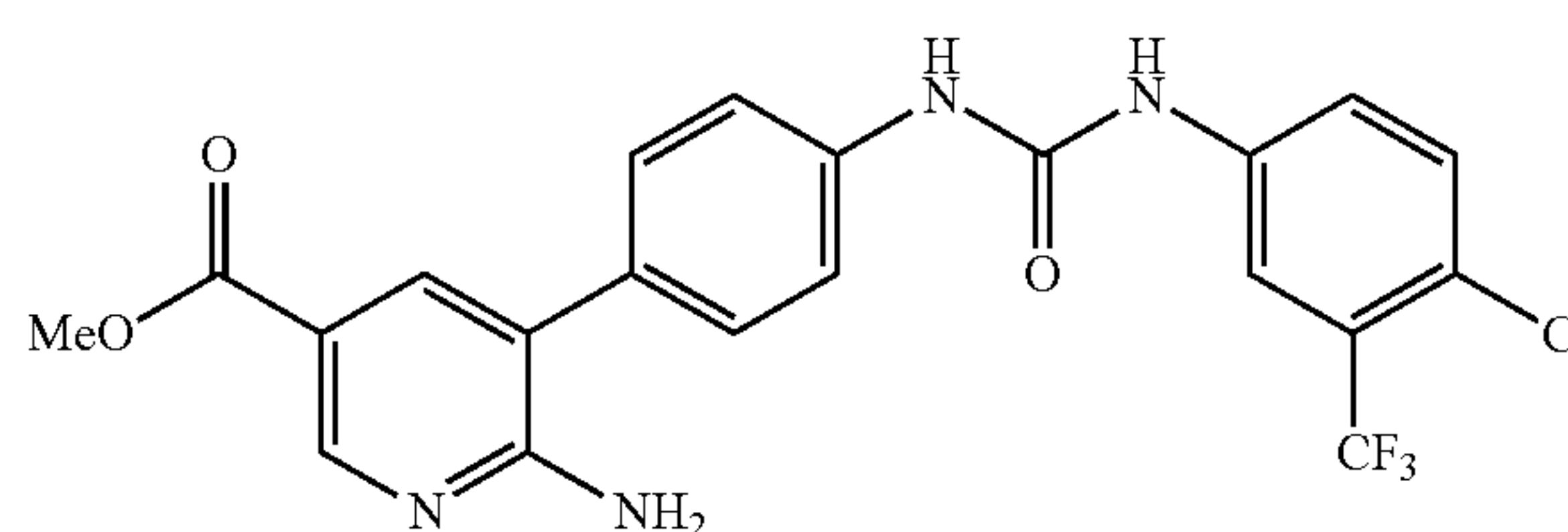
methyl 6-amino-5-[4-({(4-chloro-3-(trifluoromethyl)phenyl)carbonyl}amino)phenyl]pyridine-3-carboxylate
