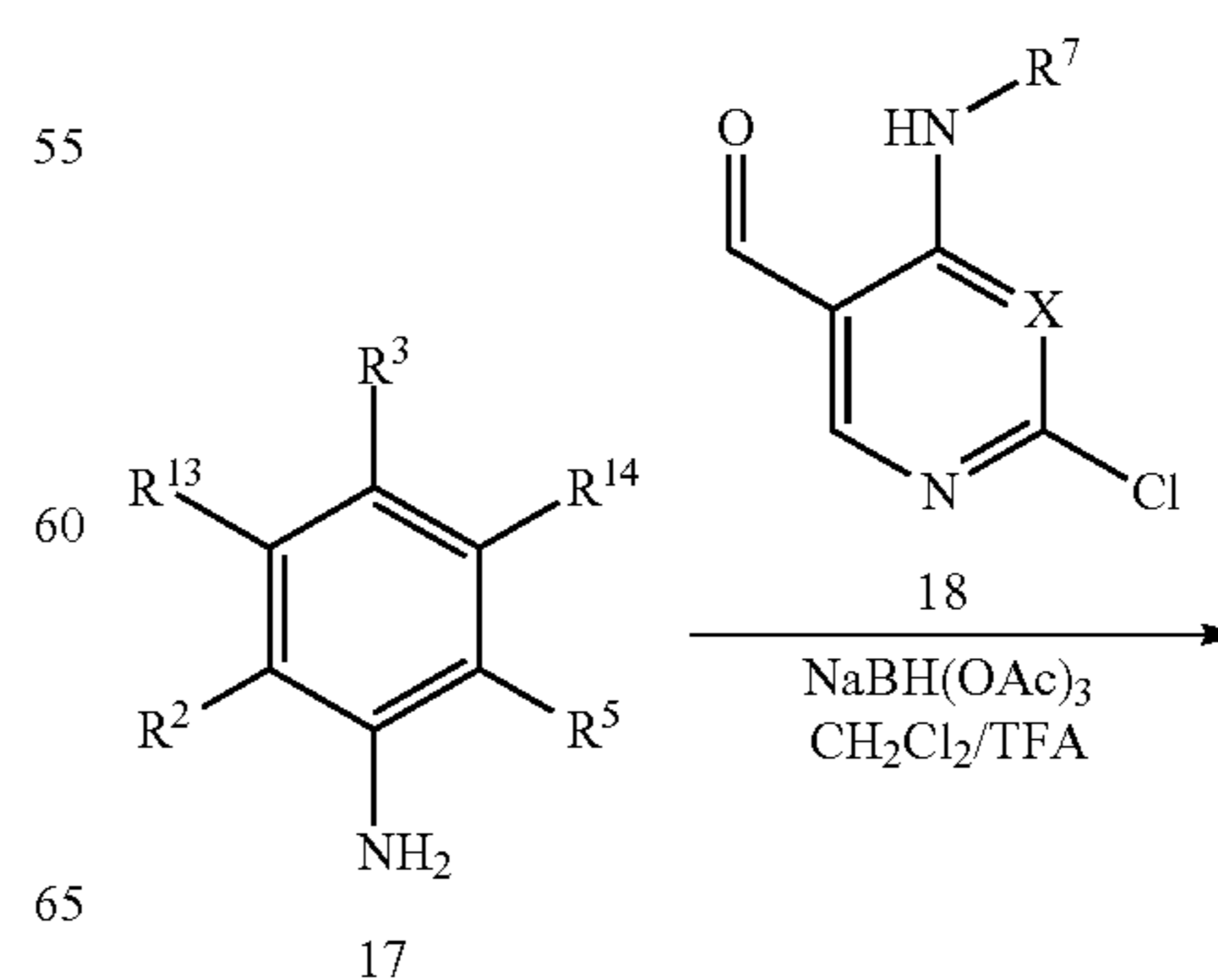
Scheme 5
