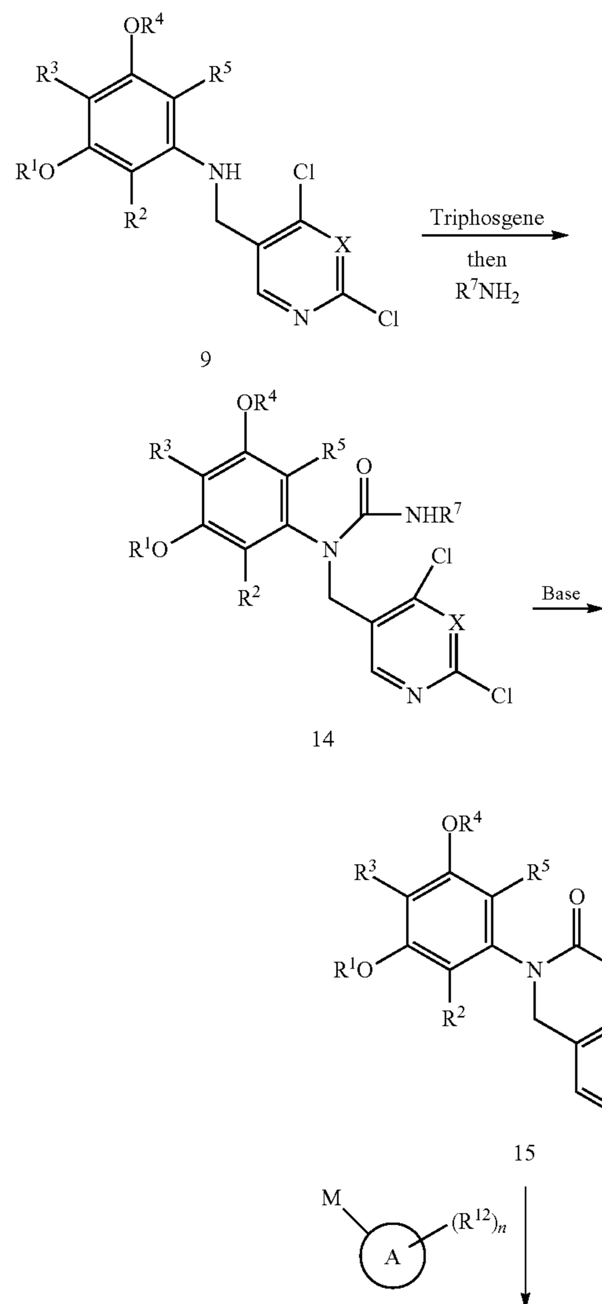
Scheme 4
