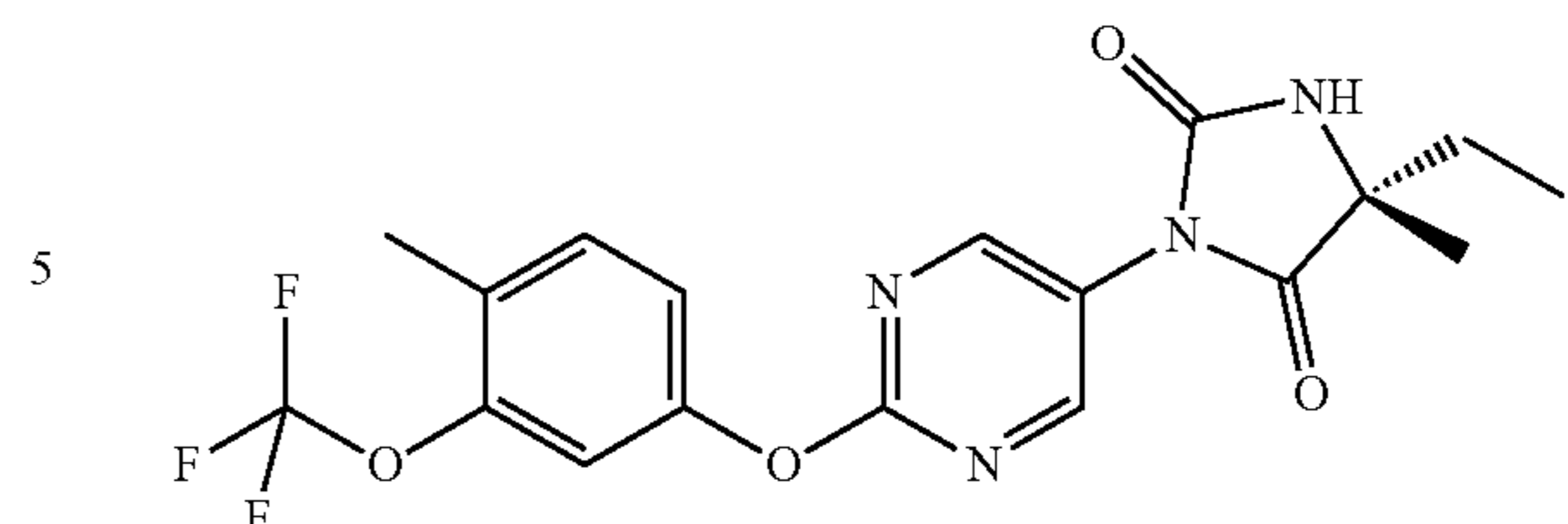
(5R)-5-ethyl-3-[6-({4-methyl-3-[(trifluoromethyl)oxy]phenyl}oxy)-3-pyridinyl]-2,4-imidazolidinedione
