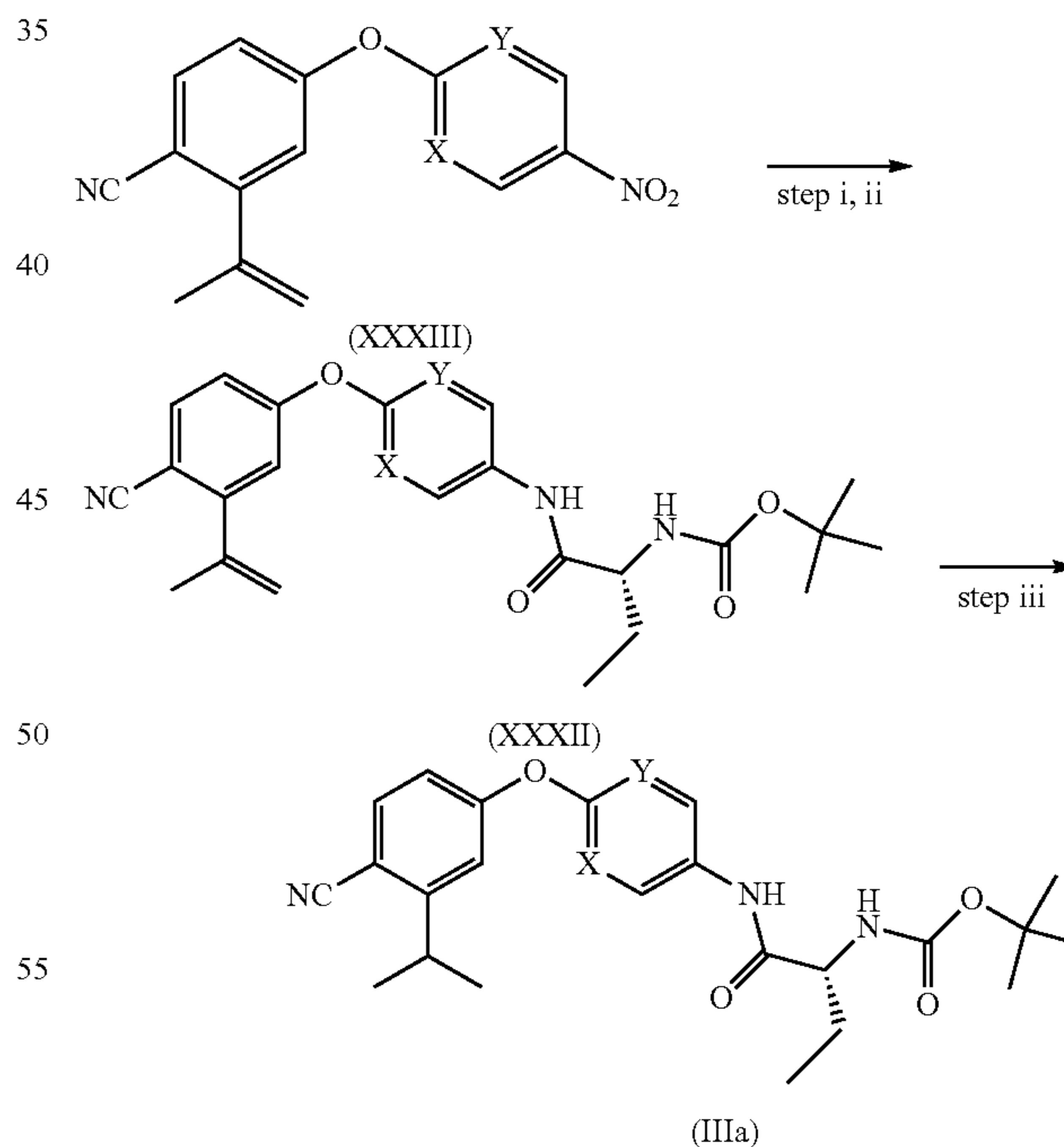
Scheme 22
