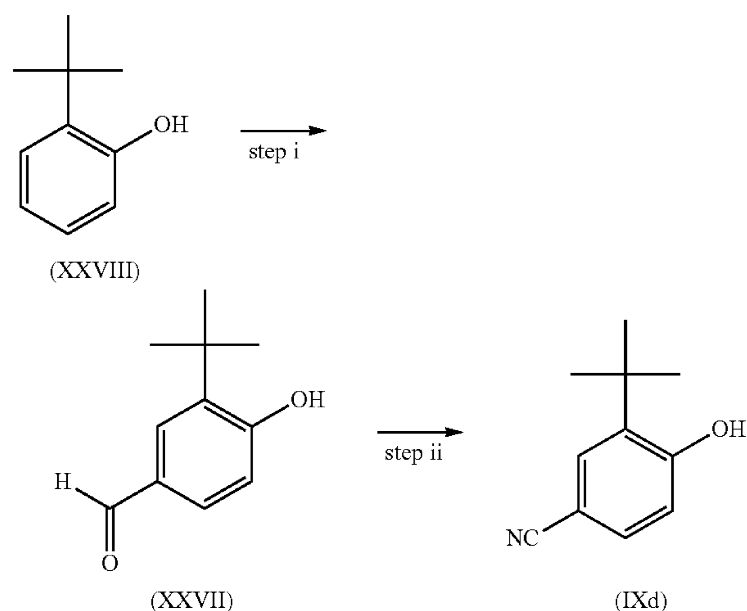
Scheme 19
