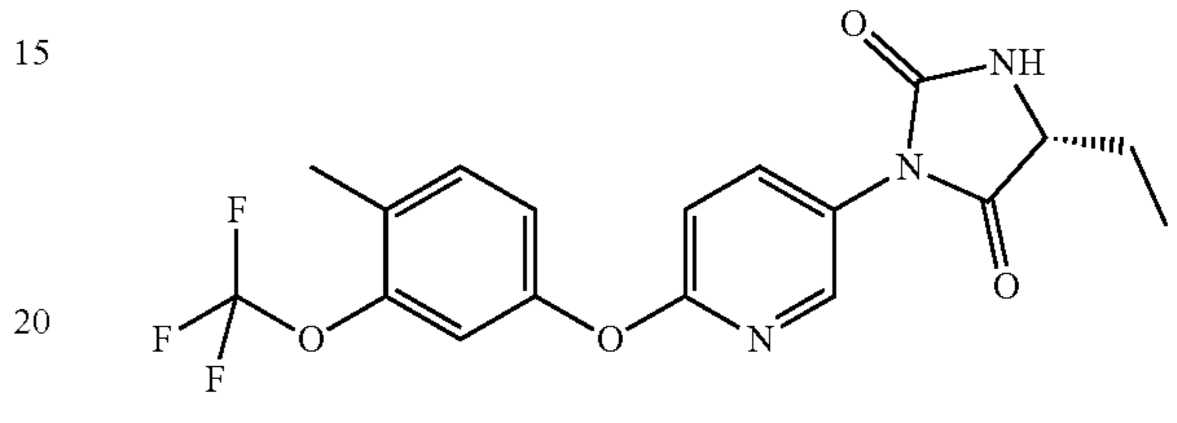
(5R)-5-ethyl-3-[2-({4-methyl-3-[(trifluoromethyl)oxy]phenyl}oxy)-5-pyrimidinyl]-2,4-imidazolidinedione
