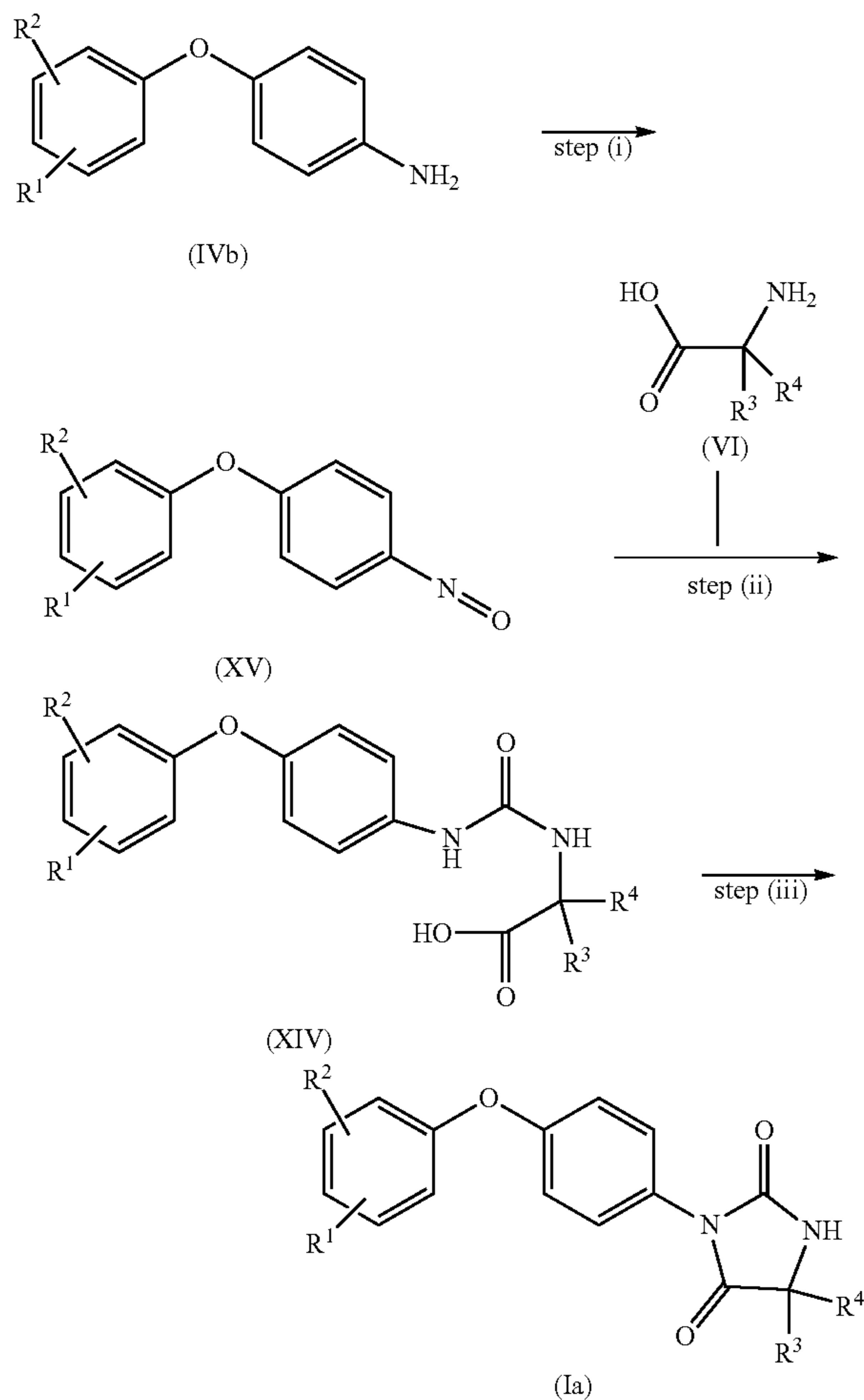
Scheme 10
