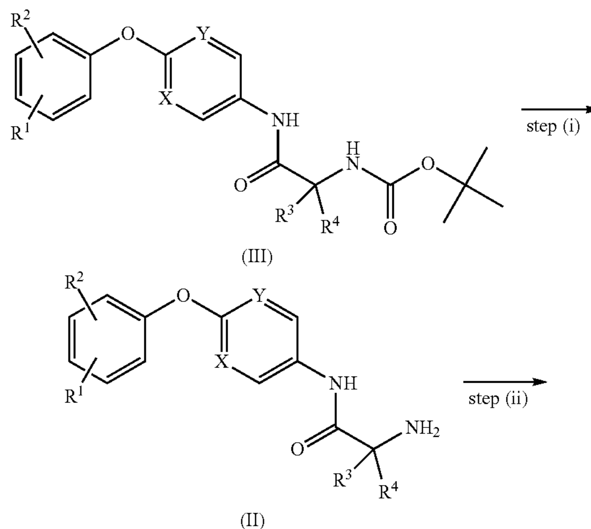
Scheme 1
