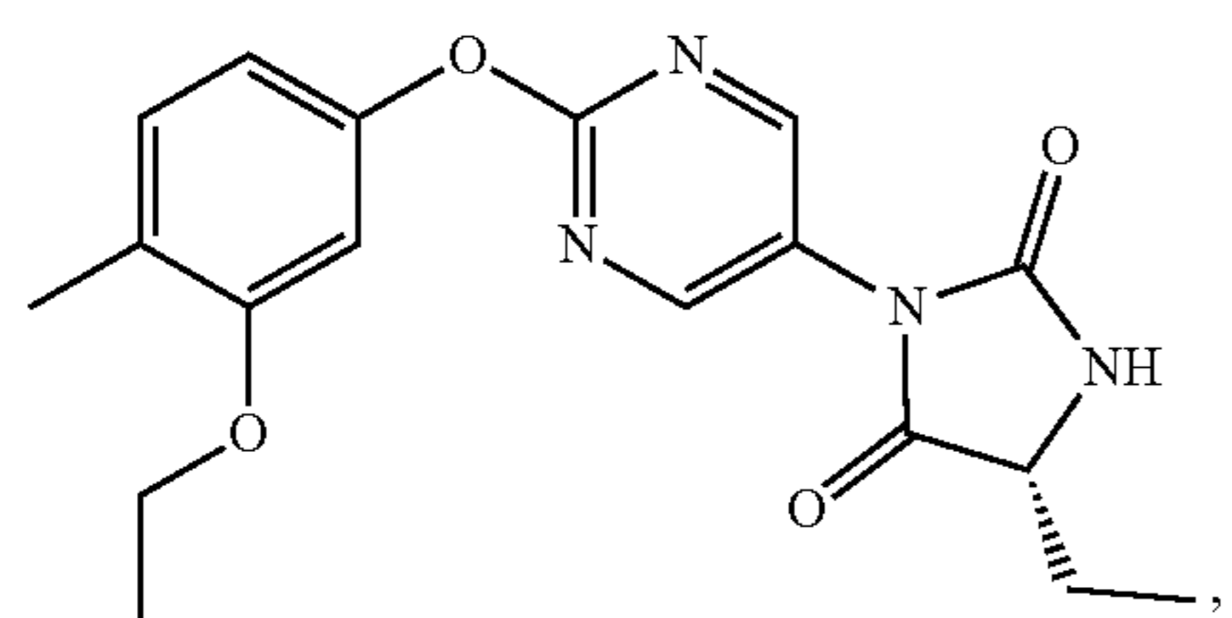
(5R)-5-ethyl-5-methyl-3-(6-{[4-methyl-3-(methoxy)phenyl]oxy}-3-pyridinyl)-2,4-imidazolidinedione
