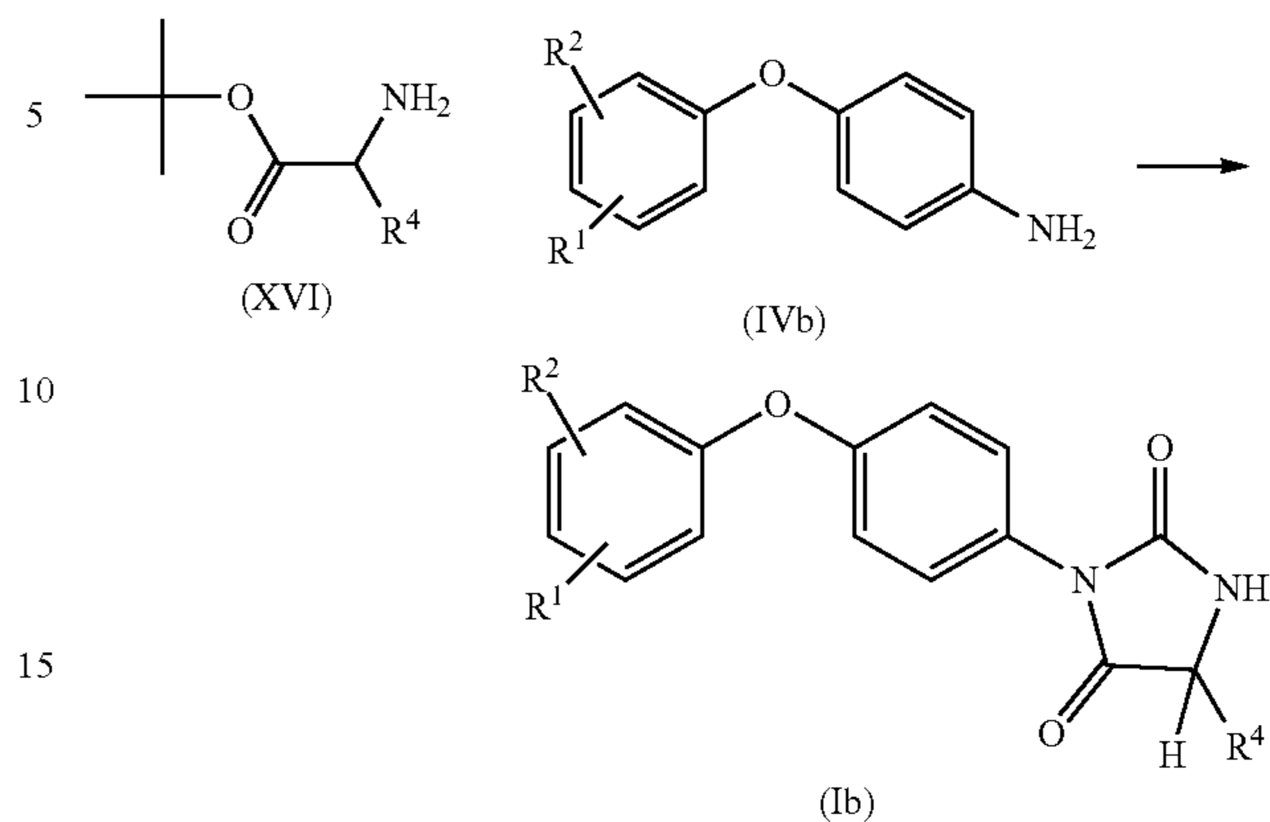
Scheme 11
