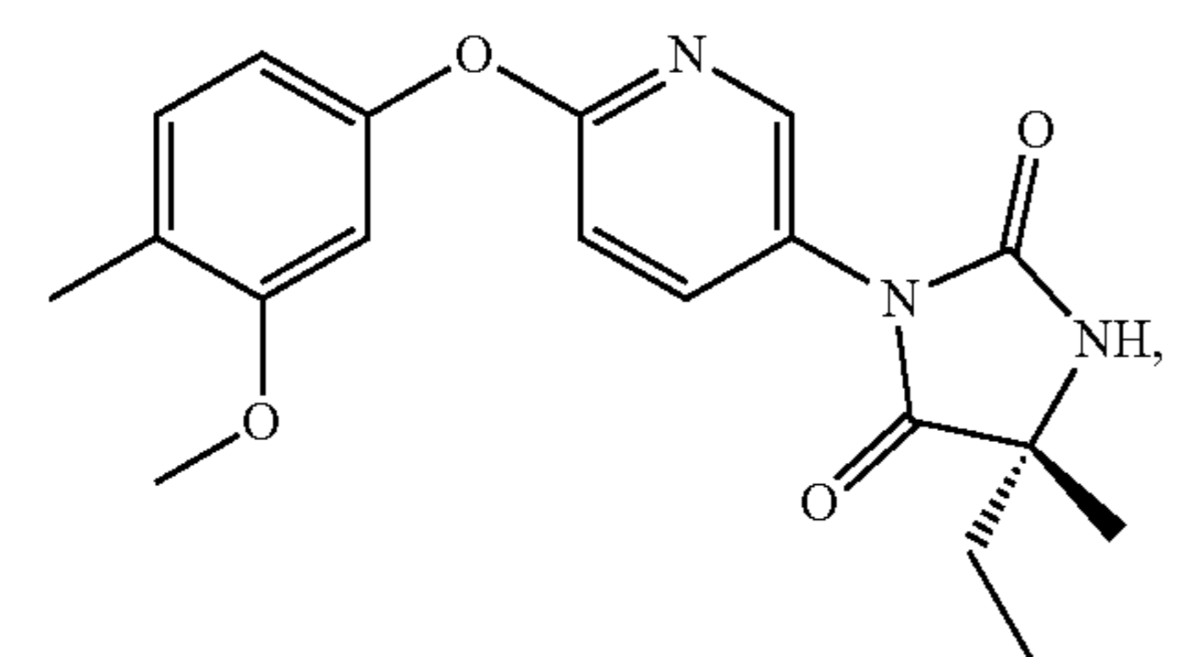
5,5-dimethyl-3-[6-({4-methyl-3-[(trifluoromethyl)oxy]phenyl}oxy)-3-pyridinyl]-2,4-imidazolidinedione
