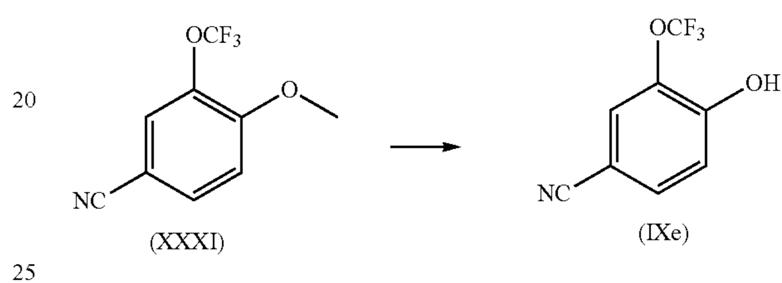
Scheme 21
