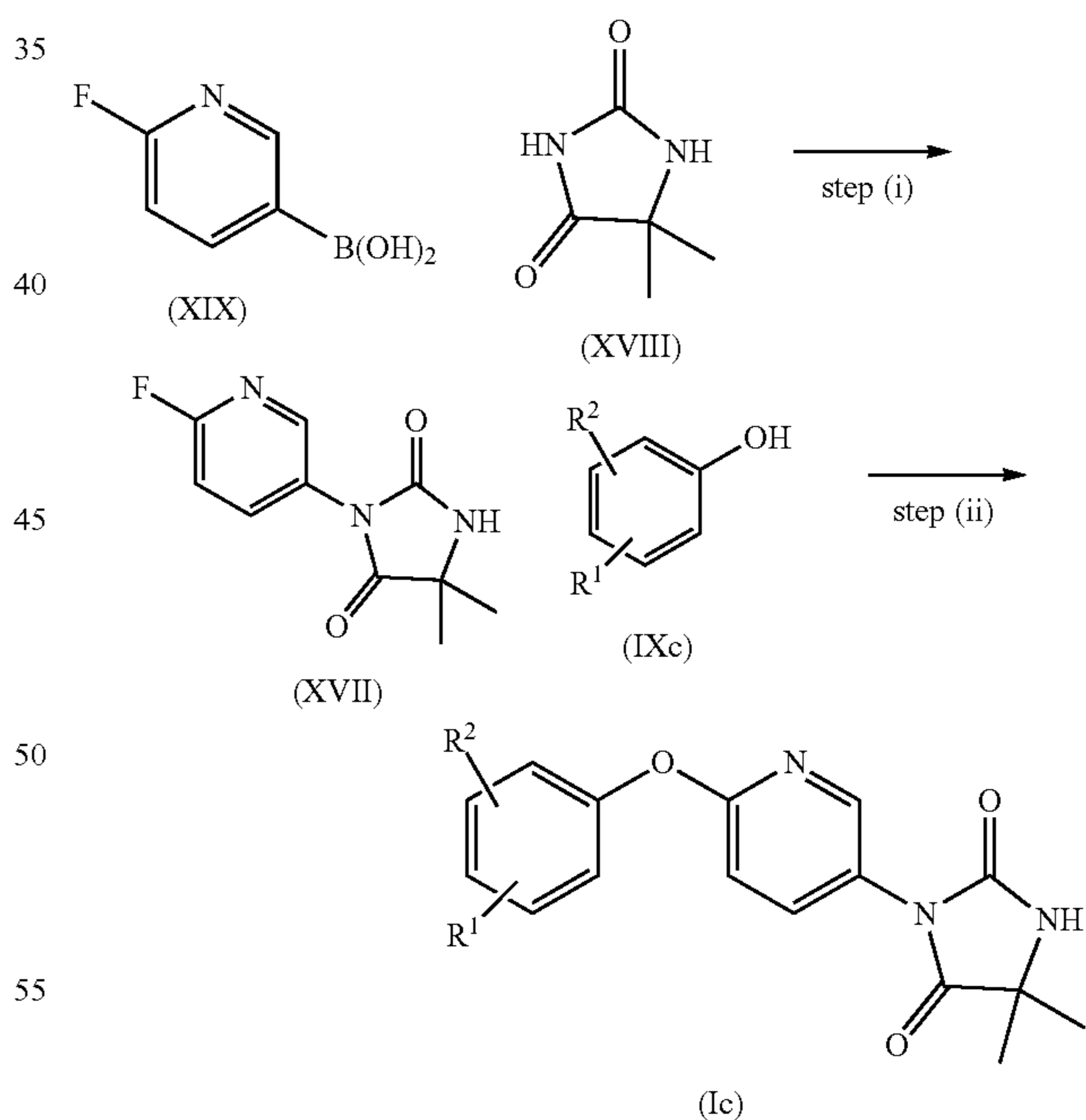
Scheme 12
