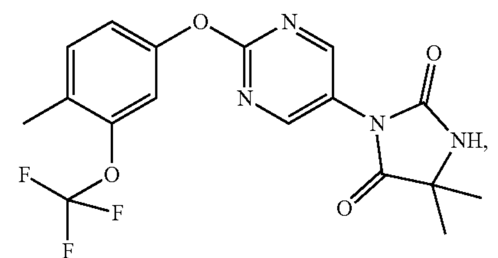
(5R)-5-ethyl-5-methyl-3-[2-({4-methyl-3-[(trifluoroethyl)oxy]phenyl}oxy)-5-pyrimidinyl]-2,4-imidazolidinedione
