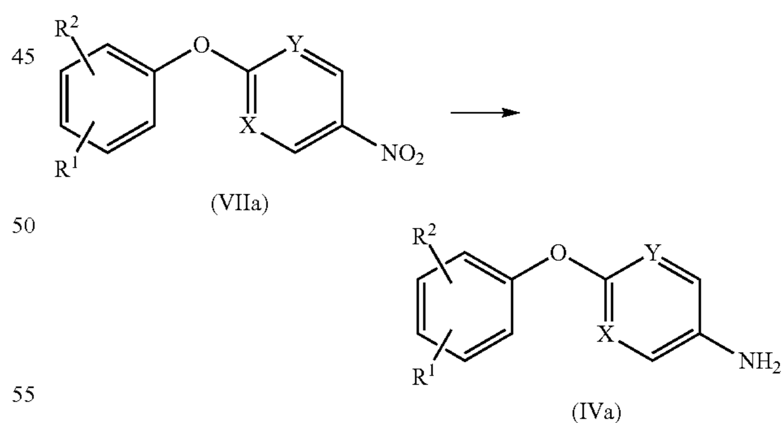
Scheme 4
