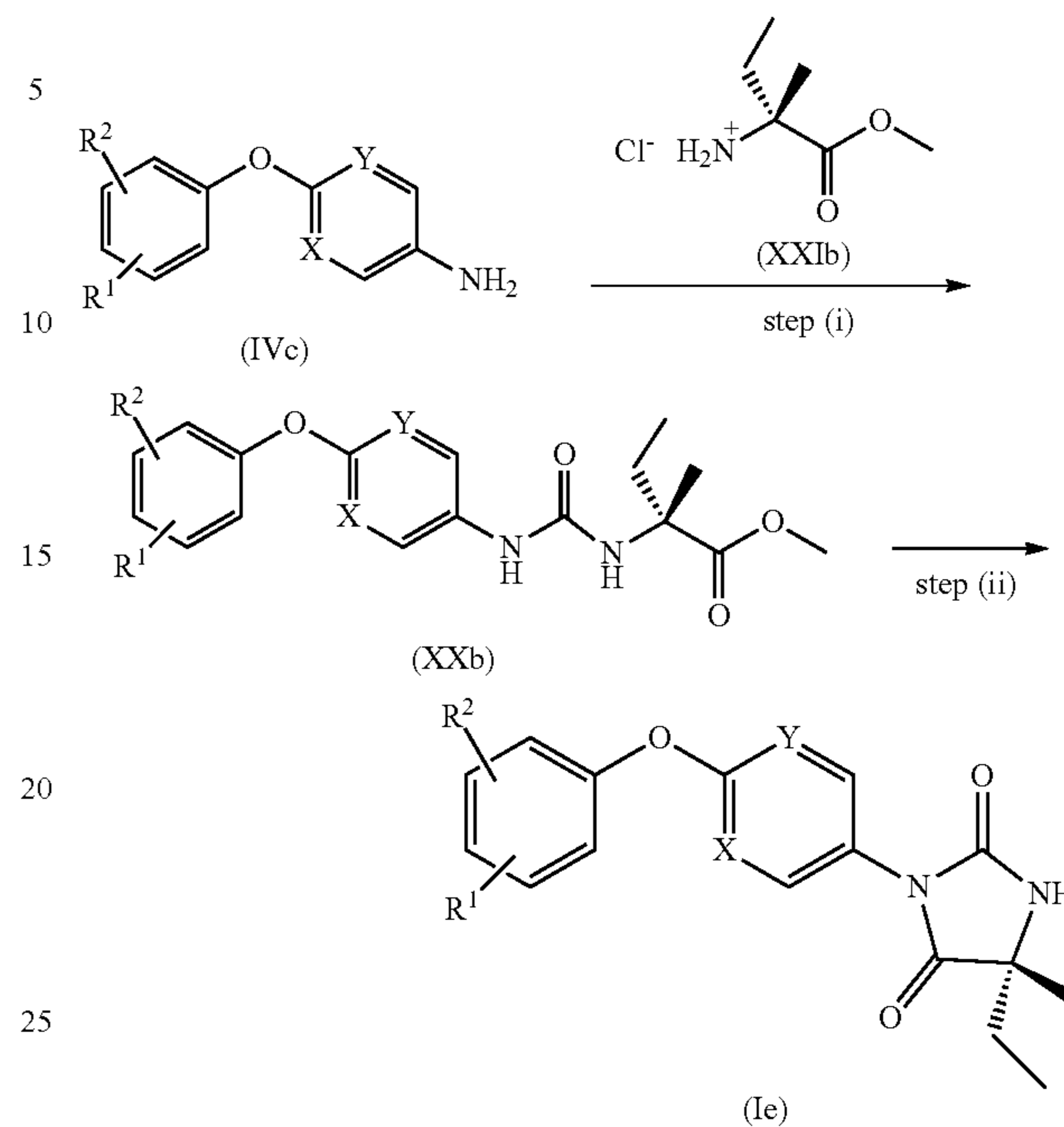
Scheme 14
