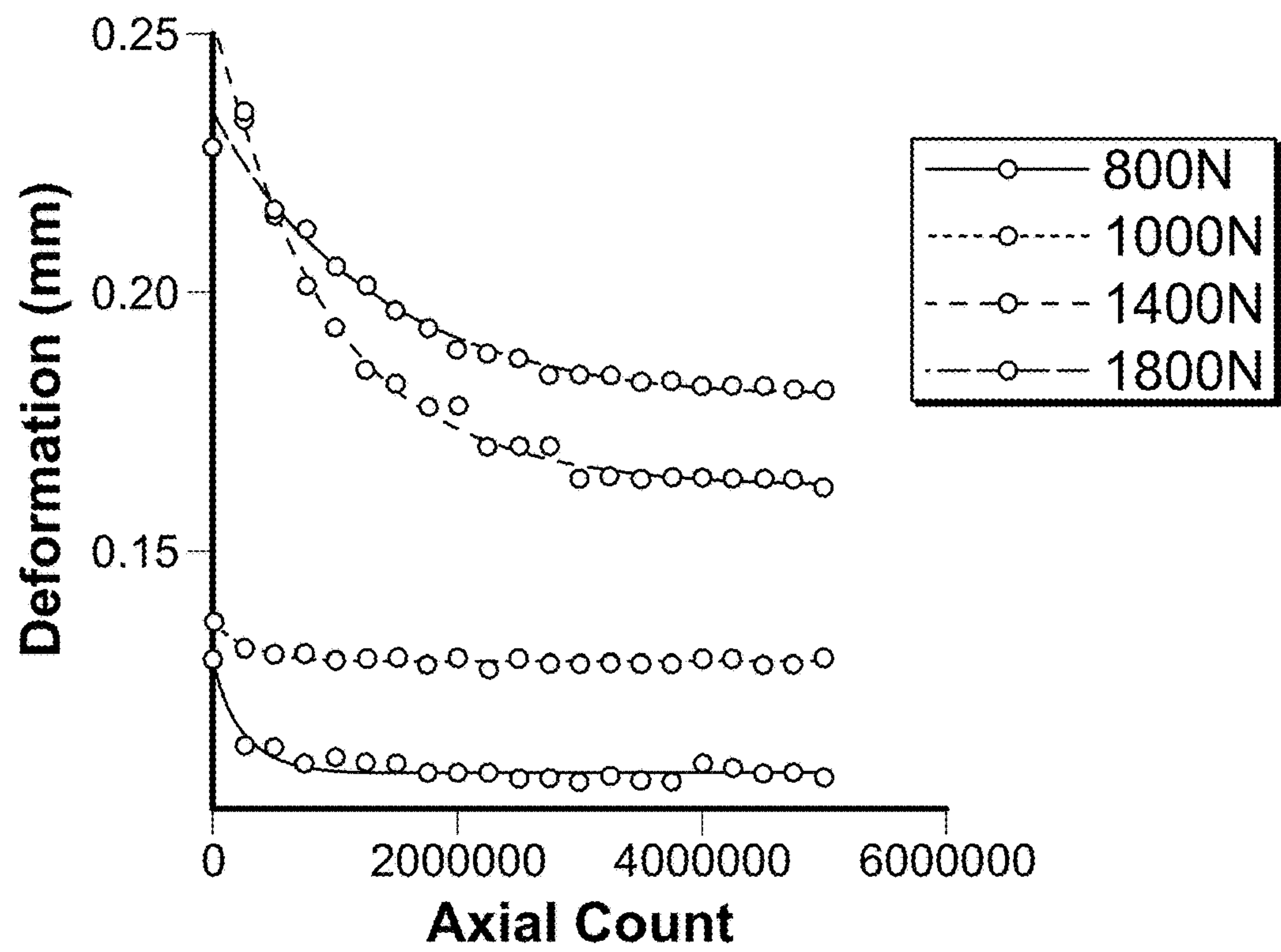
Deformation vs. Cycle Number
