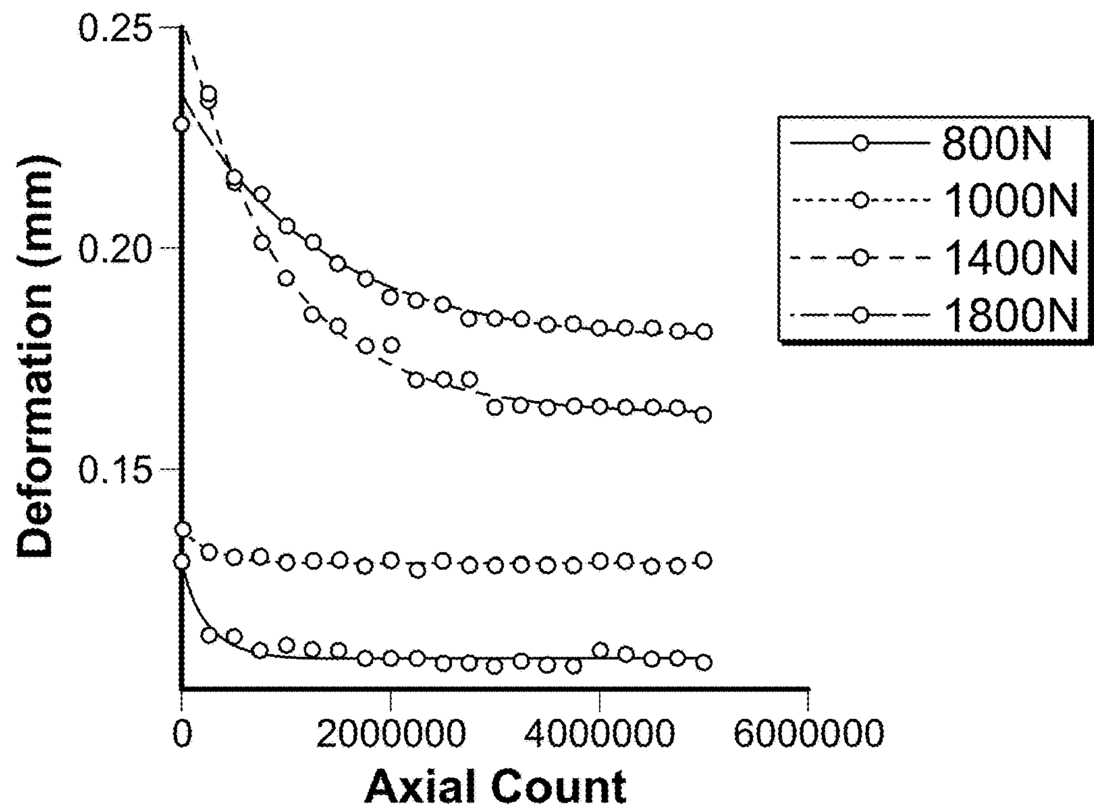
Deformation vs. Cycle Number
