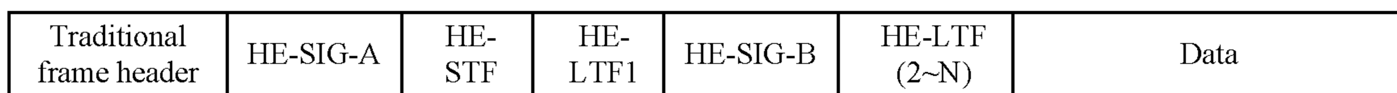
Basic frame structure 2
