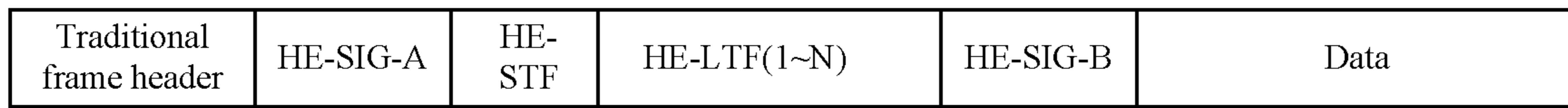
Basic frame structure 1
