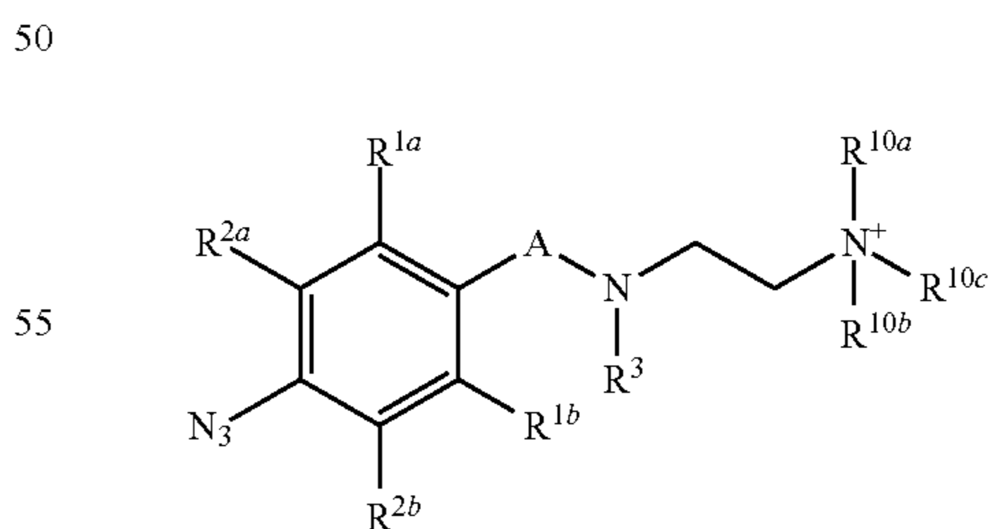
Formula IIa
