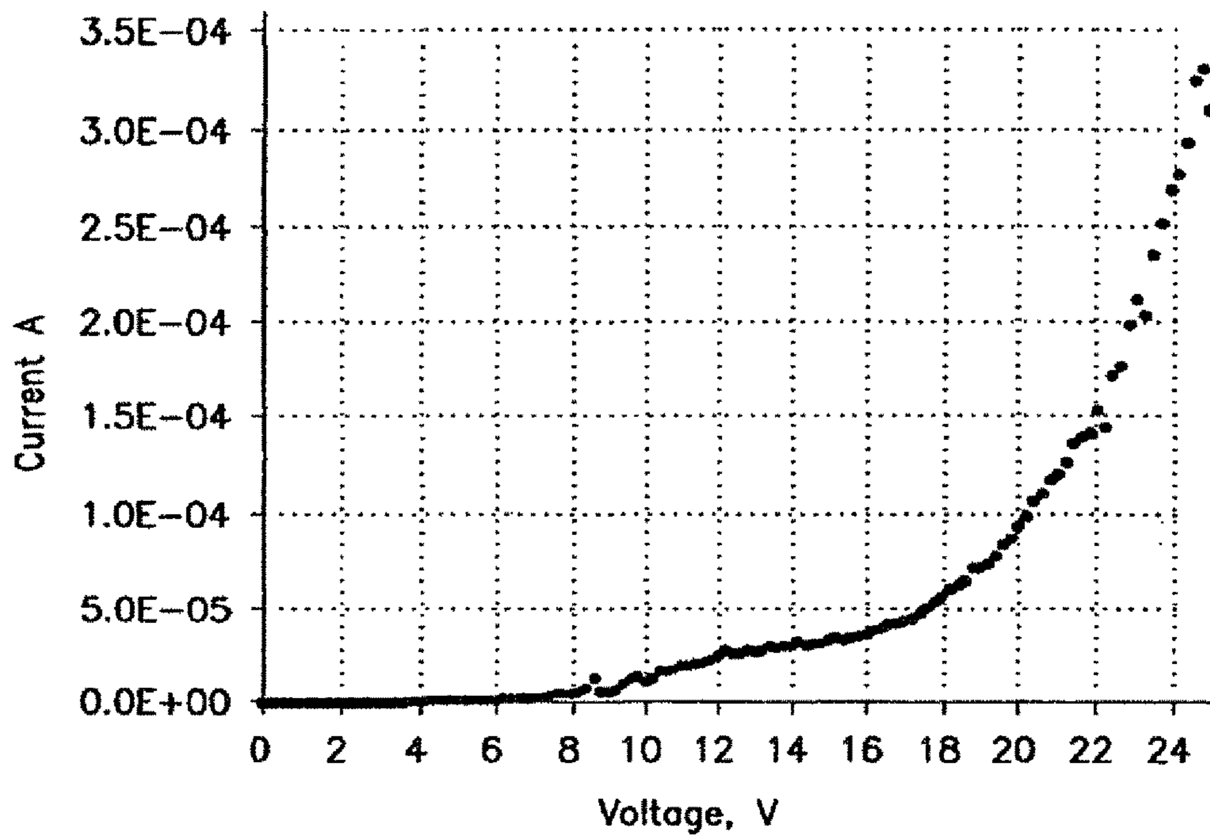
I-V characteristic of the device.
