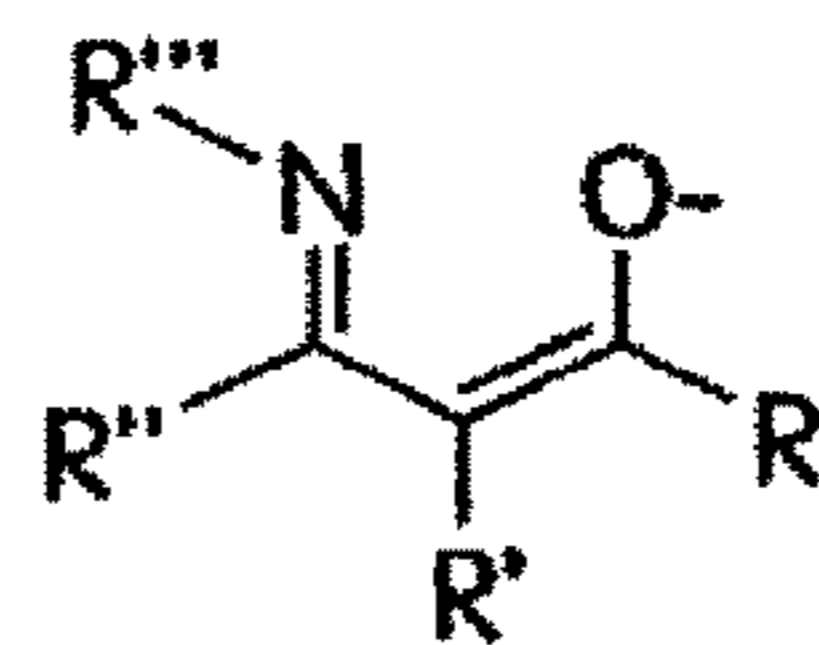
iminoacetates
