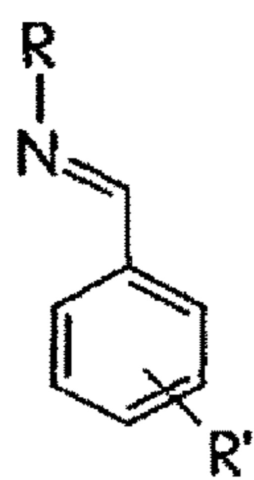
phenylimines
