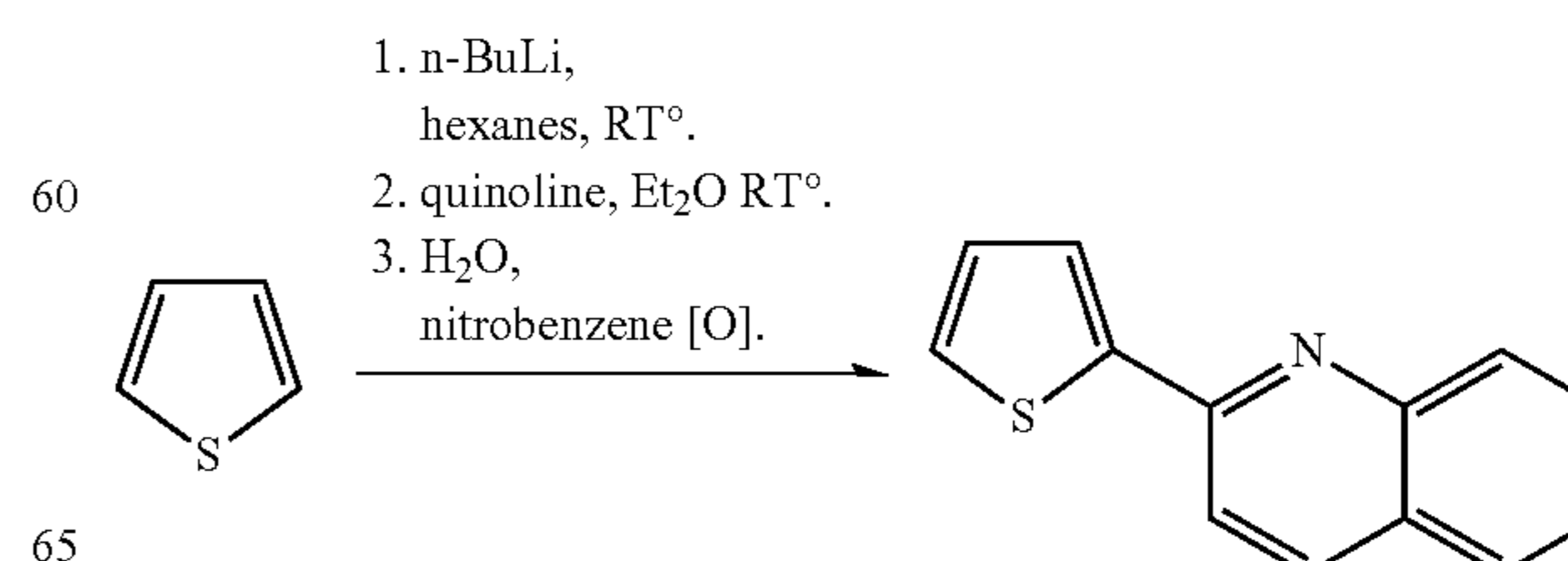
Scheme 3: Synthesis of 2-(2-thienyl)quinoline.
