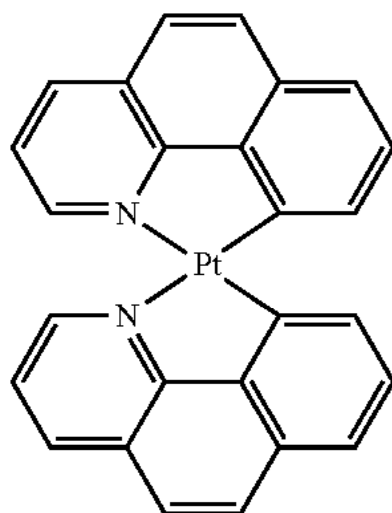
cis-Bis[benzo(h)-quinolinato-N,C] Pt(II) Pt(Bhq) 2 (3)
