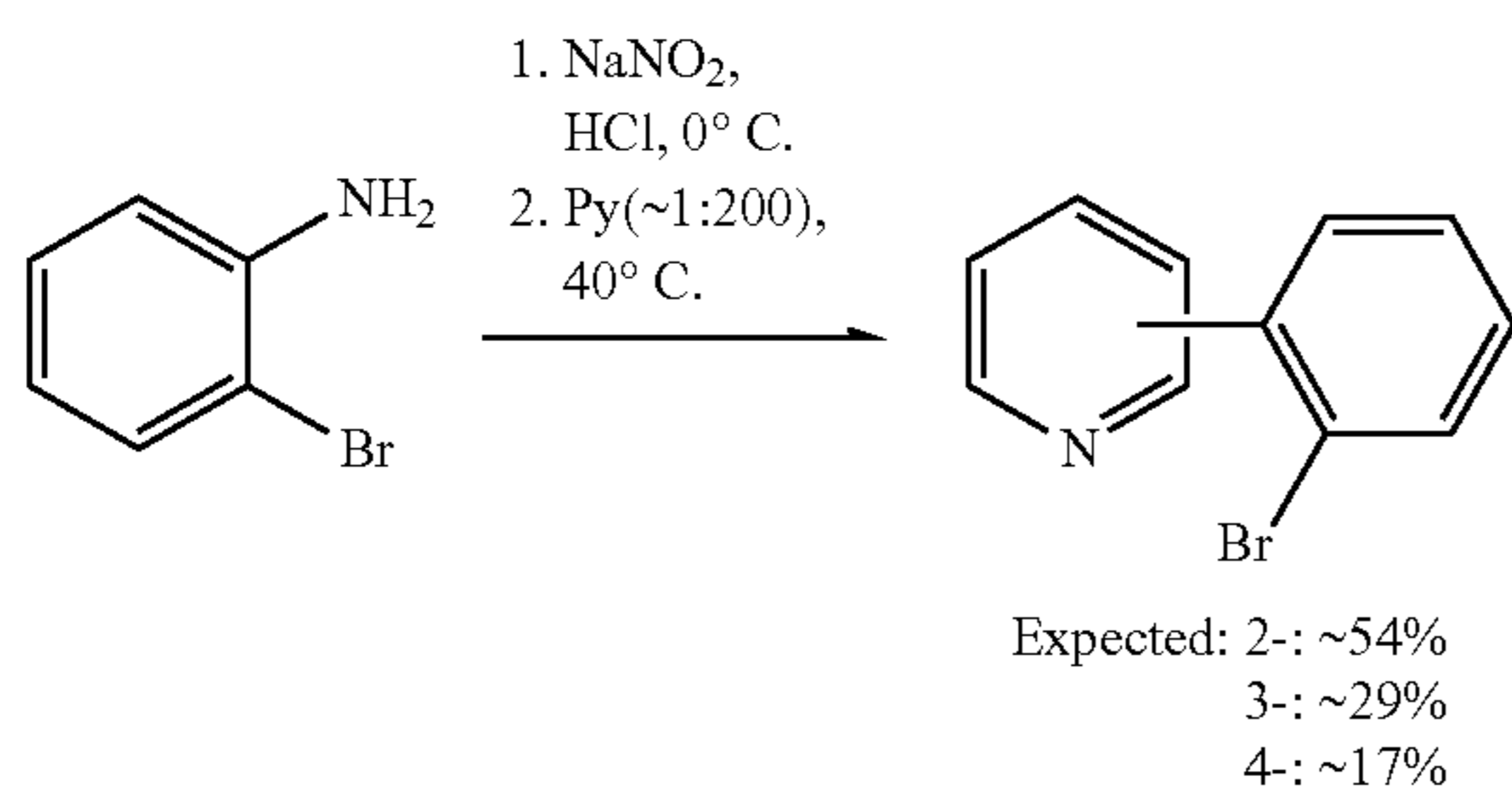
Scheme 4: Synthesis of n-(2'-bromophenyl)pyridines.
