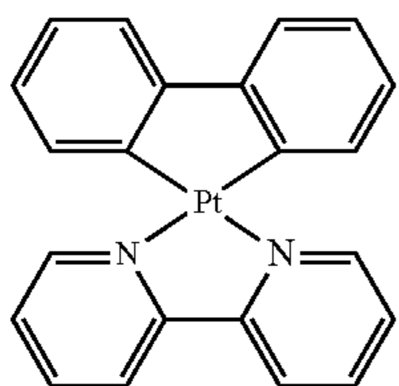
(Biphenylinato-C,C)-(bipyridinato-N,N) Pt(II) Pt(bph)(bpy)(4)
