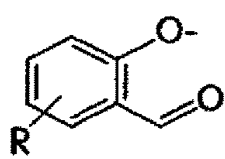
salicylaldehydes
