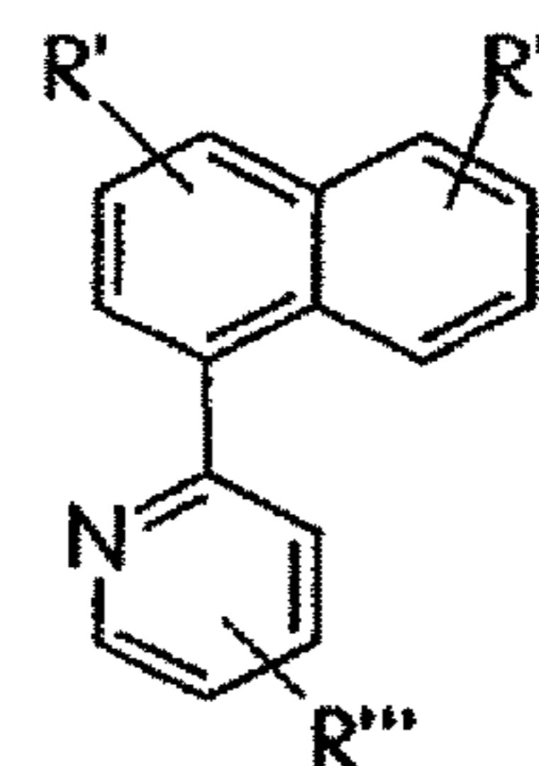
pyridyl naphthalenes
