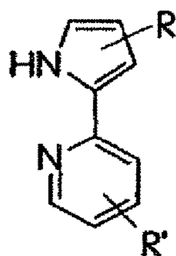
pyridylpyroles
