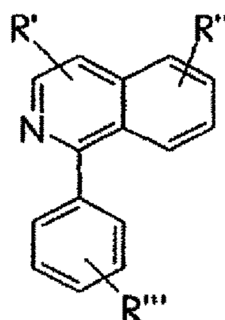
arylquinolines
