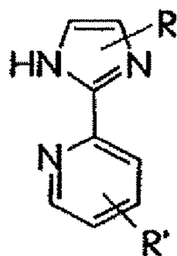
pyridylimidazoles
