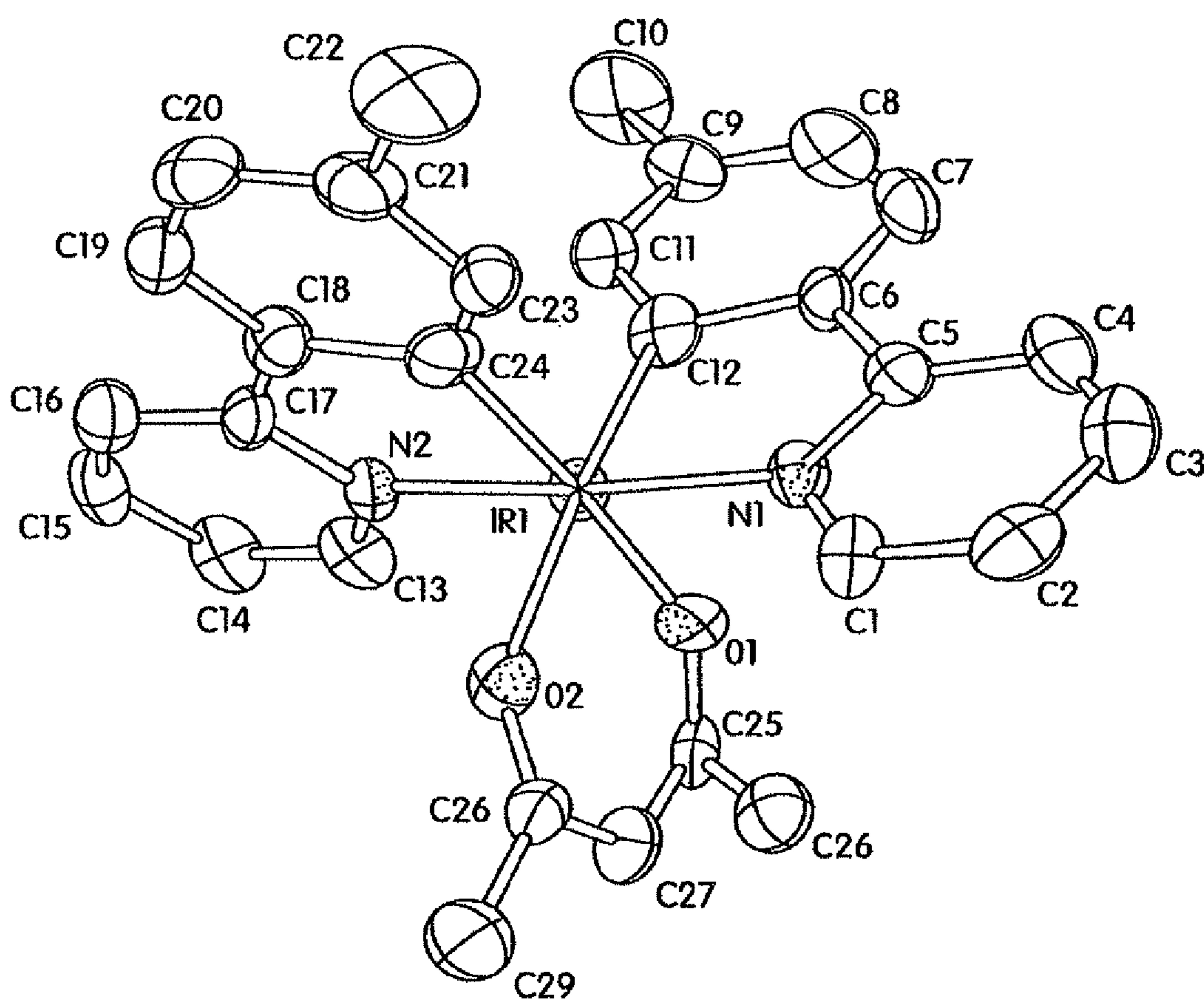
Crystal structure of tpyIr
