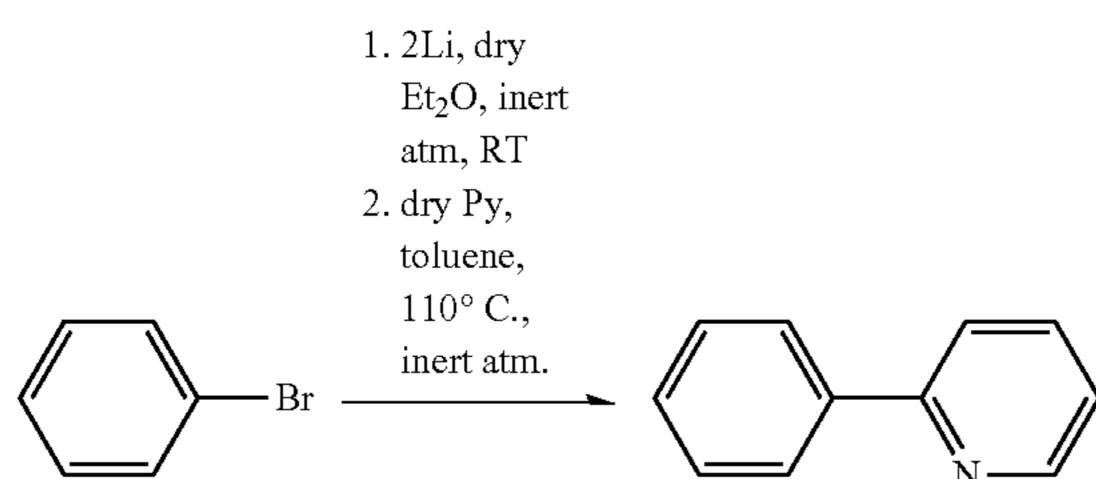
Scheme 5: Synthesis of 2-phenylpyridine.
