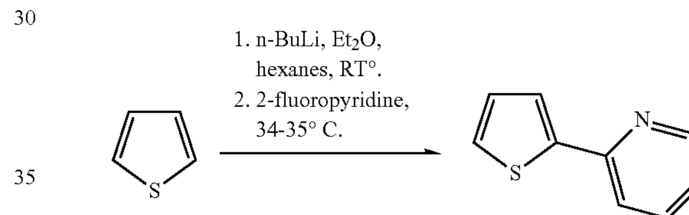
Scheme 2: Synthesis of 2-(2-thienyl)pyridine.
