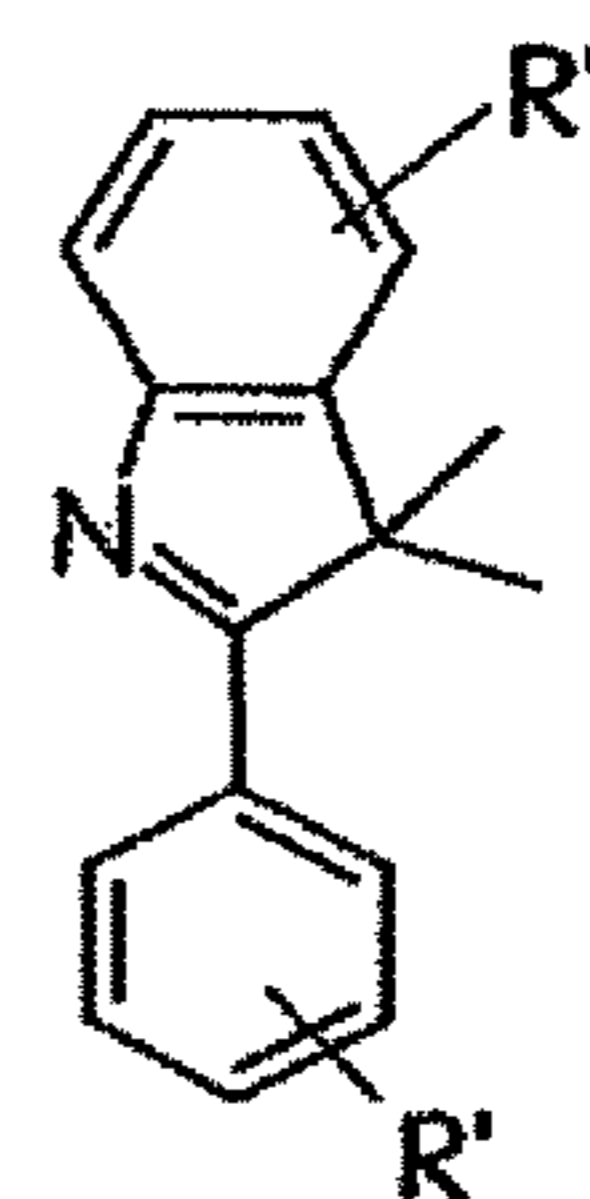
phenylindoles
