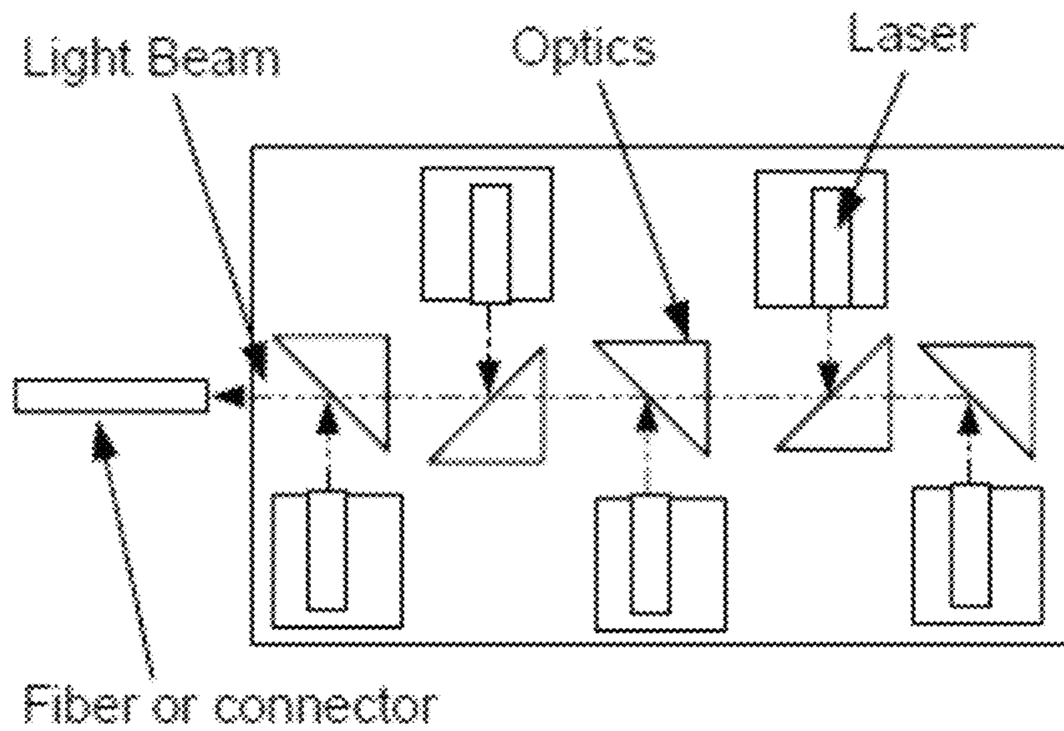
2 row configuration
