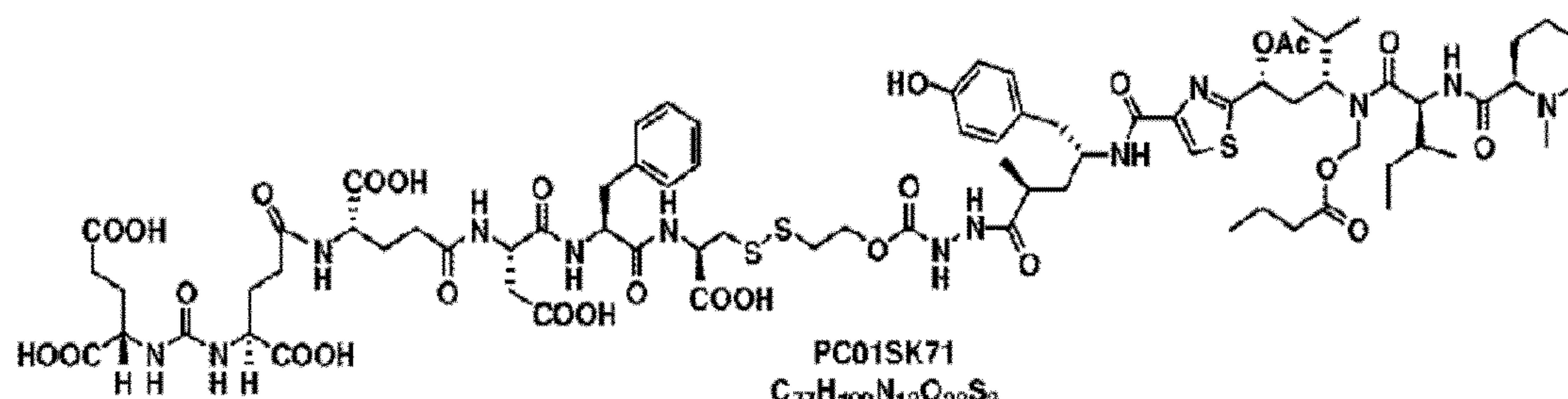
PC01SK71 C 77 H 109 N 13 O 28 S 3 Mol. Wt.: 1760.95
