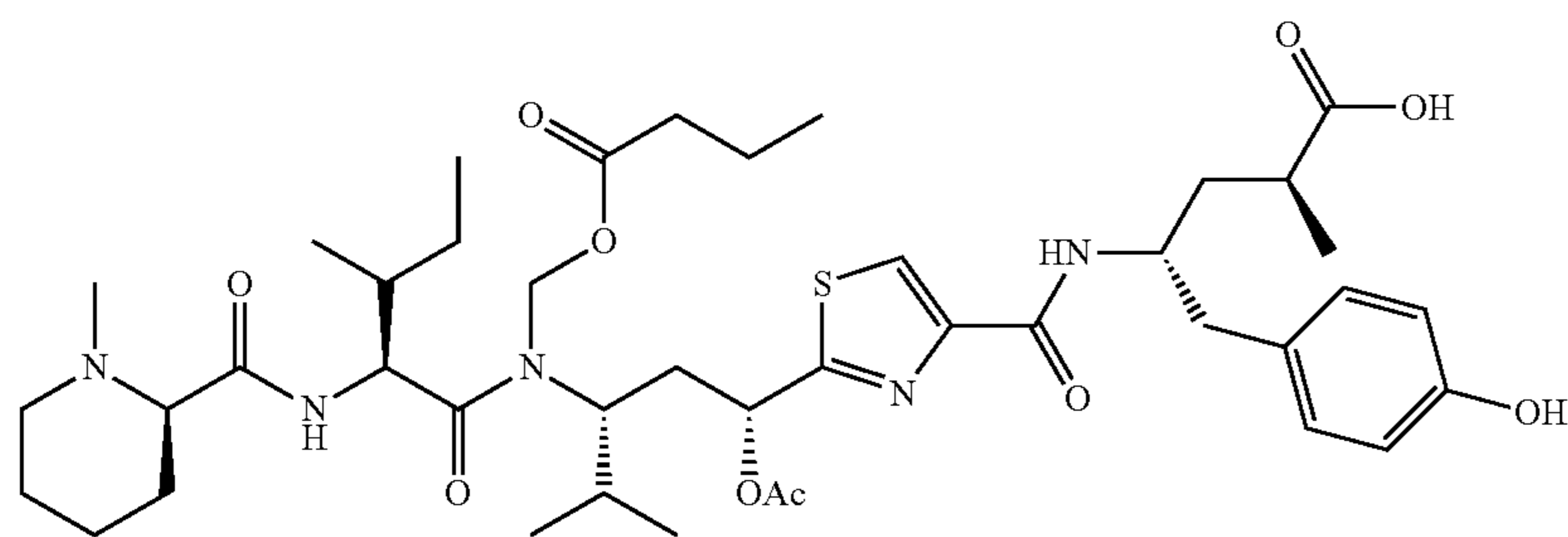
Tubulyisin B C_{42}H_{63}N_5O_{10}S Mol. Wt.: 830.04
