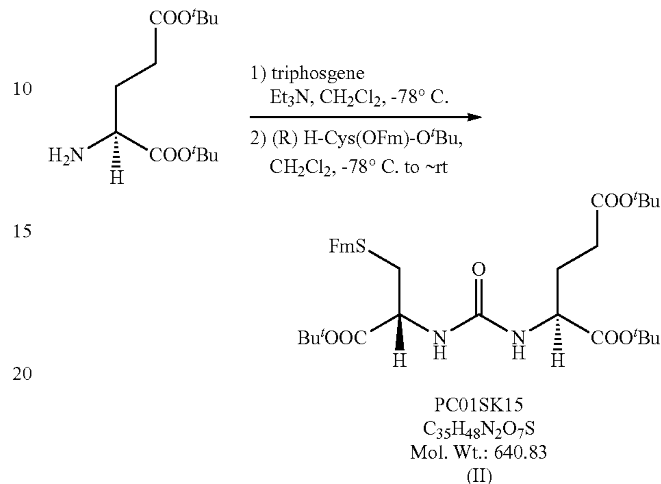
Scheme 2.2
