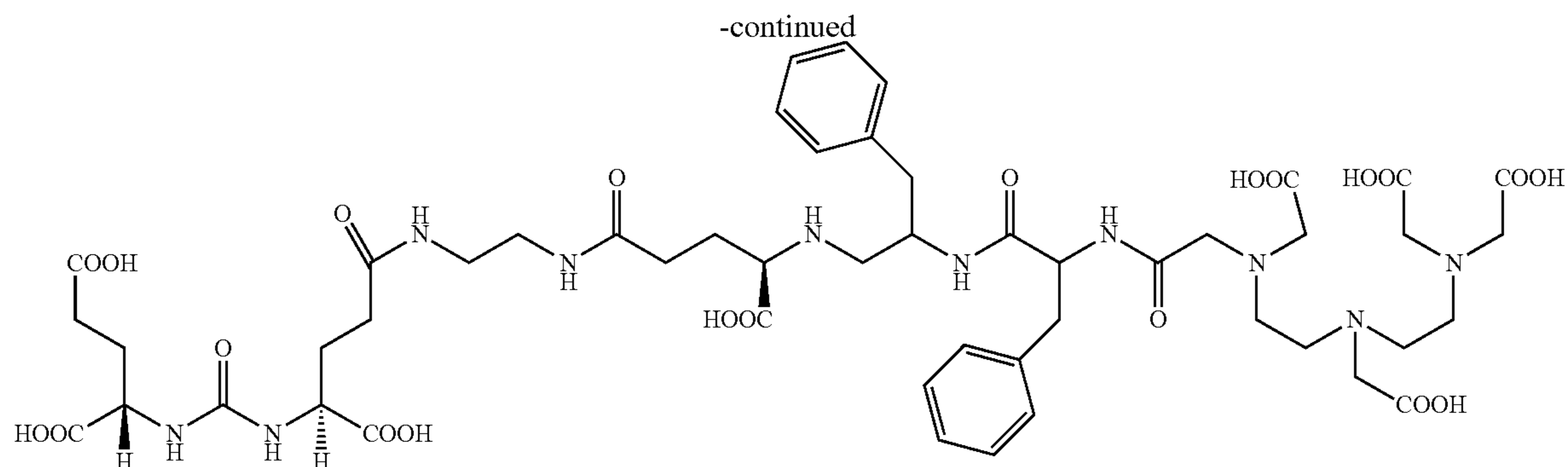
DTPA conjugate capable of chelating for example In, Ga, Ir, Yr, and the like
