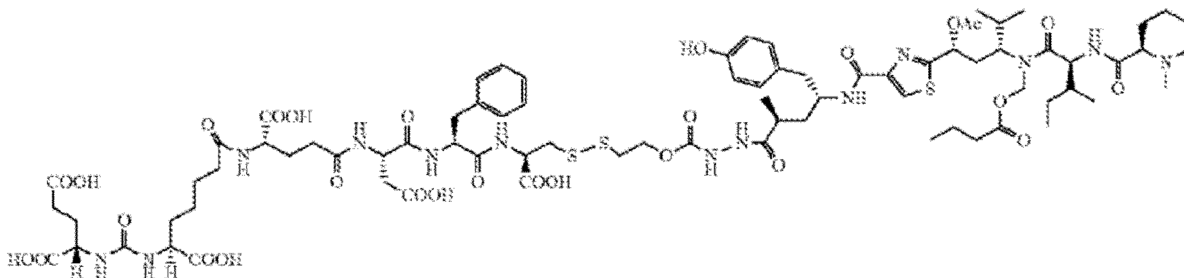
PC01SK71 C 77 H 109 N 13 O 28 S 3 Mol. Wt.: 1760.95
