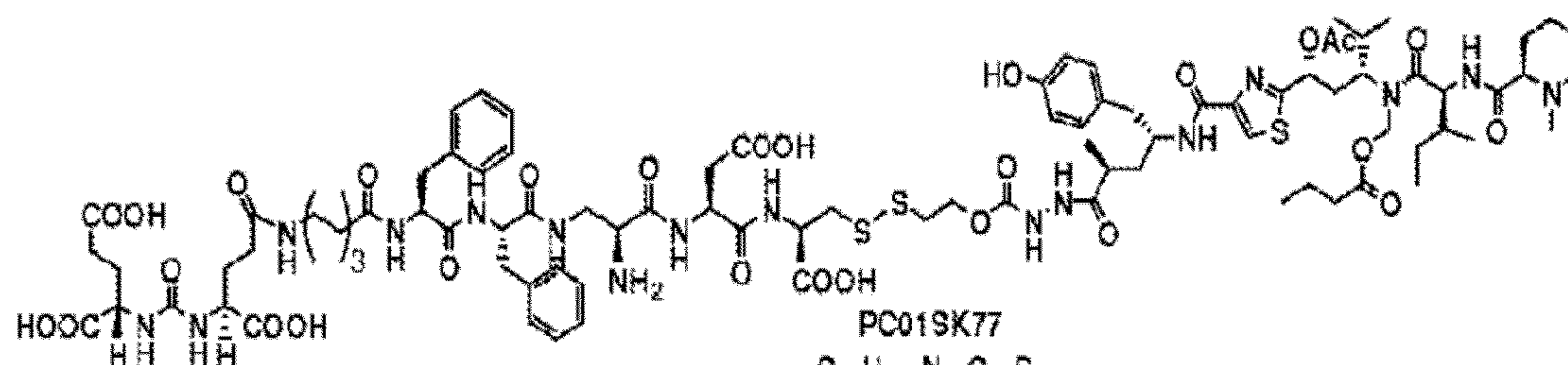
PC01SK77 C_{92}H_{133}N_{16}O_{28}S_3 Mol. Wt.: 2006.32
