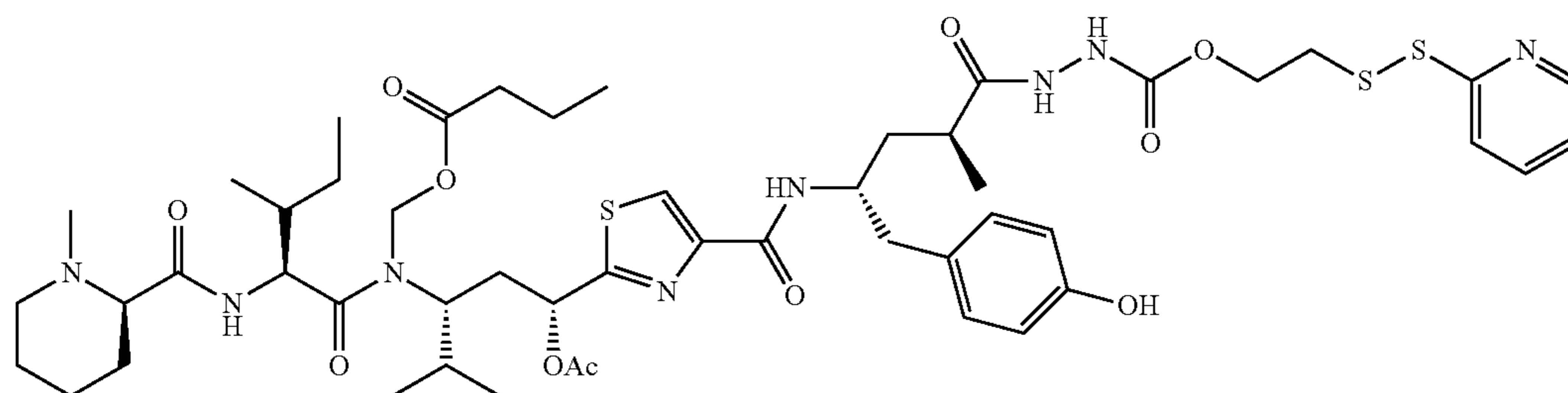
EC0312 C_{50}H_{72}N_8O_{11}S_3 Mol. Wt.: 1057.35
