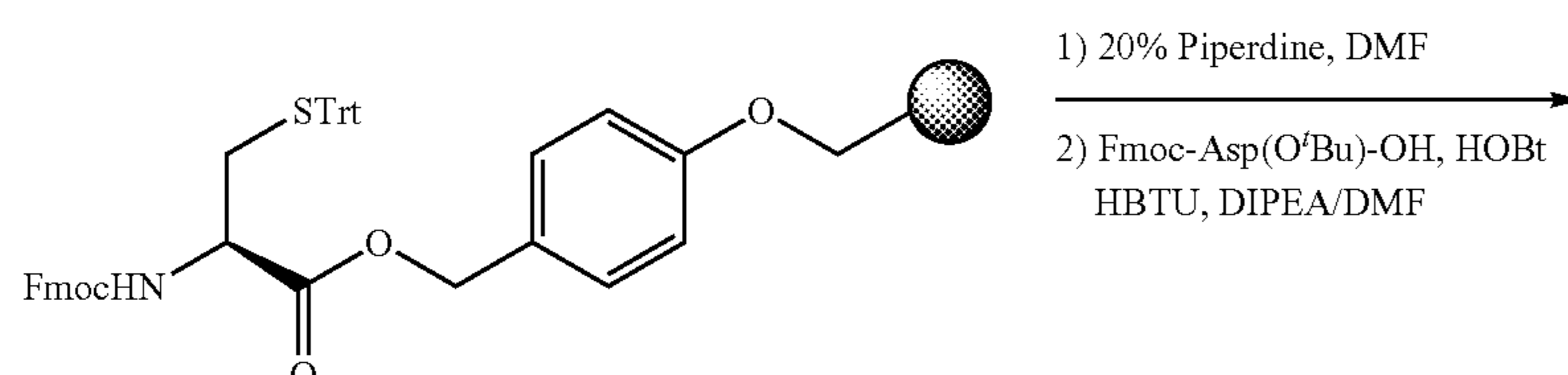
Scheme 2.3
