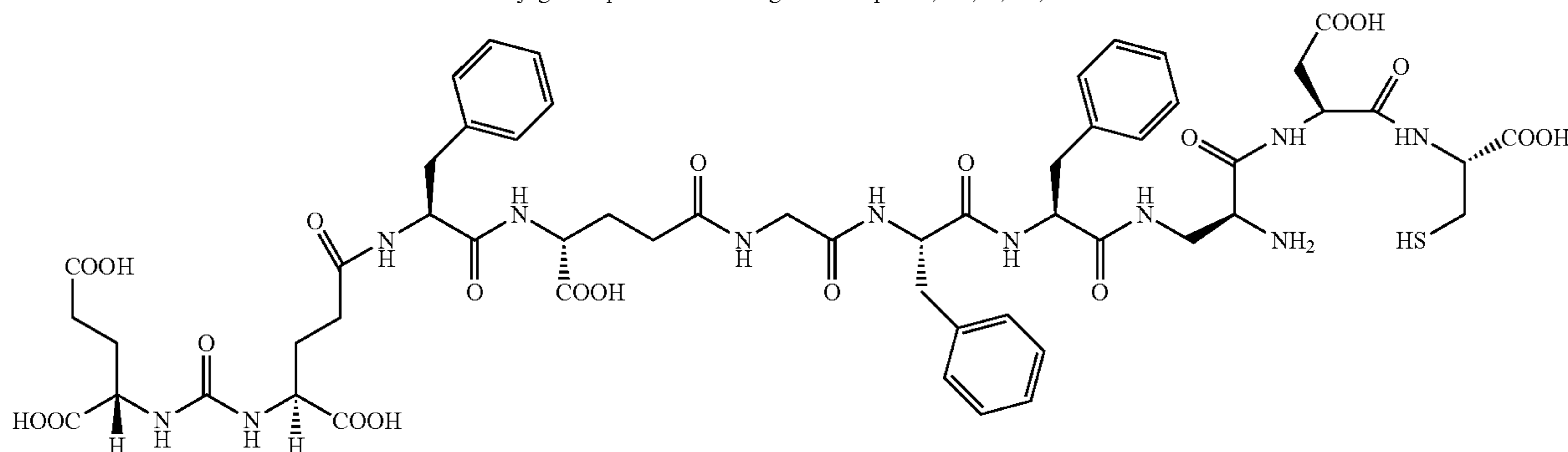
Tripeptide conjugate capable of chelating for example Tc, Tc oxides, and the like
