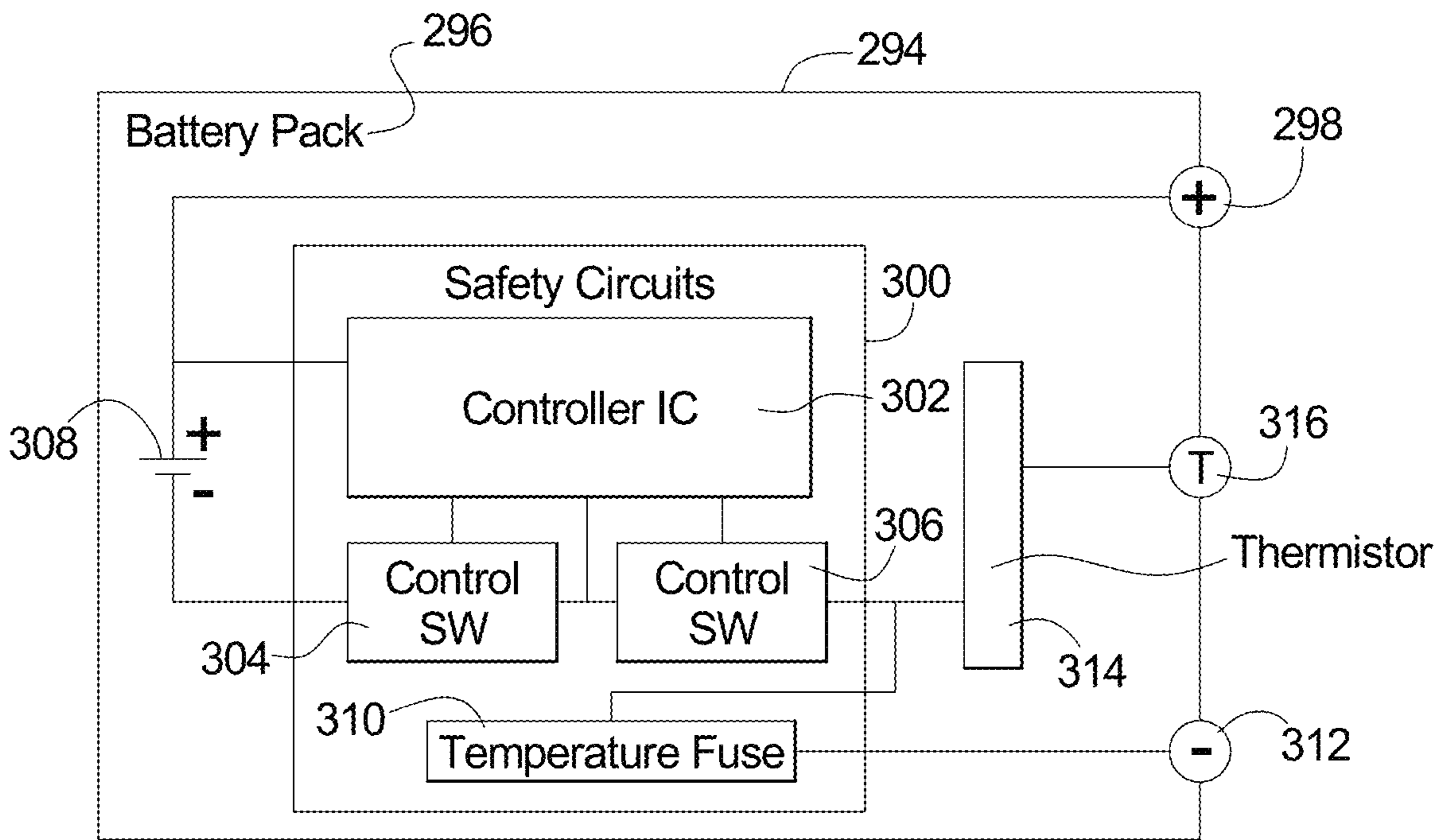
LI Battery Pack Charge System Block Diagram
