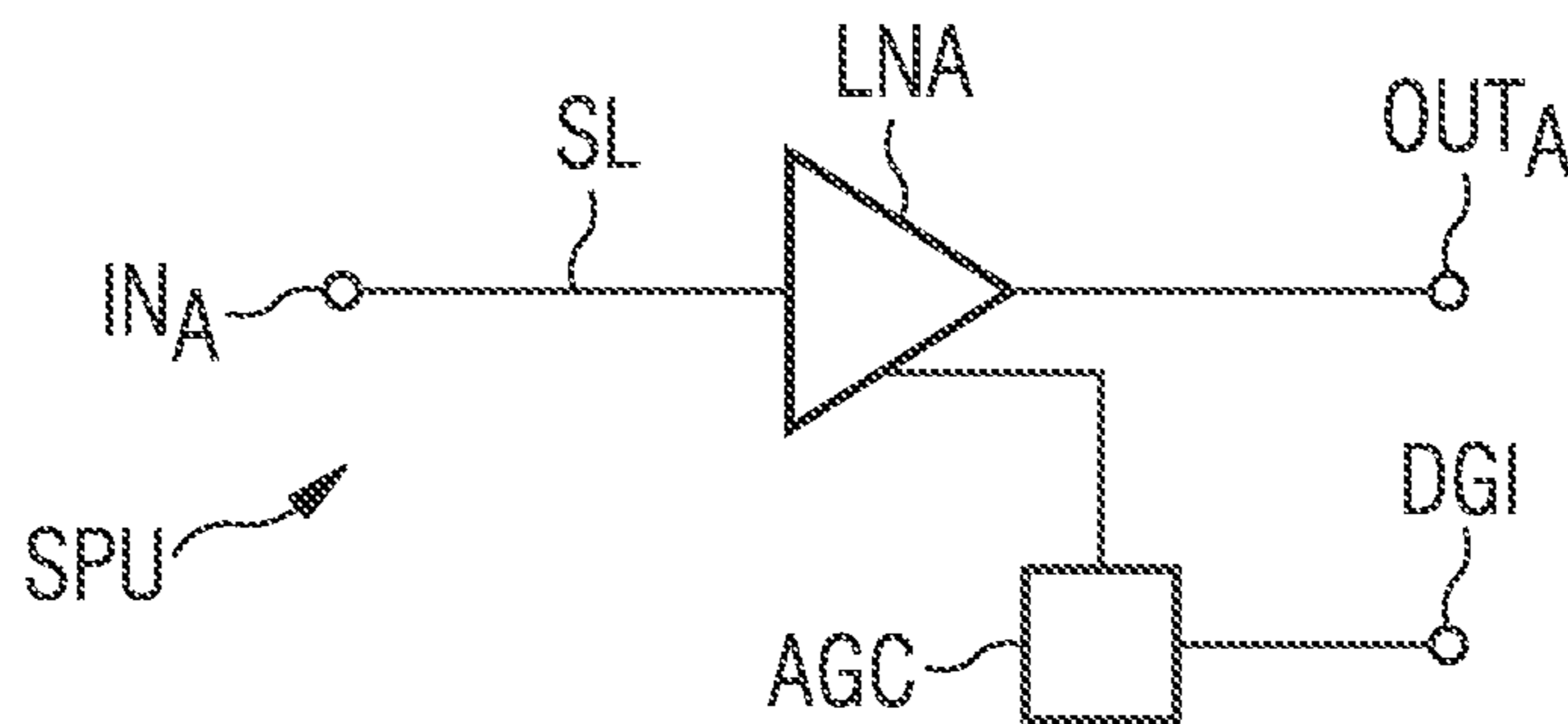
FIG 4 PRIOR ART
