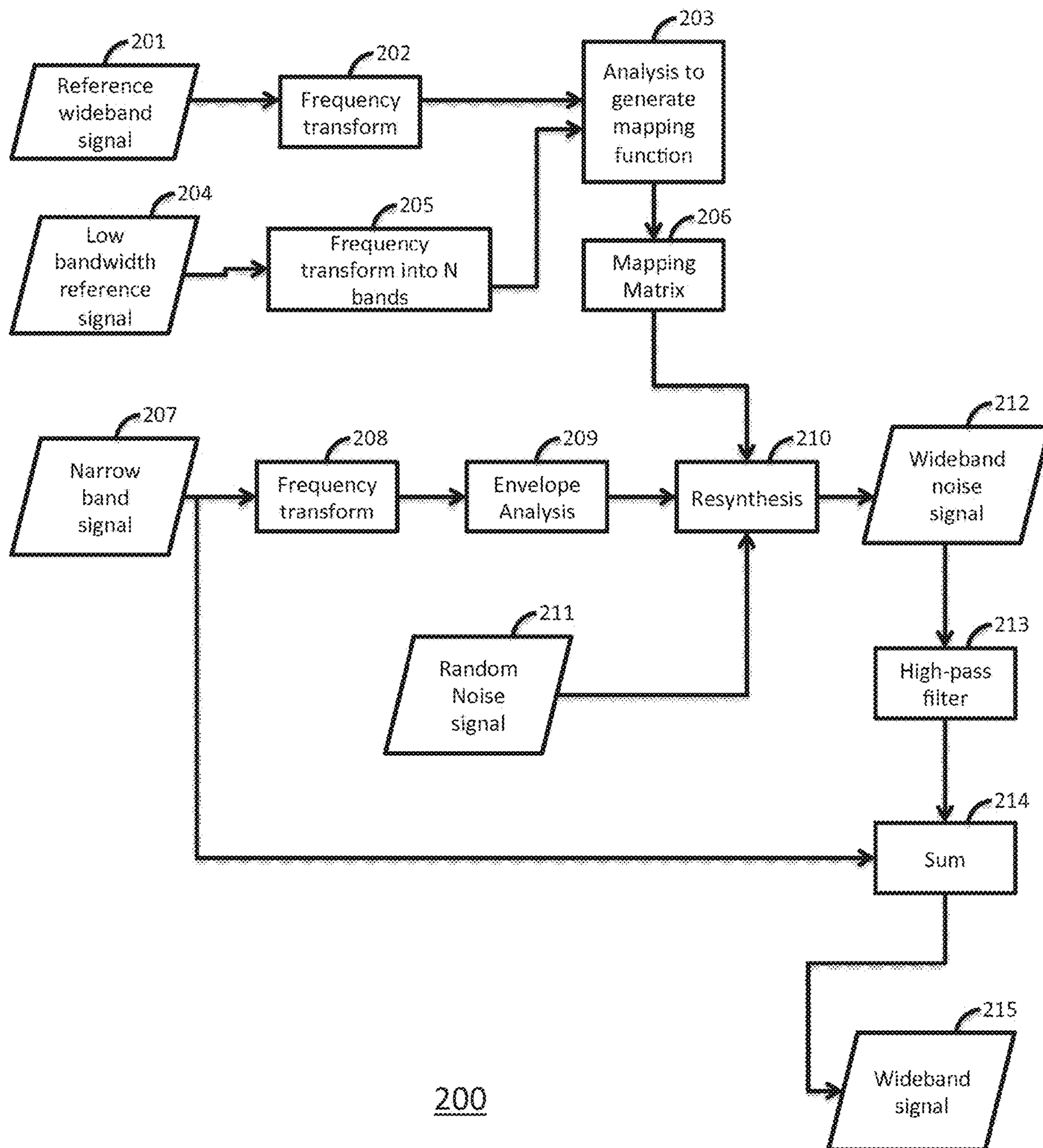
FIG. 2: Overview of Spectral Expansion System
