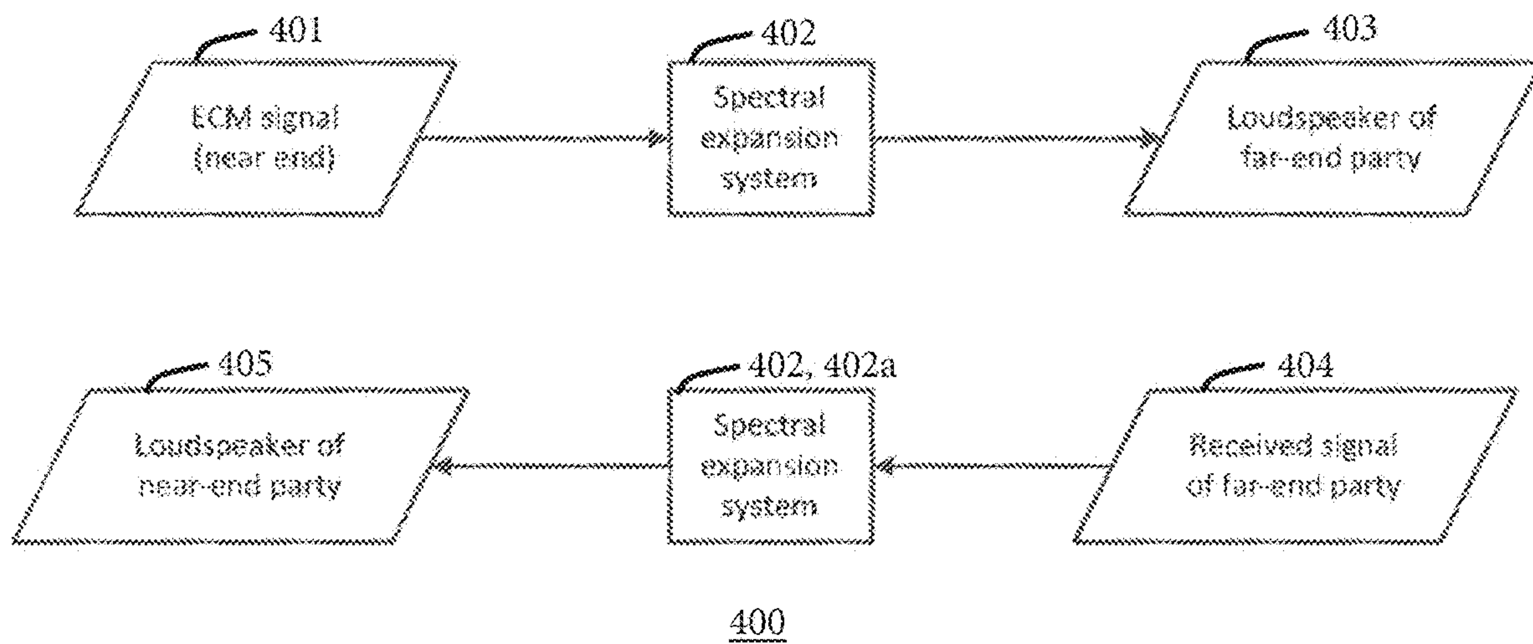
400 Figure 4: Use configurations of spectral expansion system.
