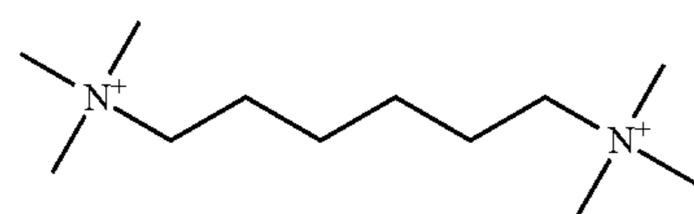
N,N,N',N',N',N'-Hexamethylhexamethylenediammonium or hexamethonium cation
