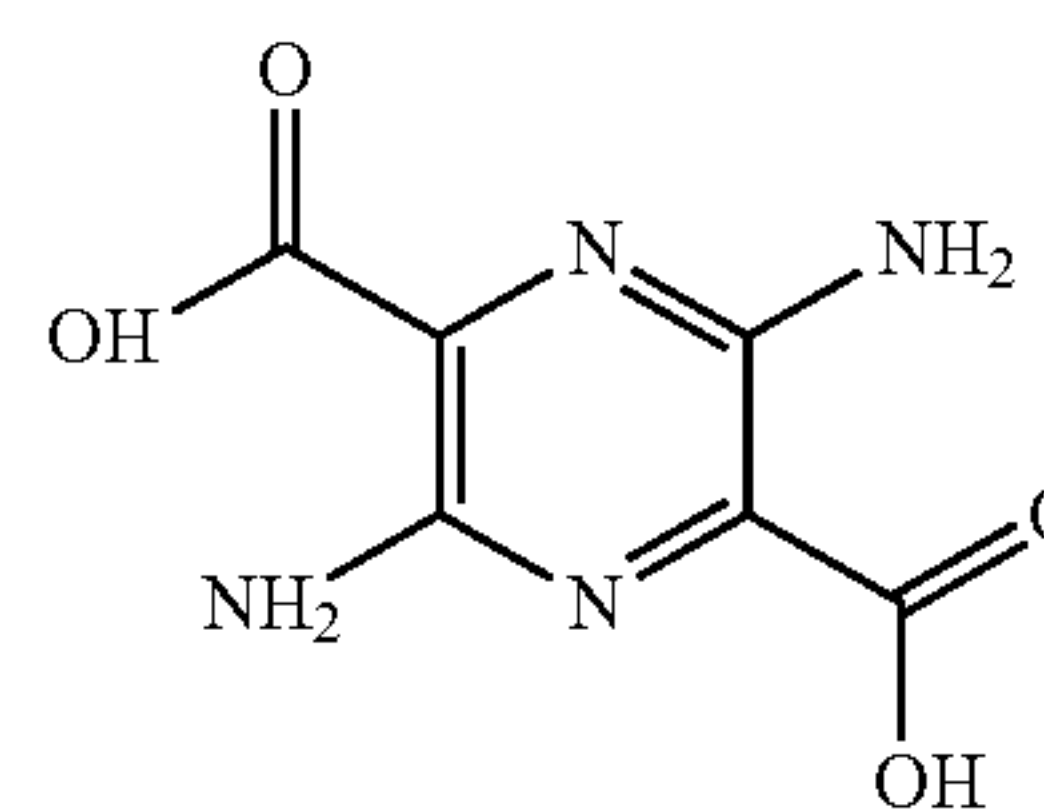
3,6-diaminopyrazine-2,5-dicarboxylic acid
