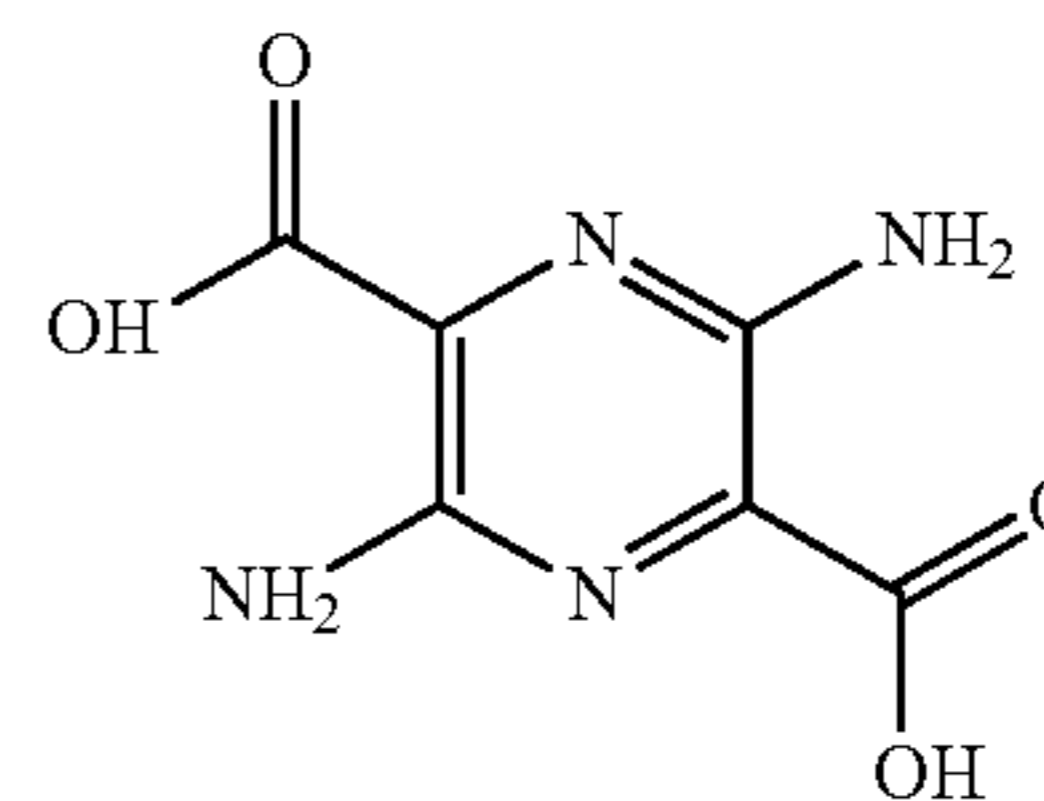
3,6-diaminopyrazine-2,5-dicarboxylic acid
