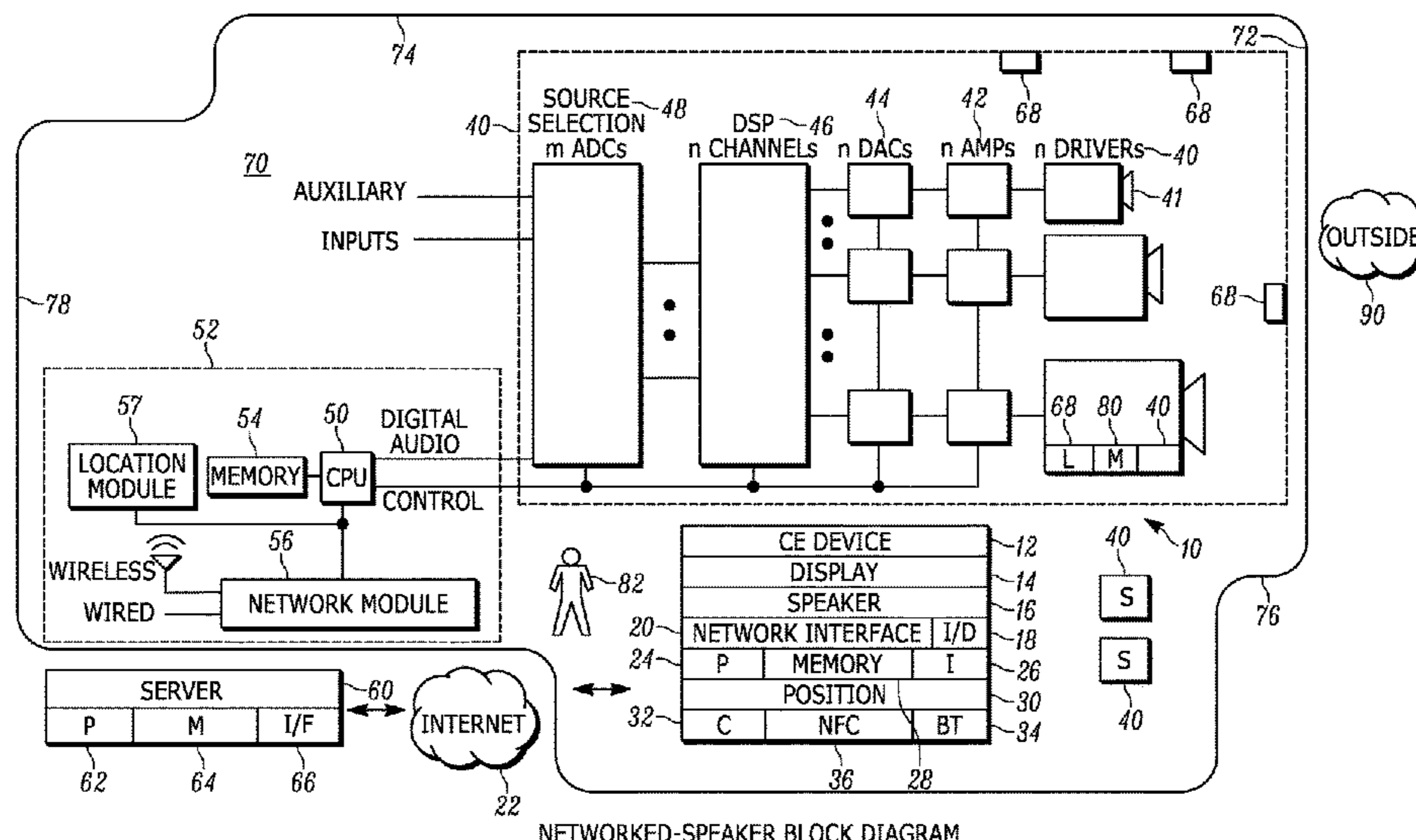
NETWORKED-SPEAKER BLOCK DIAGRAM
